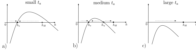
Fig. 2 The schematic graph of the function on the left hand side of (3.6) and its relationship to the stability of the value x_Y (the values x_Y is increasing with h by (3.7)) where h_H is the Holling handling ratio and thus the maximum possible value of h . When a function is positive, defending longer is optimal and vice versa. As the parameter \frac{t_a}{2} grows, one gets a) one stable root x_Y < t_h ( h_s < h_H ), b) one stable root x_Y < t_h and another stable state t_h , c) only one stable state t_h .
