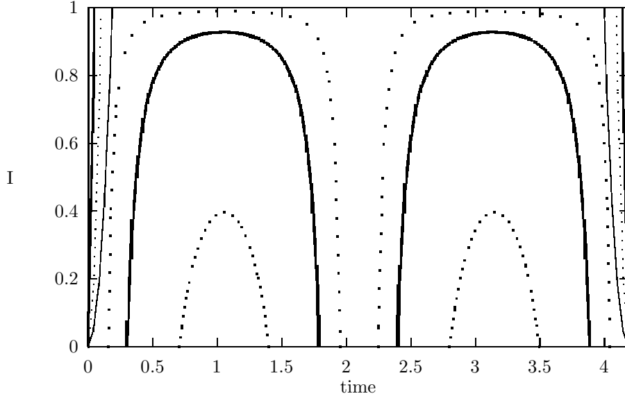
Figure 1: Upper and lower bounds for the ionization probability for the \psi_{100} -state of the hydrogen atom in the first cycle of an applied field E_z = E_0 \cos(1.5t) for E_0 = 5, 10, 20 , when neglecting the “spreading of the wave”.
