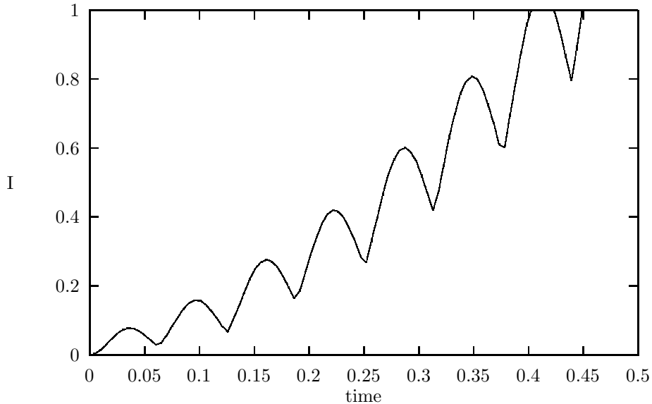
Figure 2: Upper bound for the ionization probability for the \psi_{100} -state of the hydrogen atom in the first four cycles of an applied field E_z = 10 \cos(50t) .
