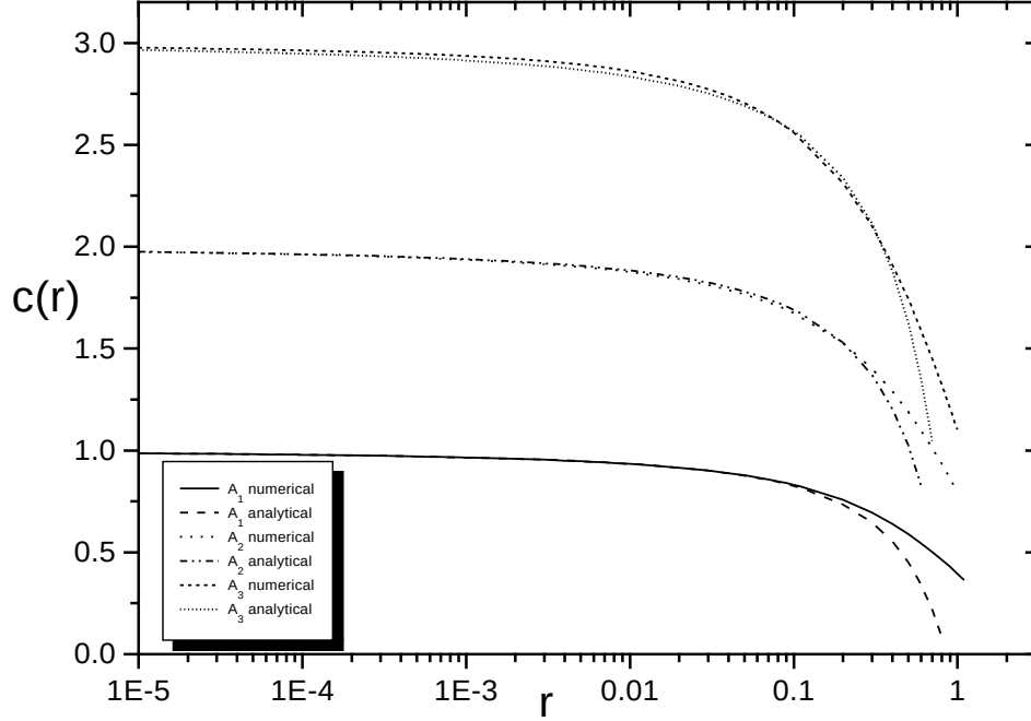
Figure 4: Numerical solution versus approximated analytical solution for the scaling function of the A_1^{(1)}, A_2^{(1)} and A_3^{(1)} -affine Toda field theory related TBA-systems with fixed effective coupling B = 0.4 .
