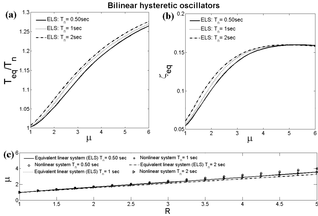
Figure 7. (a) to (b): Effective properties of ELSs corresponding to various viscously damped oscillators with bilinear hysteretic restoring force-deformation law ( \alpha = 0.5 ) compatible with the considered EC8 design spectrum. (c): Evaluation of the potential of the derived ELSs to estimate the peak response of the considered nonlinear oscillators via Monte Carlo simulations.
