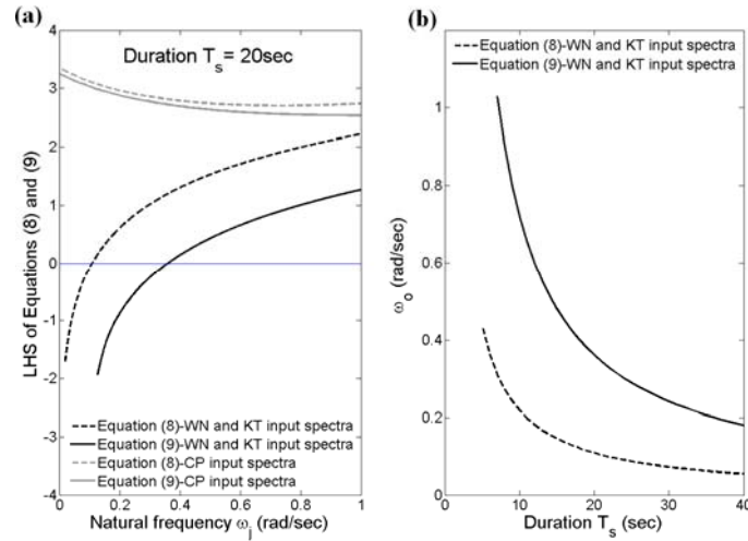
Figure 2. Numerical evaluation of the conditions posed by Equations (8) and (9) and determination of the frequency \omega_0 appearing in Equation (7) for several values of the duration T_s of the underlying stationary process characterized by the N(\omega) spectrum taken as WN (Equation (10)), KT (Equation (11) for \omega_g = 15 \text{ rad/sec} ; \zeta_g = 0.6 ), and CP (Equation (12) for \omega_g = 15 \text{ rad/sec} ; \zeta_g = 0.6 ; \omega_f = 3 \text{ rad/sec} ; \zeta_f = 1 ).
