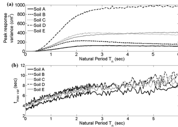
Fig. 1: Peak variances and time instants t_{\max \text{ var}} at which these peak values are attained for the response ensembles pertaining to EC8 spectrum compatible EPSs for \text{PGA} = 0.36g reported in [7] ( \zeta_n = 5\% ). Ensemble includes population: 10000.
