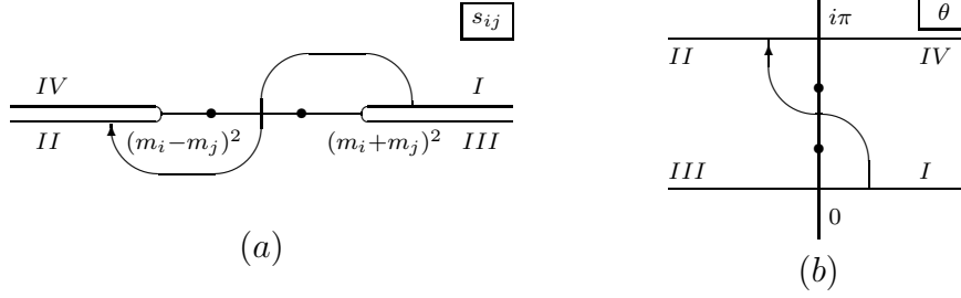
Figure 1: The analyticity domains in the complex planes of (a) the Mandelstam variable s_{ij} = (p_i + p_j)^2 and (b) the rapidity difference variable \theta = |\theta_1 - \theta_2| . The physical regimes in the s - and t -channels are denoted by I and II, respectively. The crossing transition from the s - to the t -channel is indicated by the arrow. As explained in the main text, the interchange of in and out means transition from I to III for the s -channel, and II to IV for the t -channel. The dots denote the possible positions of poles corresponding to one particle intermediate states.
