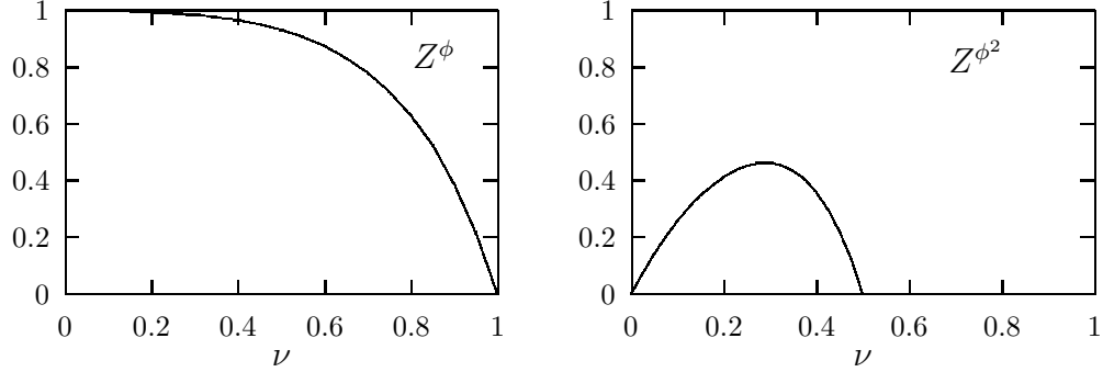
Figure 5: The wave function renormalization constants Z^\phi and Z^{\phi^2} as a function of the coupling \nu = \frac{\beta^2}{8\pi - \beta^2} = \frac{1}{1 + 2g/\pi} .
