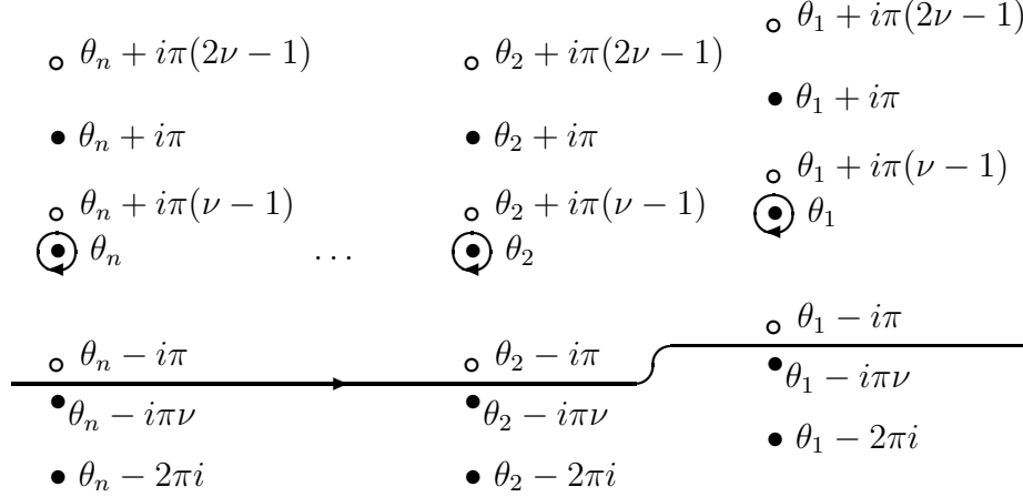
Figure 4: The integration contour \mathcal{C}_\rho (for the repulsive case \nu > 1 ). The bullets belong to poles of the integrand resulting from a(\theta_i - u_j) \phi(\theta_i - u_j) and the small open circles belong to poles originating from b(\theta_i - u_j) and c(\theta_i - u_j) .
