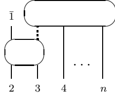
Figure 7: A graph contributing to a pole of a form factor. The dashed lines denotes an off-shell line with the propagator \frac{i}{(p_2+p_3-p_1)^2-m^2} .
