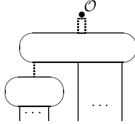
Figure 2: A singular contribution to the n -particle form factor diagram corresponding to a sub-channel. The dashed lines belong to off-shell lines.
