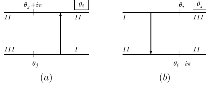
Figure 3: The physical regimes in the complex planes of the rapidity variables (a) \theta_i and (b) \theta_j for \theta_i > \theta_k > \theta_j ( k = 1, \dots, n ). Again the crossing transitions (see appendix B) are indicated by the arrows.
