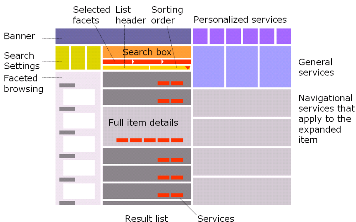
Figure 64: The general layout of the proposed INSPIRE screen
