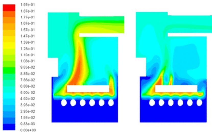
Fig. 13 Spatial distribution of the dry CO_2 mole fraction at the two reference planes.
