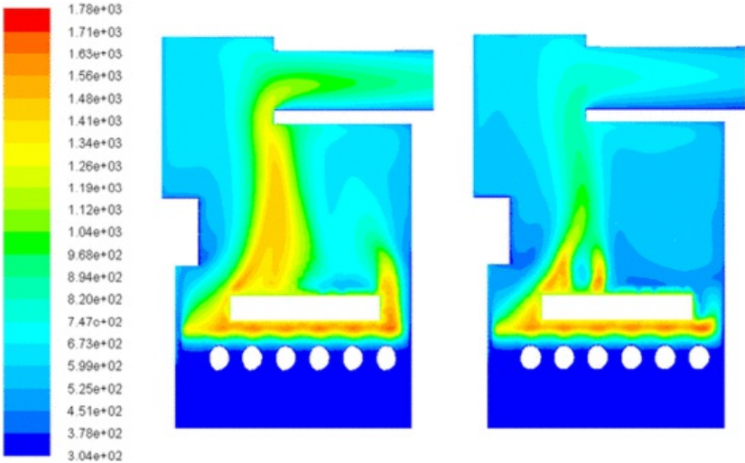
Fig. 9 Contours of spatial temperature (K) distribution at the two selected reference planes.
