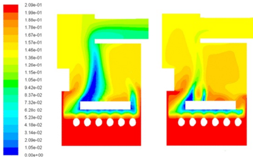
Fig. 12 Spatial distribution of the dry O_2 mole fraction at the two reference planes.
