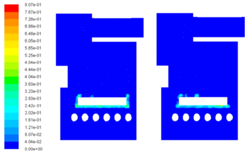
Fig. 11 Spatial distribution of the volatiles volatile volumetric mass source (kg/m³ s).
