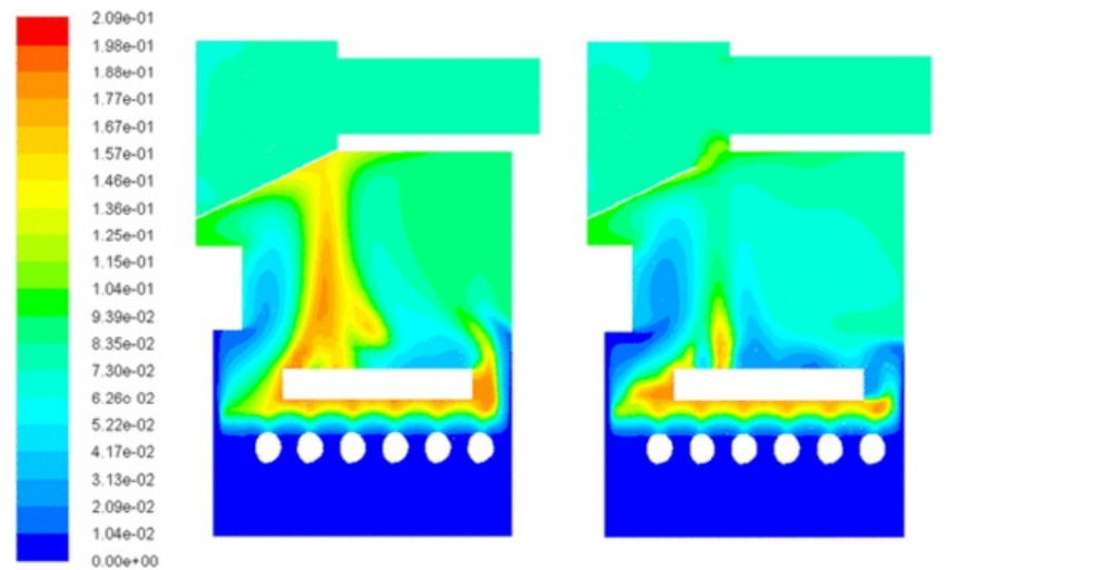
Fig. 22 Spatial distribution of the dry CO 2 mole fraction at the two reference planes: y = 0.2 (left) & y = 0.33 (right) optimized design.
