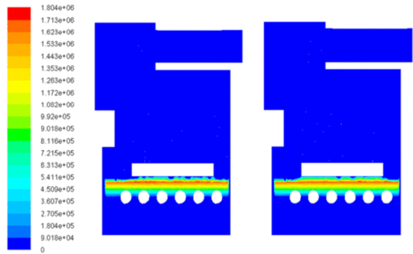
Fig. 10 Spatial distribution of the char combustion volumetric heat source (W/m³).
