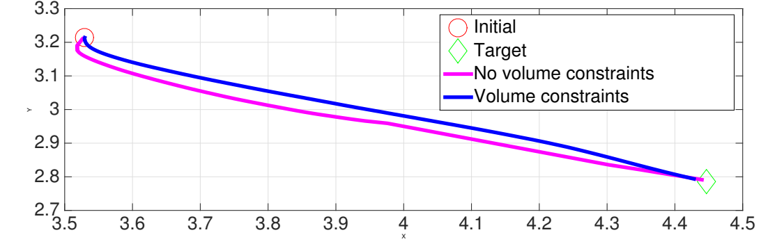
(a) Centroid trajectories together with centroids of the data.
