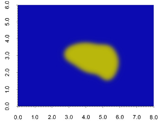
(c) Target data ( \varphi_{obs} ).
