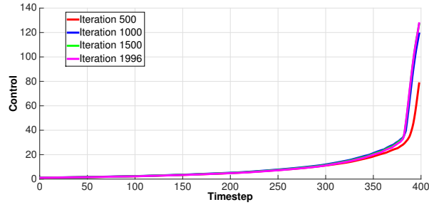
(b) Maximum value of the control for a series of iterations against time for the algorithm without volume constraints.
