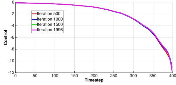
(a) Minimum value of the control for a series of iterations against time for the algorithm without volume constraints.
