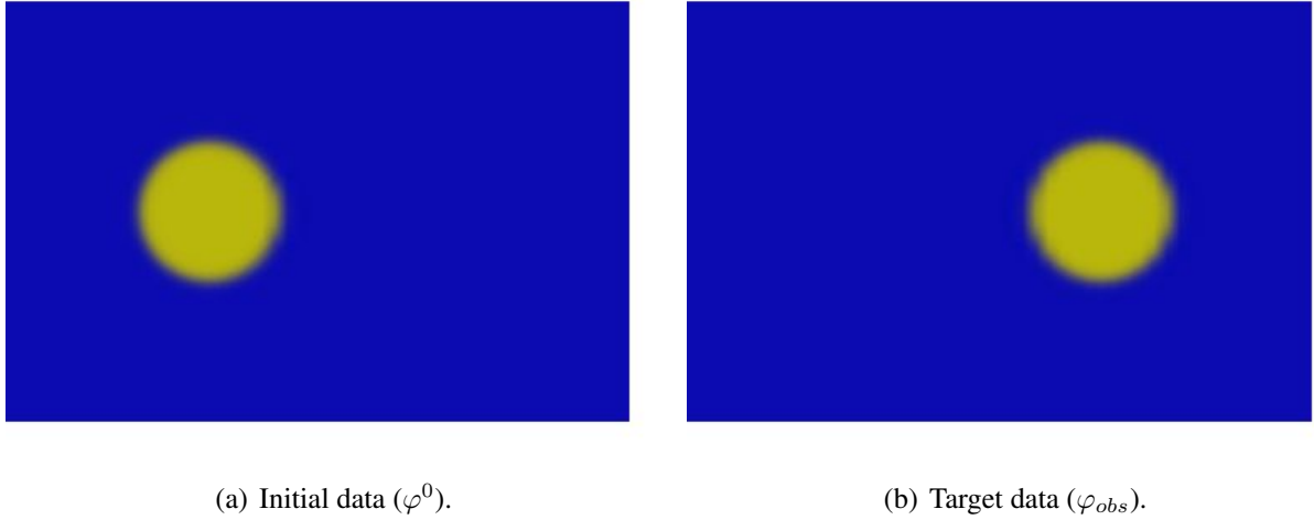
Figure 9: Initial and target data for the examples of §4.4.
