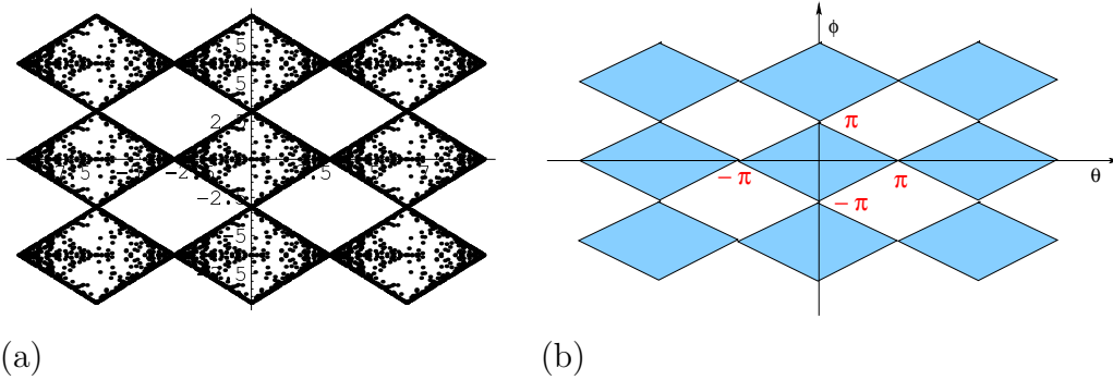
Figure 16: (a) The alga of F_0 (cf. Figure 15) draw using Monte-Carlo and redrawn in (b) to show the boundaries more clearly. We have indicated 3 \times 3 of the fundamental region to show the periodicity. Not all algæ are as regular as this.
