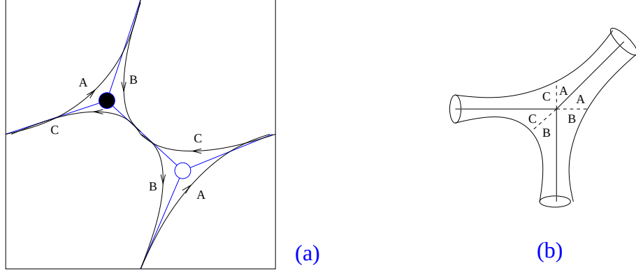
Figure 17: (a) The projection of the gluing locus for \mathbb{C}^3 onto the alga. The 3 punctures on the curve define cylinders along the (1, 1) , (0, -1) and (-1, 0) directions which project to cycles with the same winding number, labeled by A, B and C. They are shown as smooth curves, and in the limit where they glue together they meet along the locus in blue, which is the graph of the dimer model for \mathbb{C}^3 . Note that the bipartite nature of the graph follows automatically, since neighbouring vertices are surrounded by opposite orientations. This choice of (p, q) winding cycles bound polygonal regions on the torus, which are the faces of the dimer model and will later be identified with the wrapped branes. Note that each “edge” of the faces is produced by two intersecting (p, q) cycles, which will each give rise to a bifundamental chiral multiplet. (b) The dashed lines on the curve P(z, w) = 0 shows the gluing locus, i.e. the graph \Gamma .
