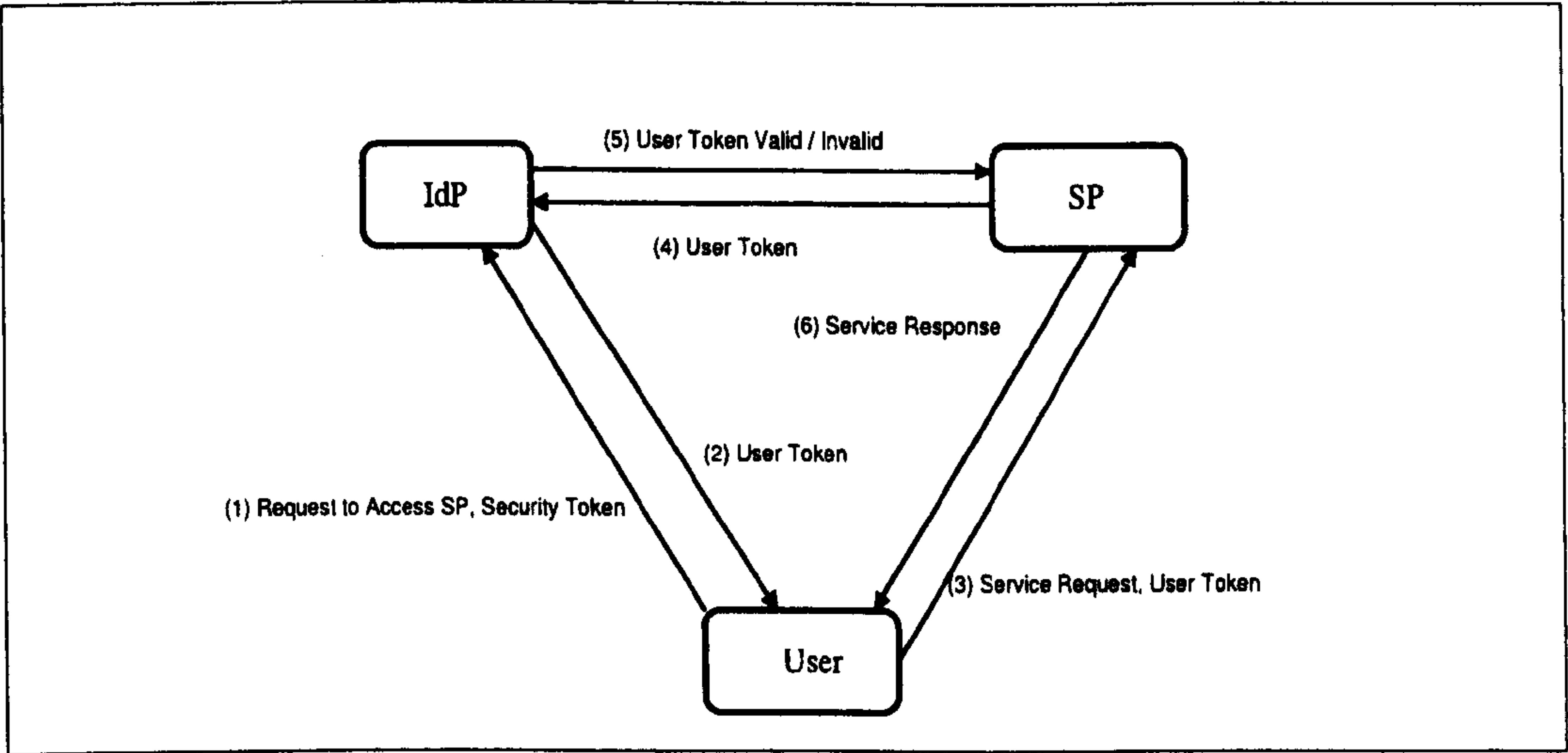
Figure 4.5: User Authentication
