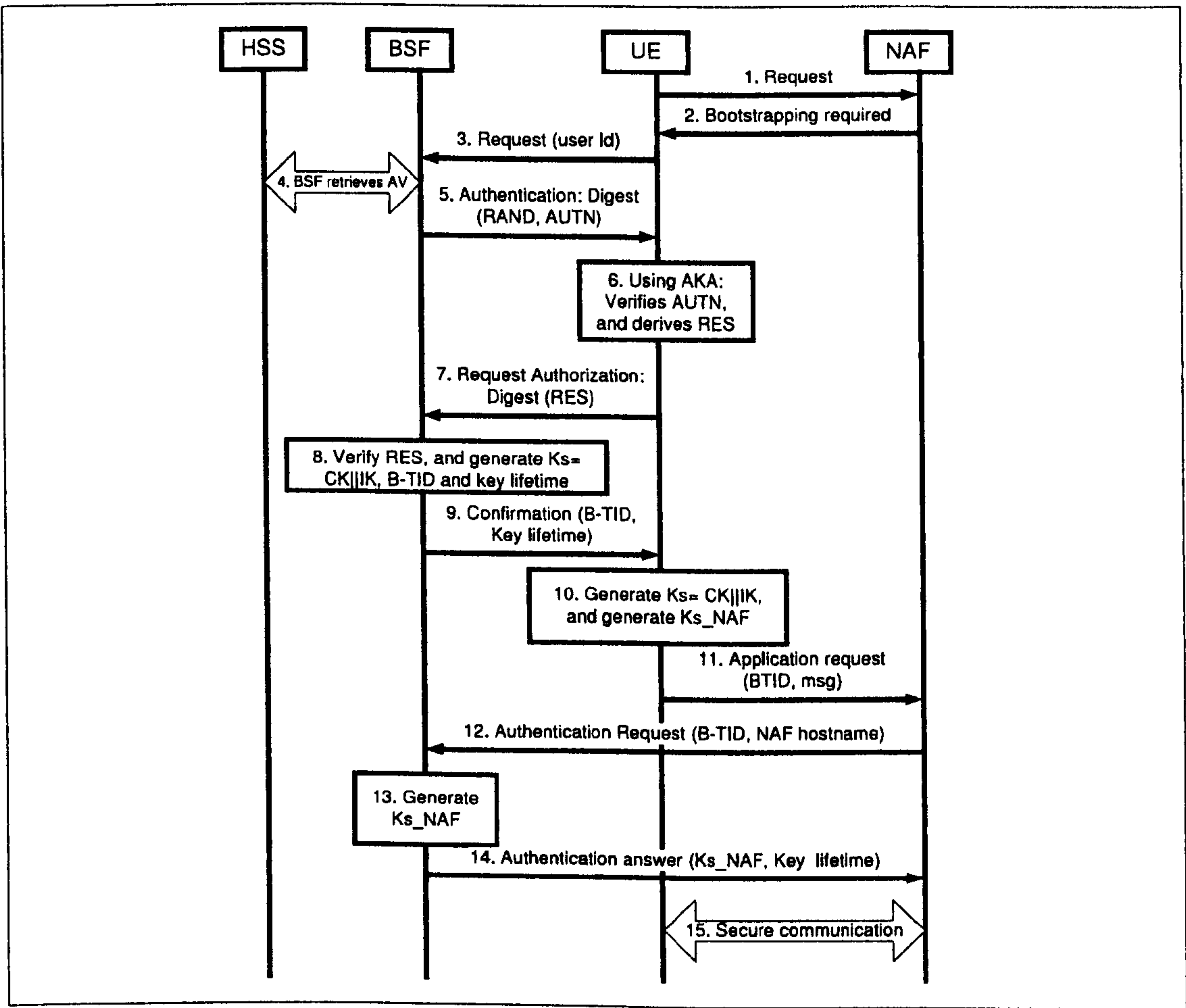
Figure 5.8: Bootstrapping procedure
