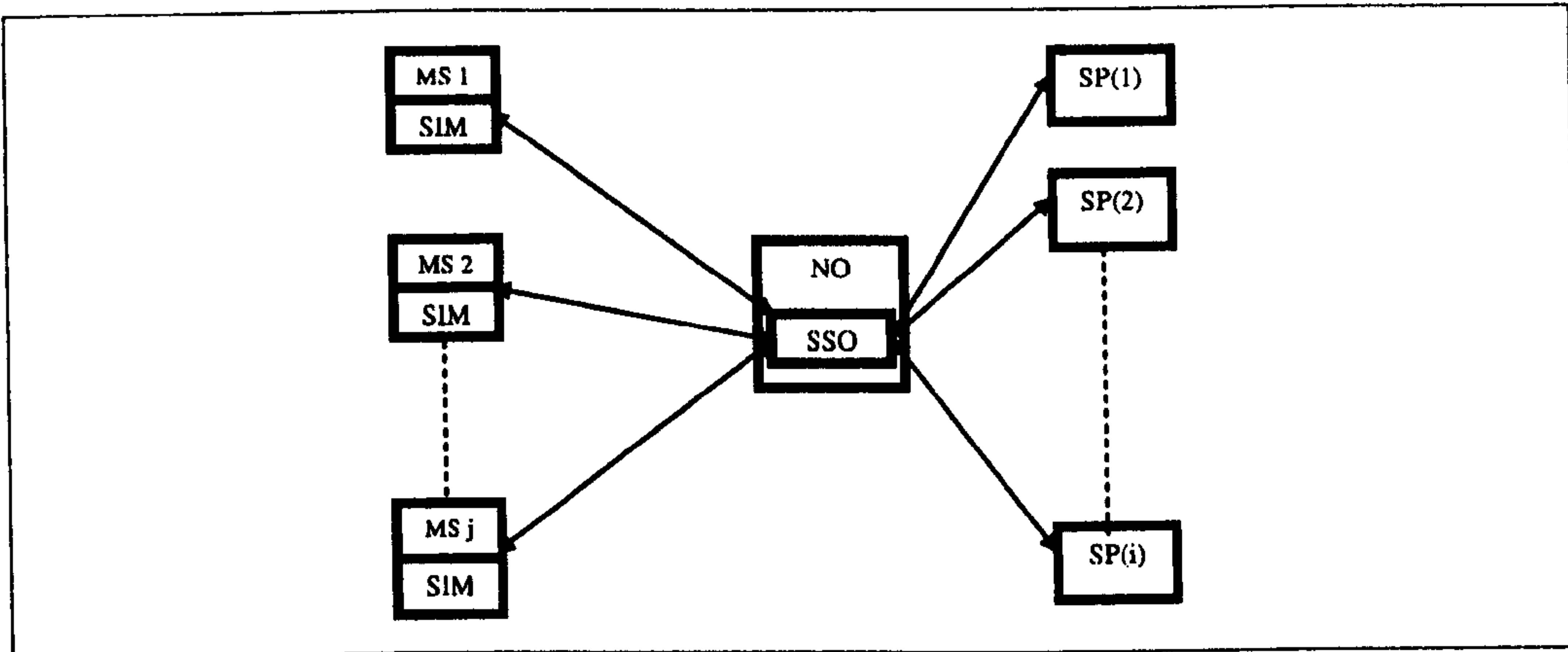
Figure 4.6: Proposed Architecture
