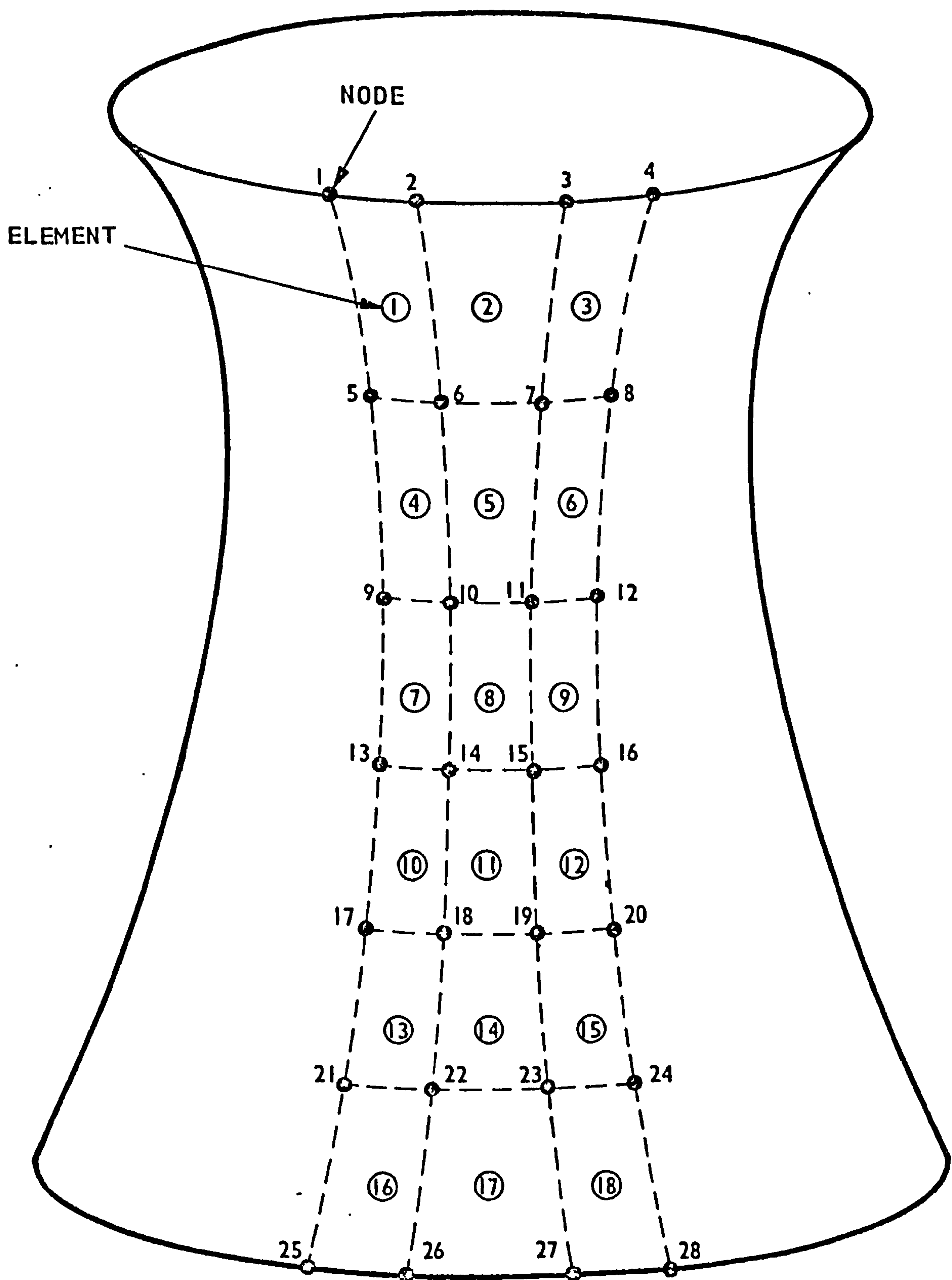
FIG. 11.29 (6x3) SHELL ELEMENT MESH FOR THE ANALYSIS OF A DOUBLY CURVED STRUCTURE WITH SYMMETRY BOUNDARY CONDITIONS (FOR THE SAKE OF CLARITY THE CIRCUMFERENTIAL DIMENSION OF THE MESH HAS BEEN EXAGGERATED)
