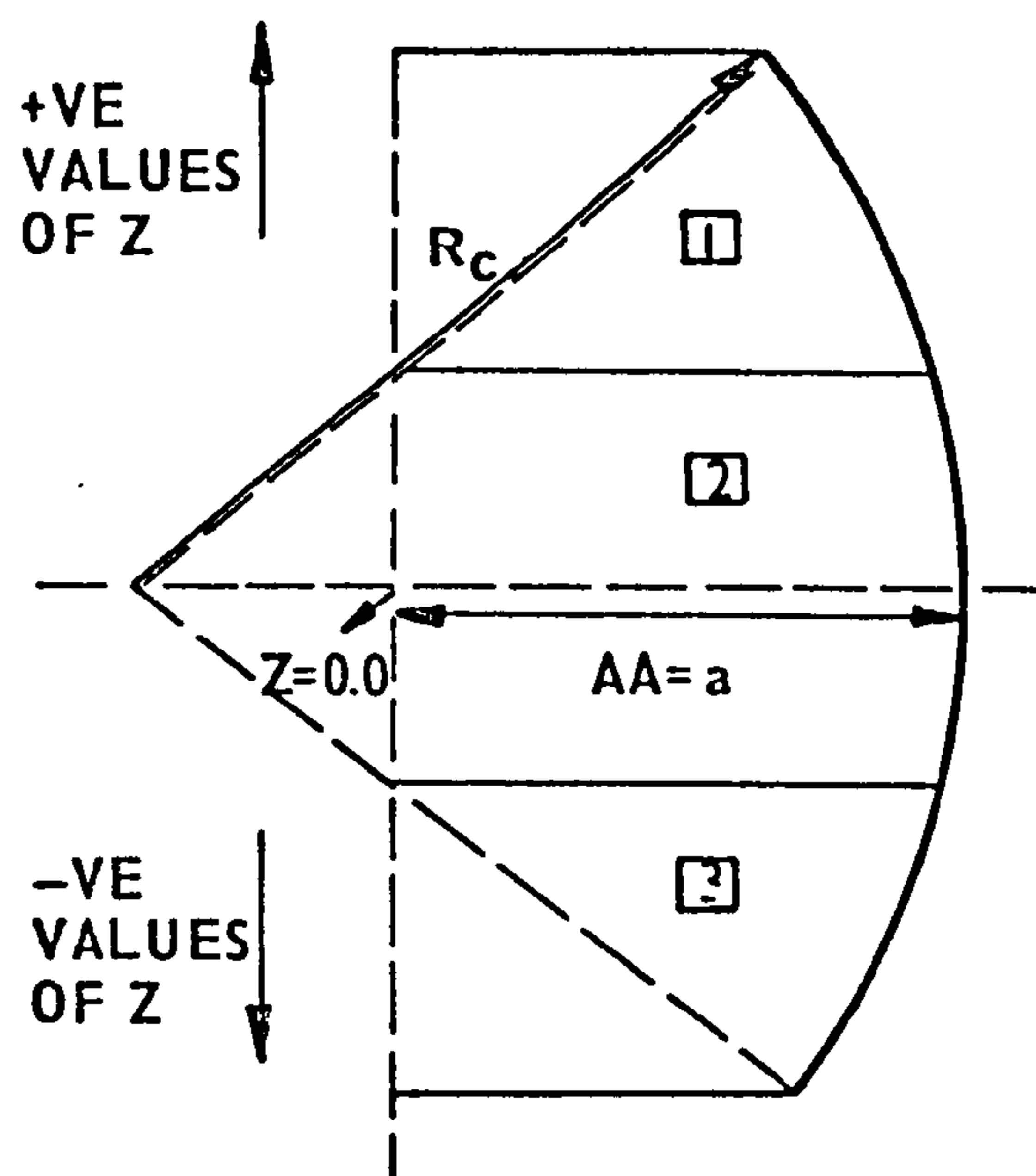
FIG7.5 REPRESENTATION OF MERIDIAN WITH CONSTANT CURVATURE. THREE SECTIONS ARE ILLUSTRATED. AA IS SHOWN IN THE FIGURE BB= |R_c| . (CARD TYPE 1H6) EQUATION : R = (a - R_c) - \sqrt{R_c^2 - Z^2} . FOR SPHERICAL SHELL a = |R_c|
