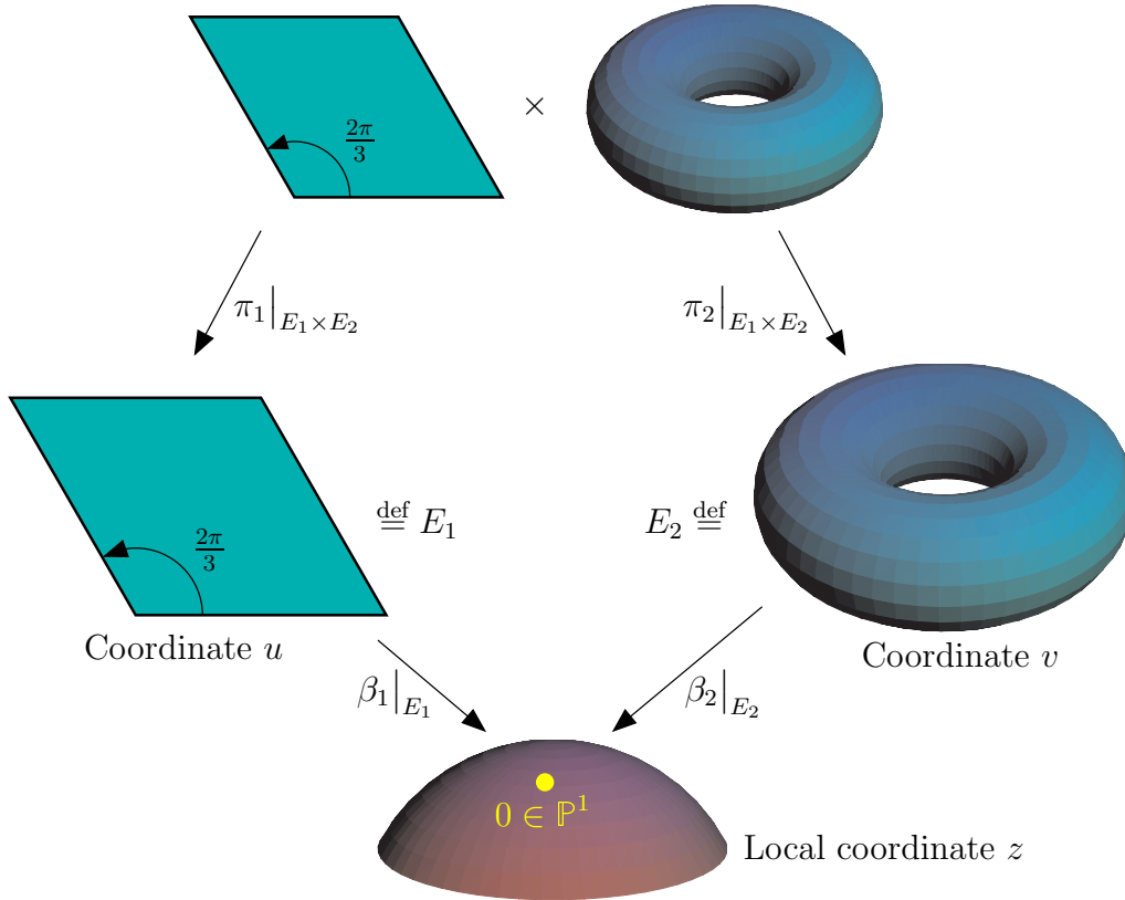
Figure 1: Fibers over 0 \in \mathbb{P}^1 .
