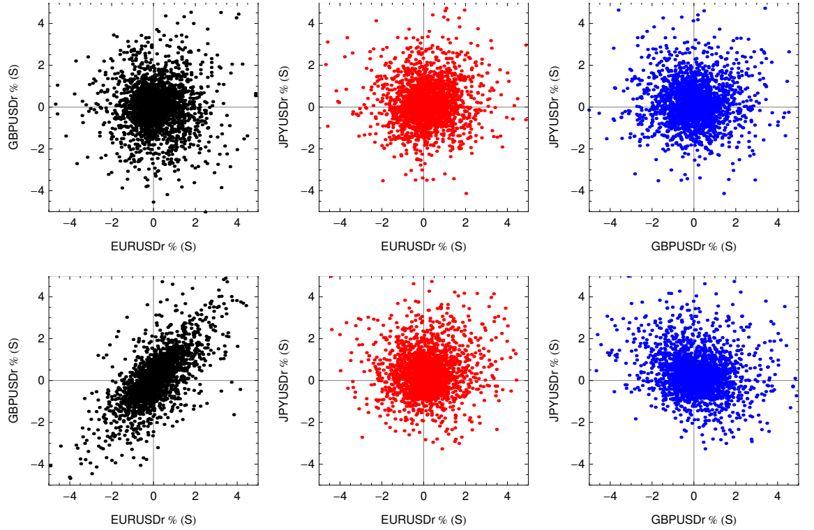
Figure 5: Bilateral scatter plots of 2540 simulated three dimensional CCVG log returns EUR/USD, GBP/USD and JPY/USD, upper panel: from the 10 parameter, non-correlated CCVG; lower panel: from the 13 parameter, correlated CCVG.
