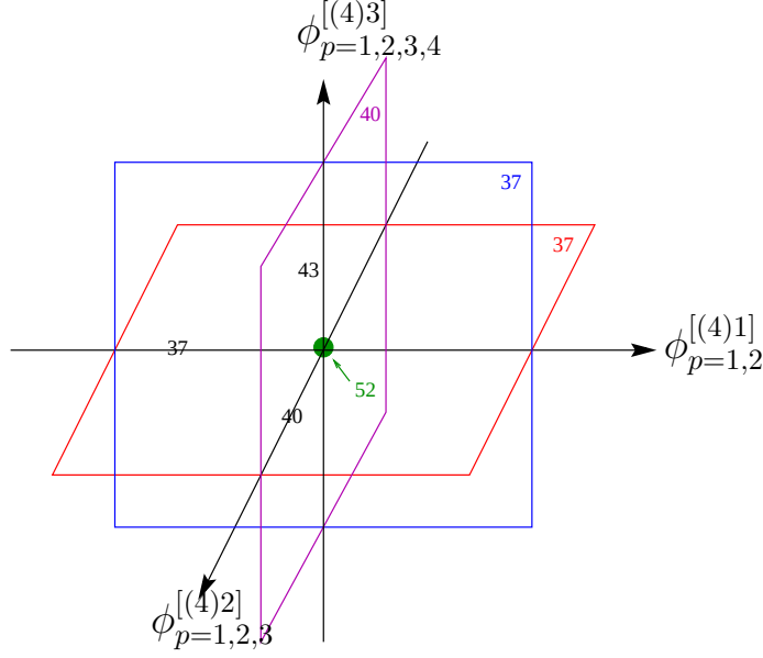
Figure 1: A subspace of the moduli space \mathcal{M} of \phi 's spanned by \phi^{[(4)1]}_{p=1,2} , \phi^{[(4)2]}_{p=1,2,3} and \phi^{[(4)3]}_{p=1,2,3,4} . Generically, in the bulk, n_{\bar{5}} = 37 , its minimal value. As we restrict to various planes and intersections thereof, we are confining ourselves to special sub-spaces of co-dimension one or higher. In these subspaces, the value of n_{\bar{5}} can increase dramatically.
