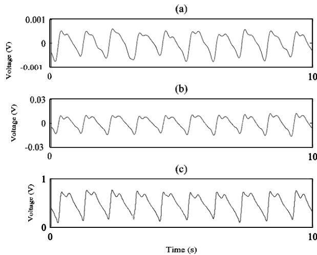
Fig.3. Infrared Photoplethysmographic traces from the forearm and fingers. (a) ZenPPG reflectance photoplethysmography from the forearm. (b) ZenPPG reflectance photoplethysmography from the finger. (c) Finger photoplethysmography from the commercial pulse oximeter.
