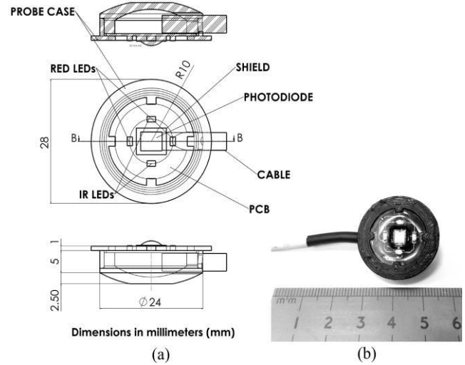
Fig.2. Reflectance forearm PPG probe. (a) Mechanical drawing, probe elements, and section. (b) Final manufactured reflectance PPG probe.
