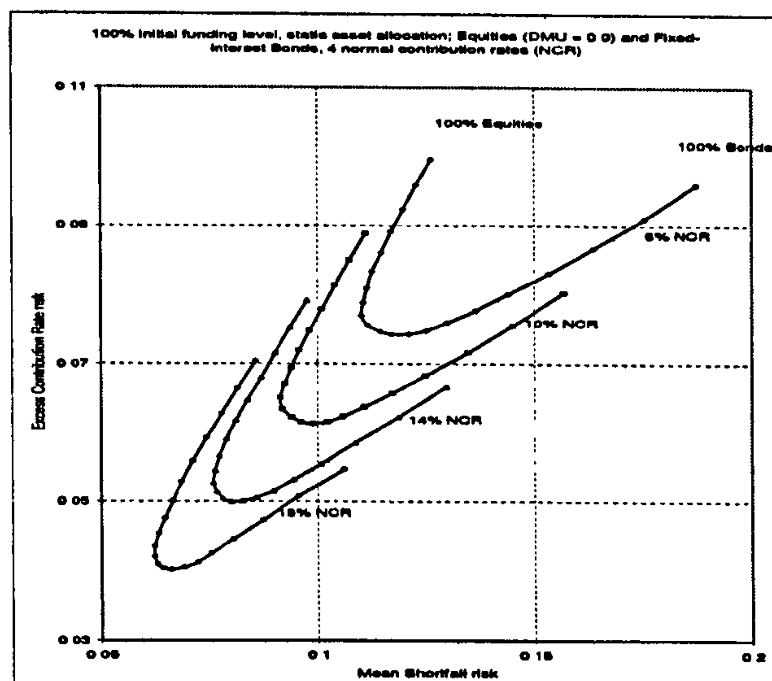
Figure 6.16: Mean Shortfall risk and Excess Contribution Rate risk trade-off at the end of 15 years for various Normal contribution rates
