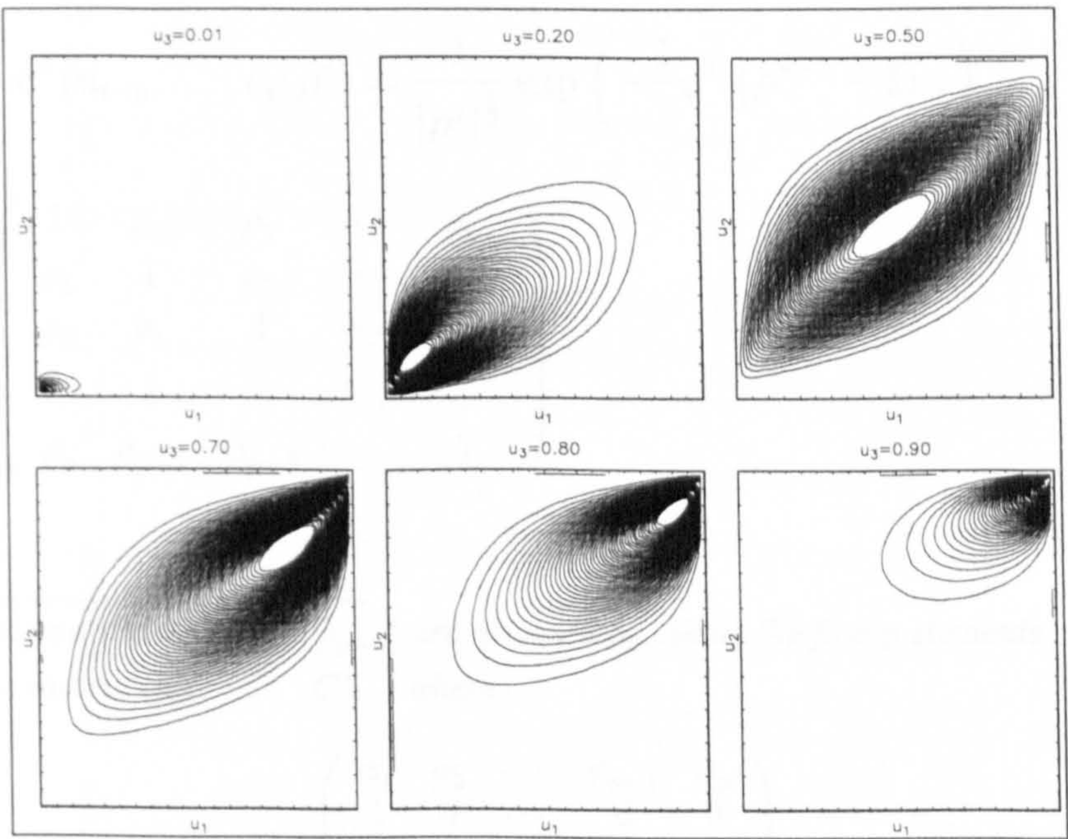
Figure 4.4: Contour slices of the 3–dimensional gaussian copula with an AR(1) correlation structure with \rho = 0.9
