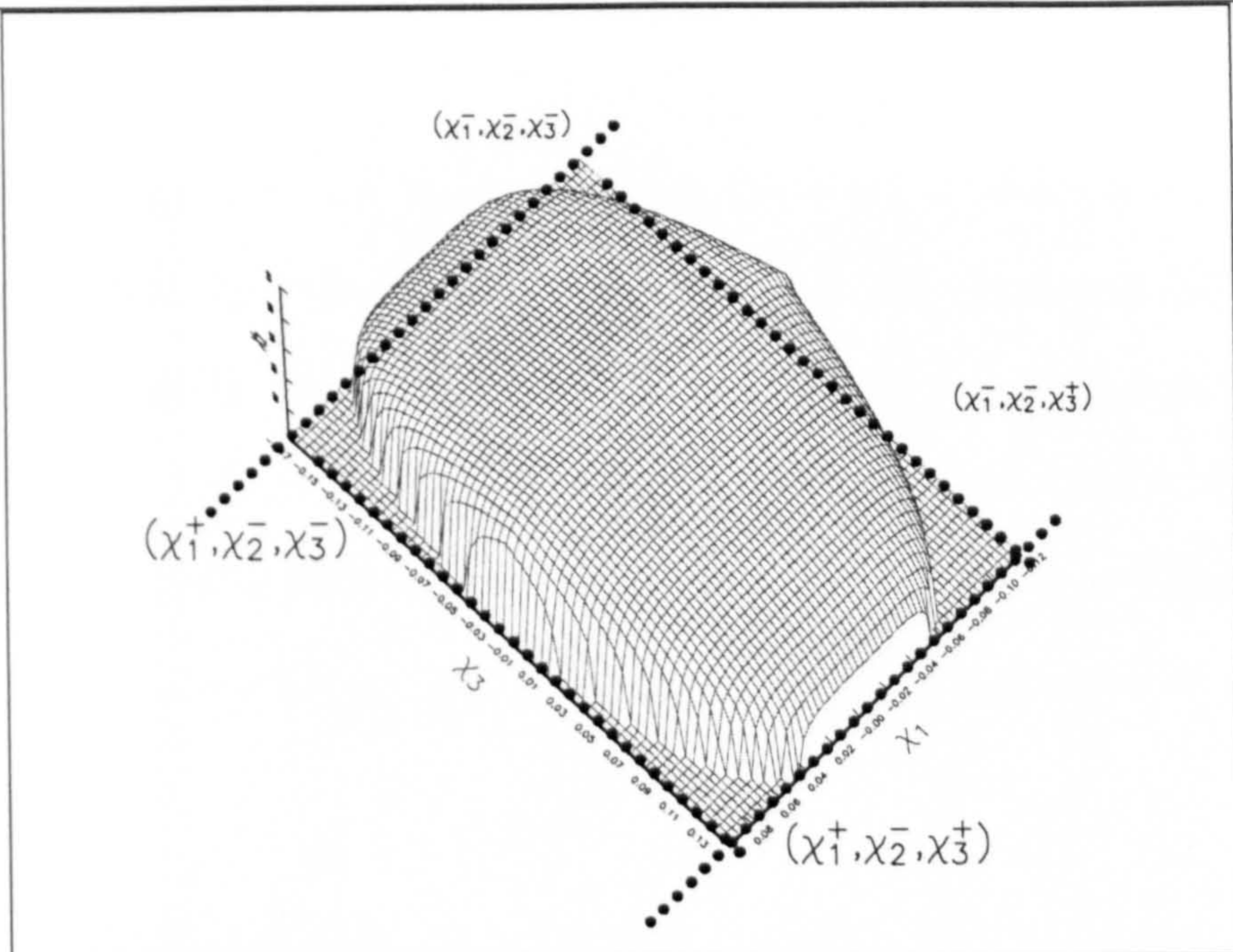
Figure 3.4: Trivariate failure areas \mathcal{A}_p^{+--}, \mathcal{A}_p^{+-}, \mathcal{A}_p^{--}, \mathcal{A}_p^{---} for MSGE ( \chi_1 ), MSUS ( \chi_2 ) and MSJP ( \chi_3 ) with a 50 years waiting period (surface). Univariate stress test scenarios are also represented (dotted line)
