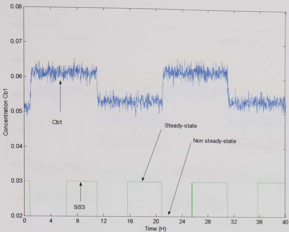
Figure (8-10): C_{b1} and SS trajectories
