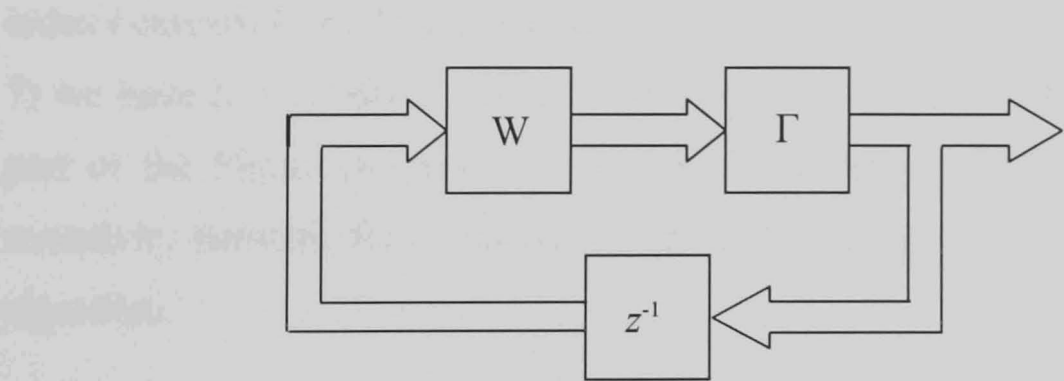
Figure 5-6: Bloc diagram representation of a typical Hopfield network.
