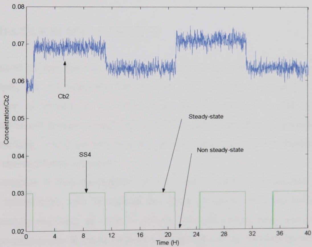
Figure (8-11): C_{b2} and SS trajectories
