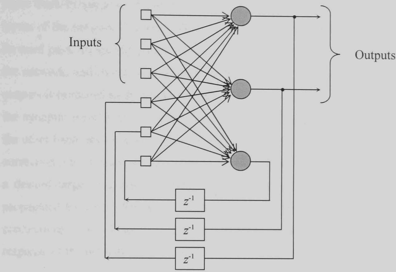
Figure 5-5: Recurrent network with hidden neurons.
