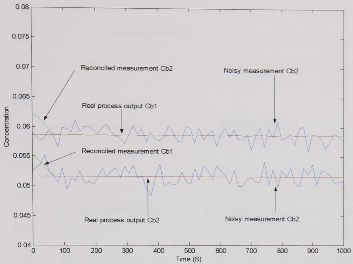
Figure (6-4): Reconciliation when measurements were subject to noise but without bias.
