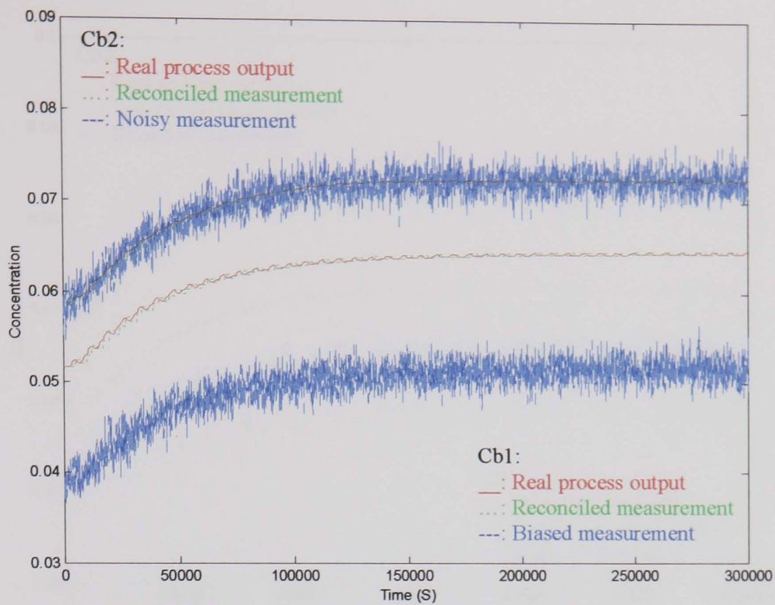
Figure (7-8): Real process output and noisy measurements trajectories, case when optimisation was applied when C_{bl} was biased with data reconciliation.
