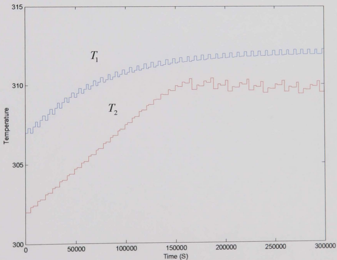
Figure (7-9): Set-points trajectories, case when optimisation was applied when C_{bl} was biased with data reconciliation.
