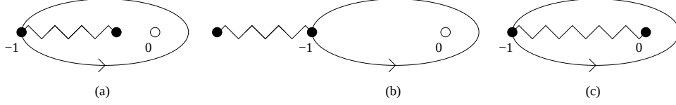
Figure 1: The contour \mathcal{C} for appendices C and D. In (a) and (b) we show the singularity structure of eq. (123), with branch points at -1 and -y'/y . In (c) we show the structure of eqs. (126) (for integer k ) and (140).
