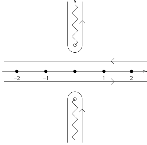
Figure 2: This figure shows the contours relevant for analyzing the various sums and integrals in appendix E. In each case, the contour is deformed from the one enclosing the real axis to the one enclosing the branch cuts on the imaginary axis. Note that the integrands in eqs. (144) and (152) have two additional poles on top of the branch cuts, while the integrand in eq. (148) has two additional poles on the real axis.
