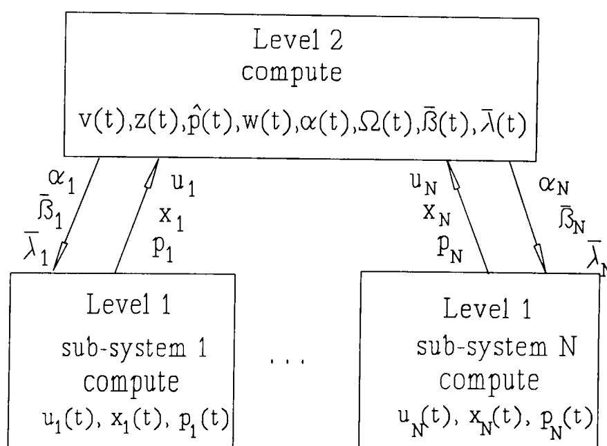
Figure 4.3.2: Information exchange in Algorithm 4.3.2
