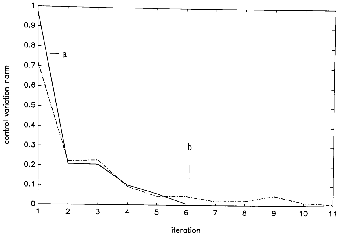
Figure 3.4.1.3: Example 3.4.1, control variation norm versus iterations
