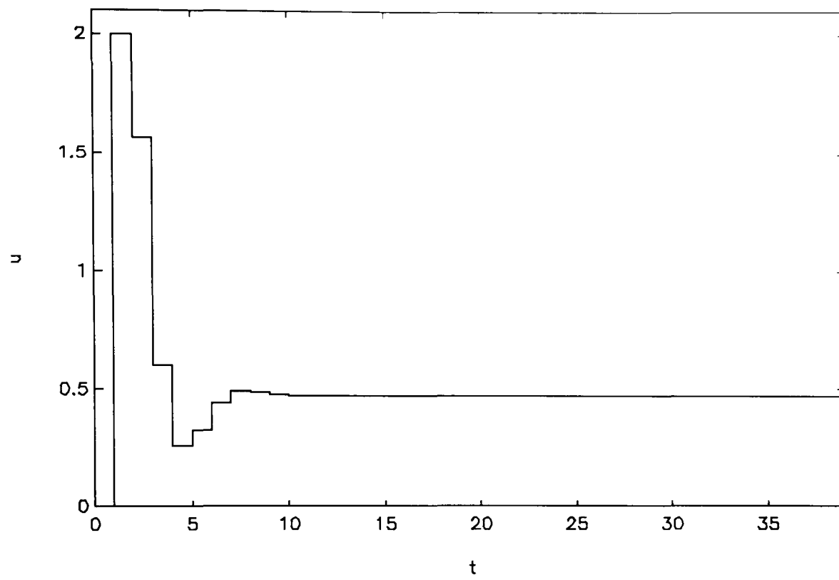
Figure 9.5.1.2: Example 9.5.1, control signal
