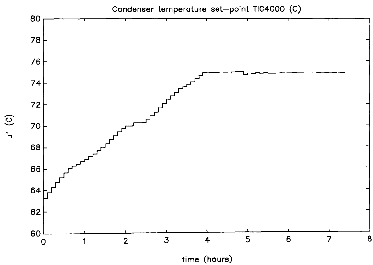
Figure 10.6.2.3: Example 10.6.2.a, condenser temperature controller set-point
