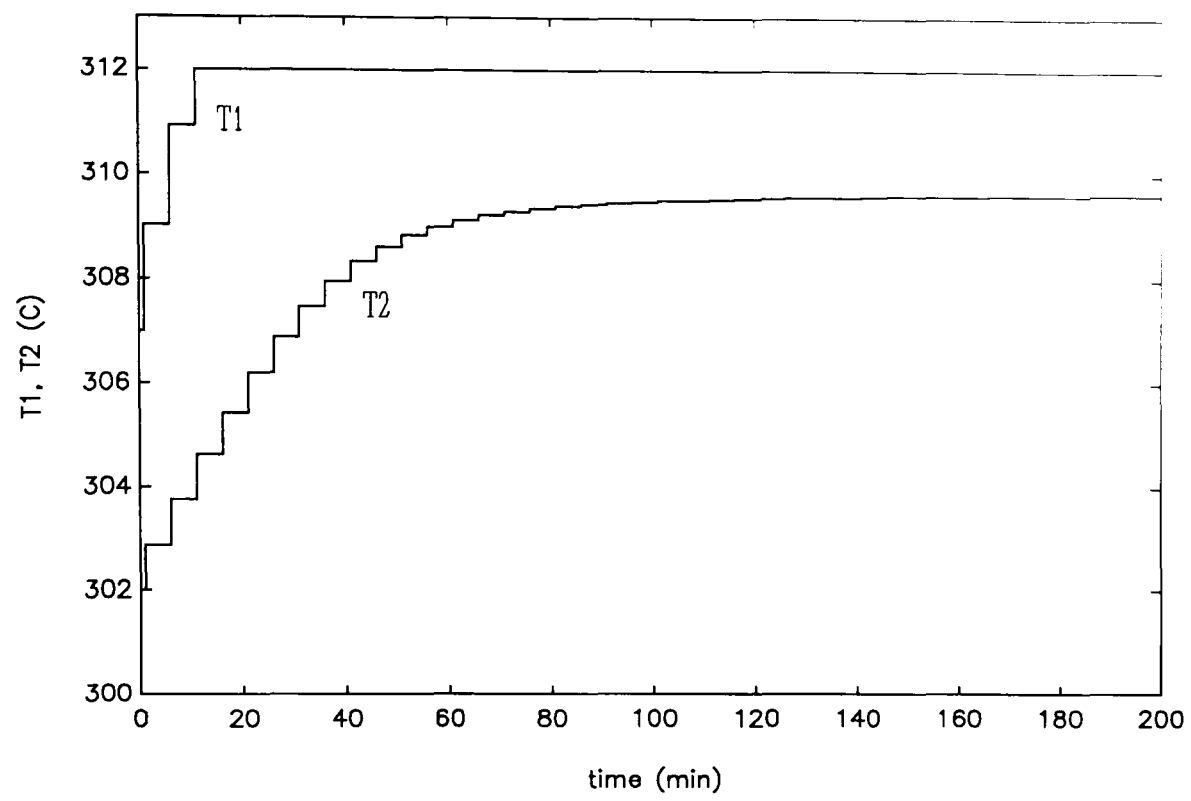
Figure 10.6.3.2: Example 10.6.3a, control signals, temperatures in reactors 1 and 2
