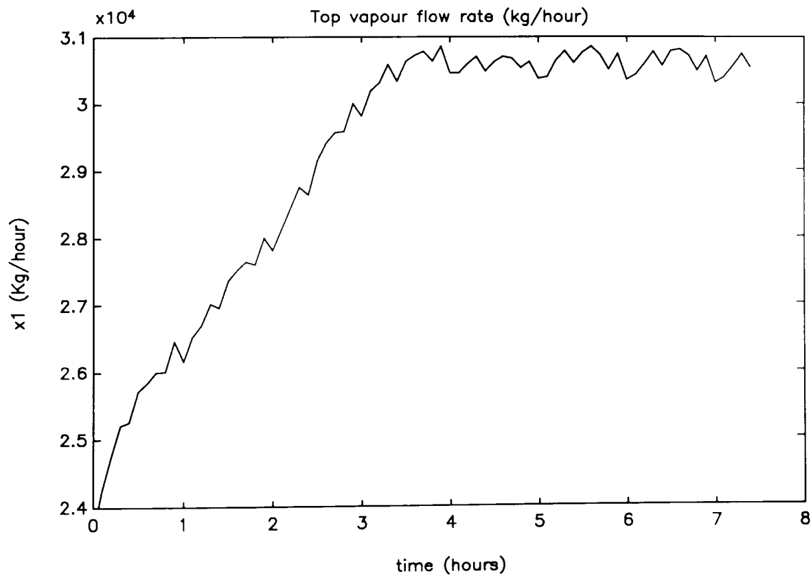
Figure 10.6.2.1: Example 10.6.2.a, Top vapour flow rate trajectory
