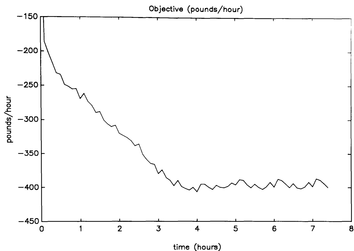
Figure 10.6.2.6: Example 10.6.2.a, evolution of the steady-state objective function
