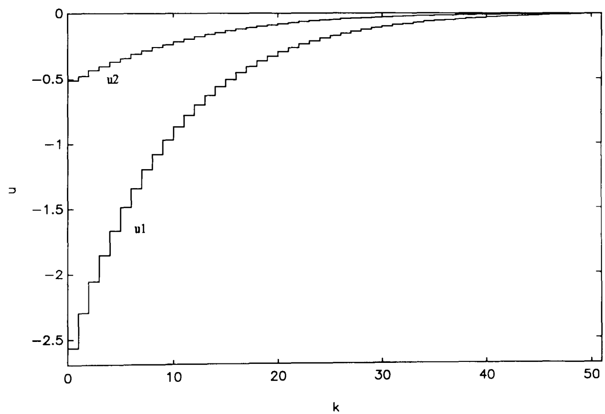
Figure 5.5.1.2: Example 5.5.1, final control vector
