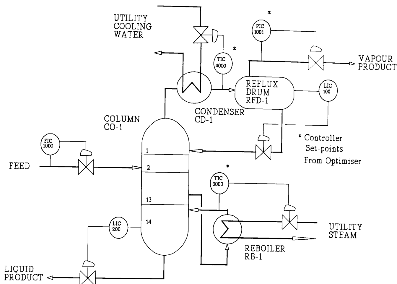
Figure 10.6.2.18: Example 10.6.2, schematic diagram of the process
