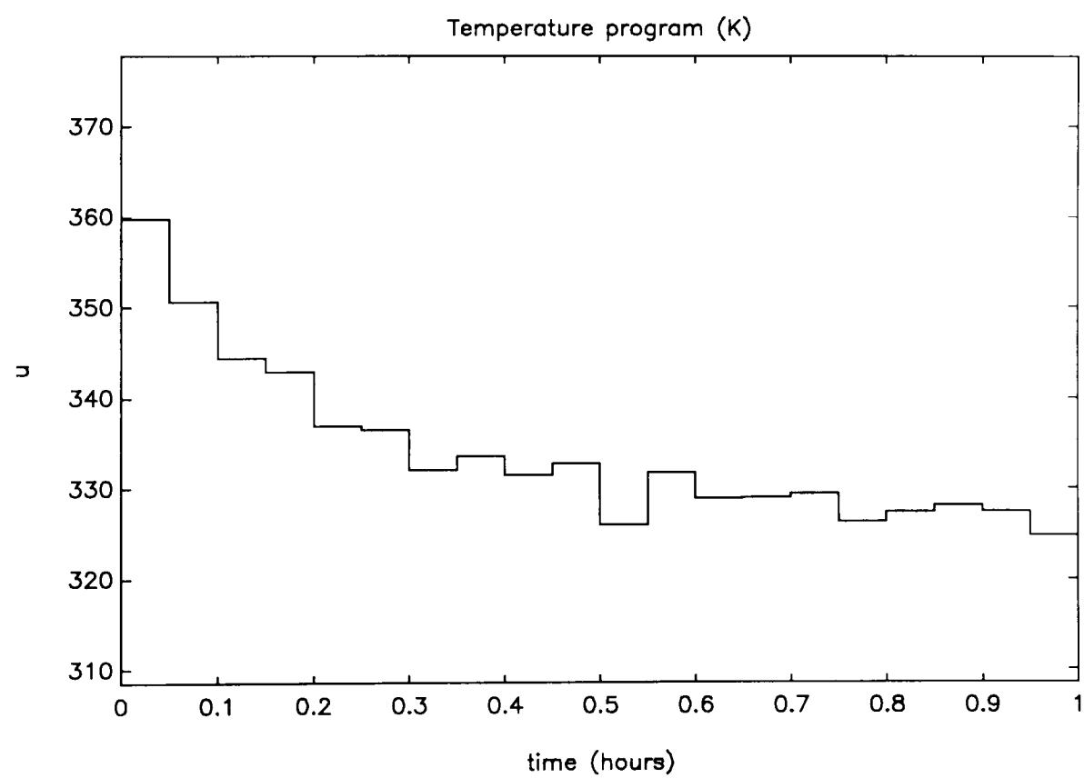
Figure 8.7.1.2: Example 8.7.1, final temperature profile
