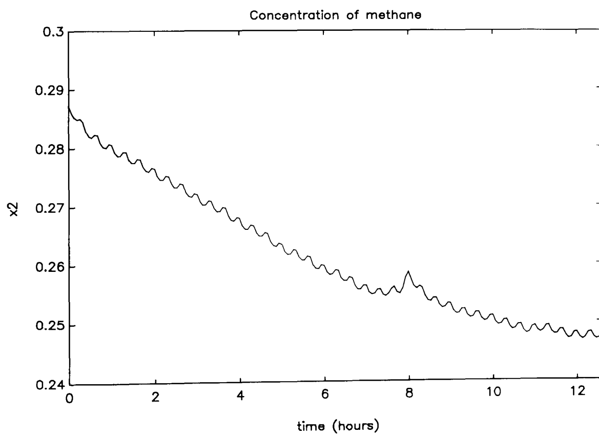
Figure 10.6.2.13: Example 10.6.2.b, concentration of methane trajectory
