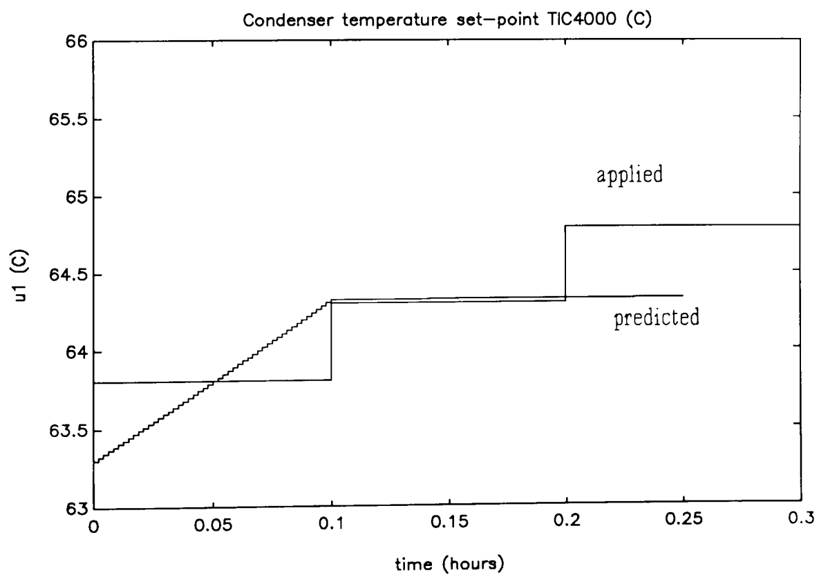
Figure 10.6.2.9: Example 10.6.2.a, predicted and applied condenser temperature controller set-point
