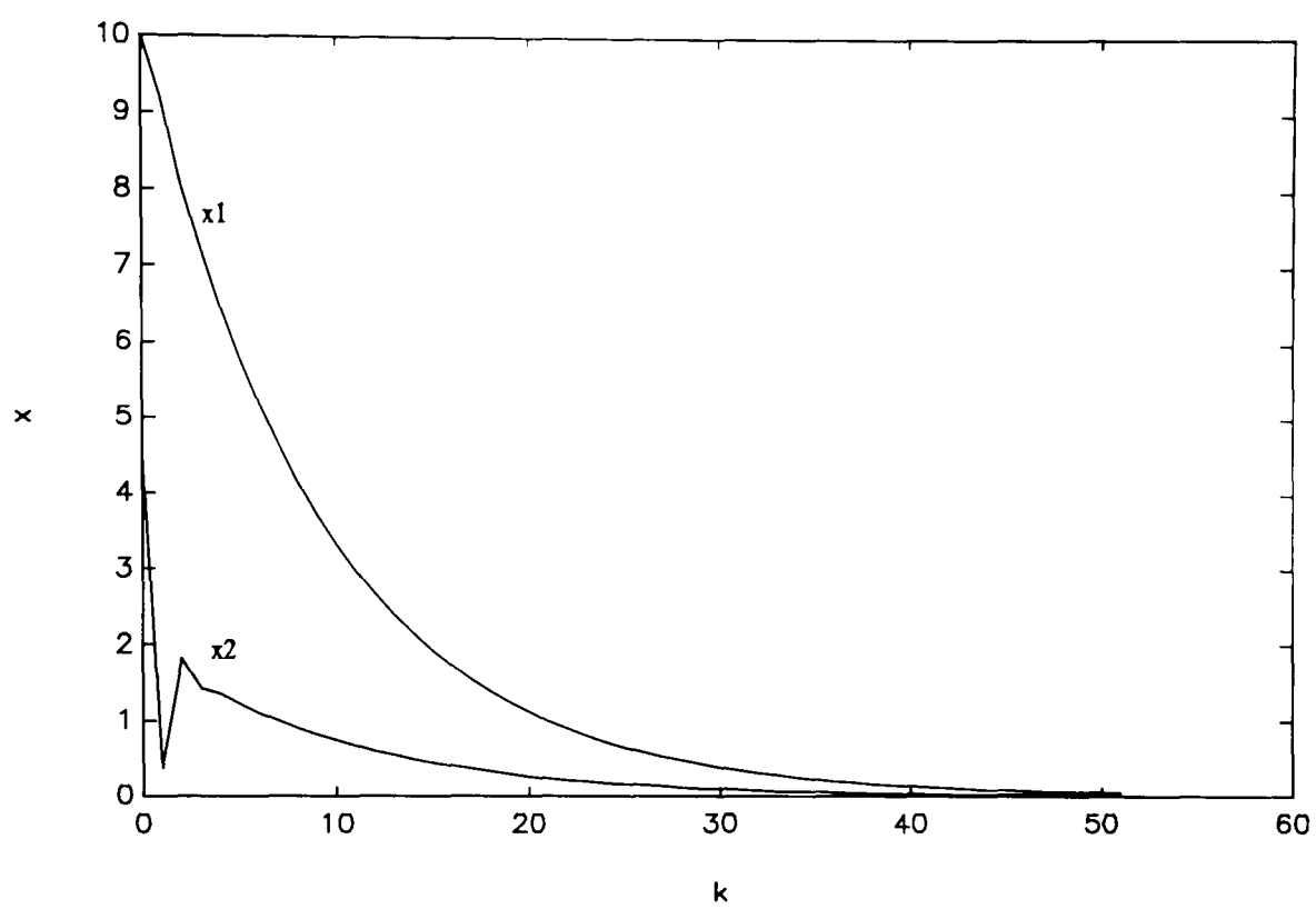
Figure 5.5.1.1: Example 5.5.1, final state response
