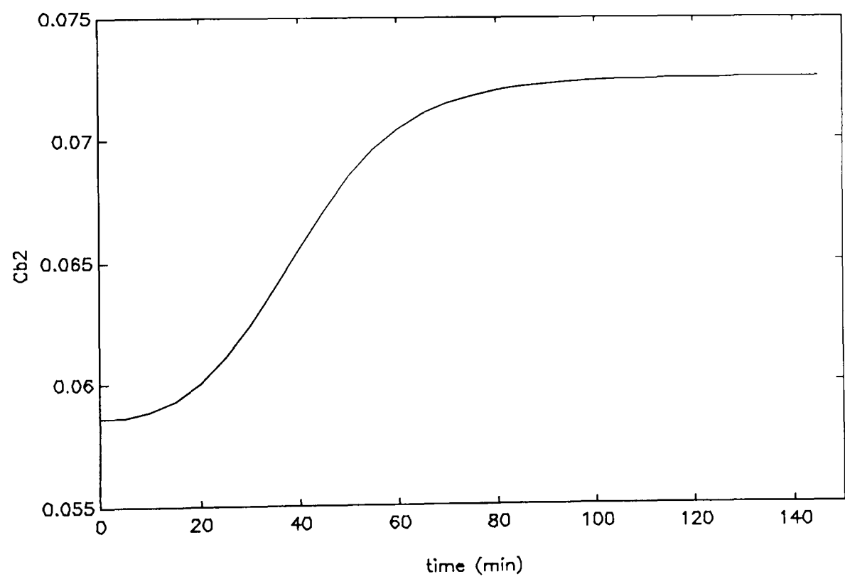
Figure 9.5.4.1: Example 9.5.4, trajectory of concentration of B in the second reactor
