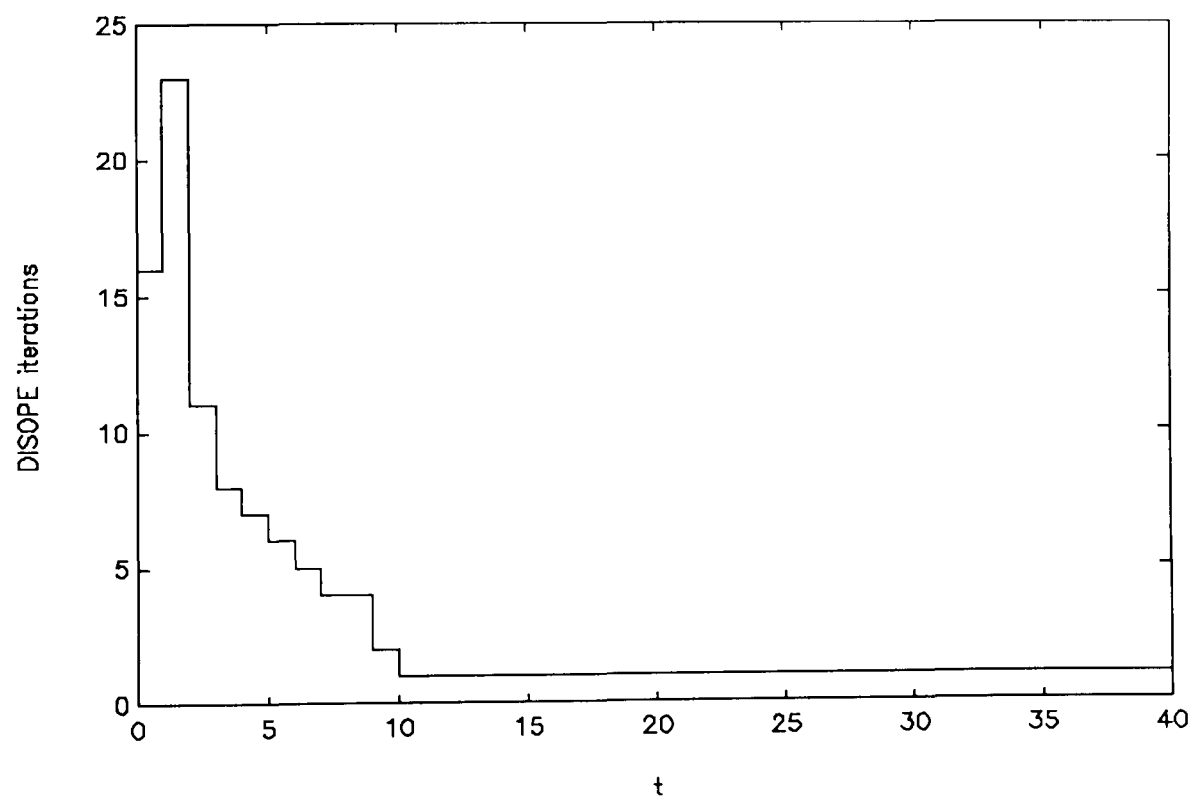
Figure 9.5.1.3: Example 9.5.1, number of DISOPE iterations per sample interval
