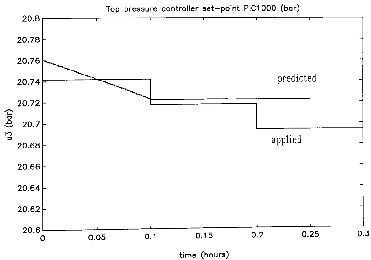
Figure 10.6.2.11: Example 10.6.2.a, predicted and applied top pressure controller set-point
