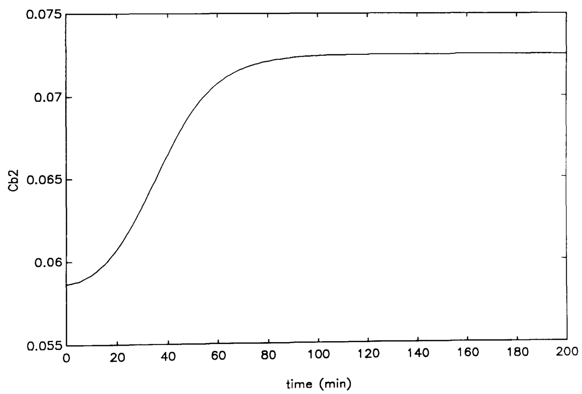
Figure 10.6.3.3: Example 10.6.3b, trajectory of concentration of B in the second reactor
