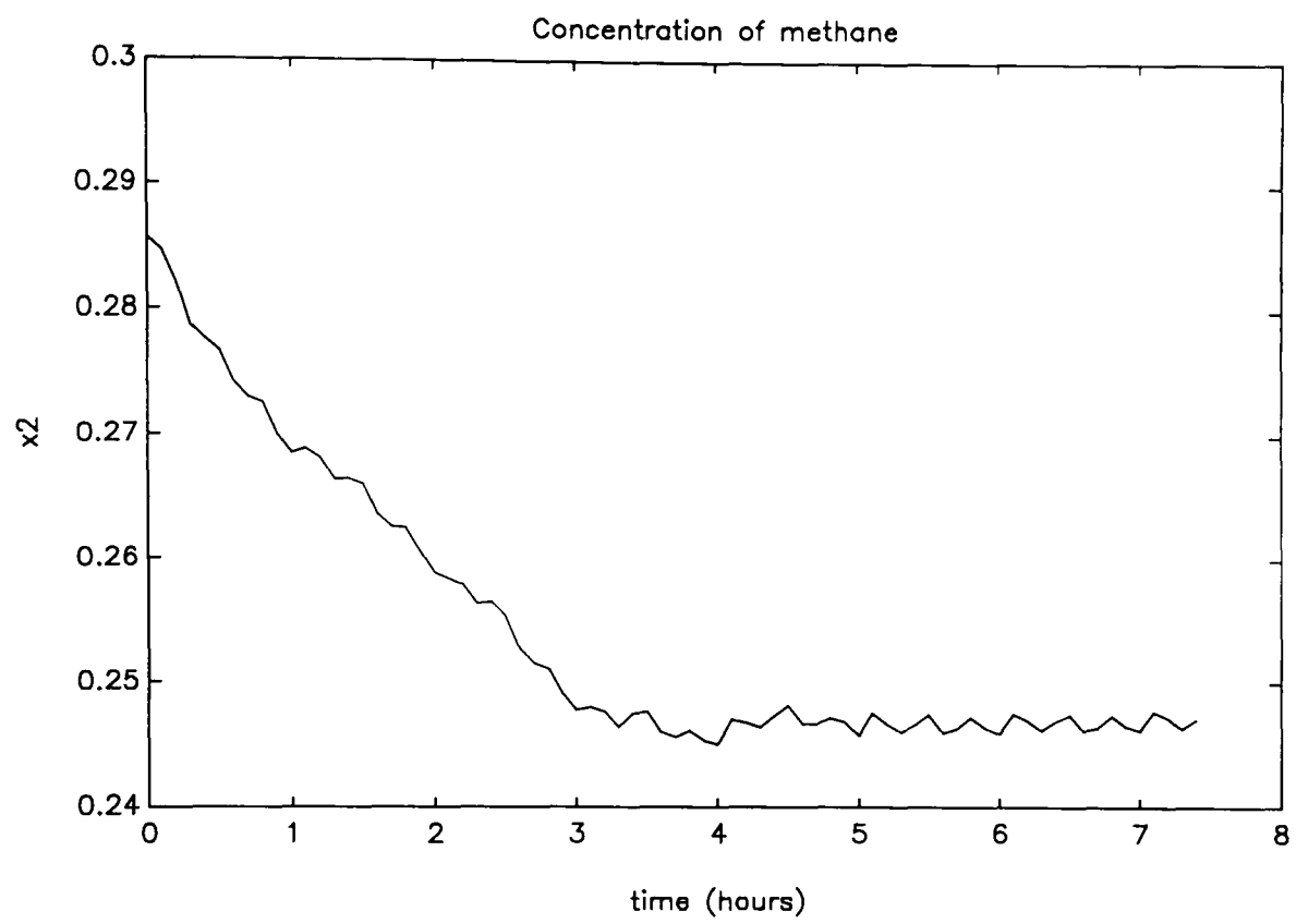
Figure 10.6.2.2: Example 10.6.2.a, concentration of methane trajectory
