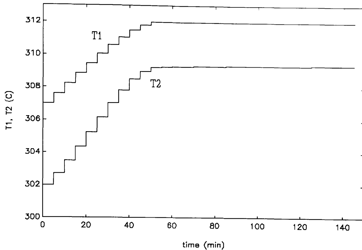
Figure 9.5.4.2: Example 9.5.4, control signals, temperatures in reactors 1 and 2
