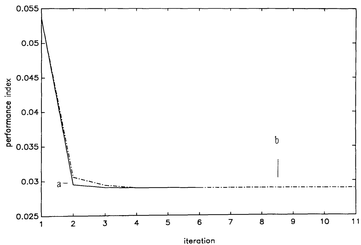
Figure 3.4.1.2: Example 3.4.1, Convergence of the performance index
