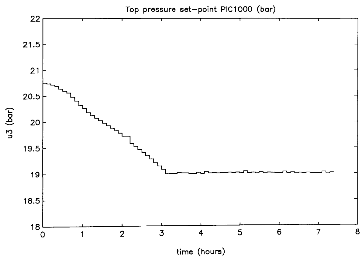
Figure 10.6.2.5: Example 10.6.2.a, top pressure controller set-point
