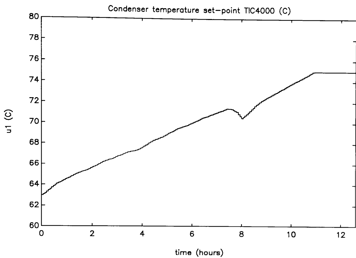
Figure 10.6.2.14: Example 10.6.2.b, condenser temperature controller set-point
