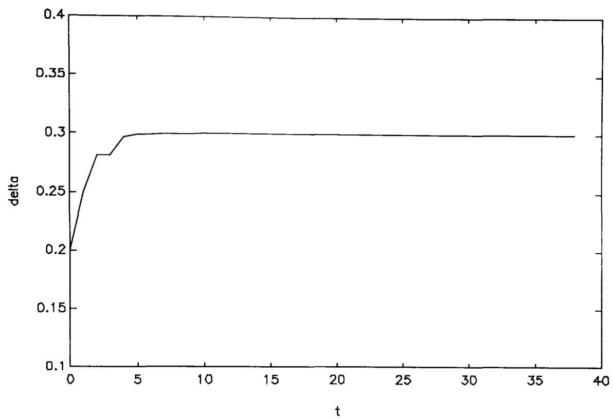
Figure 9.5.2.3: Example 9.5.2, parameter estimate, case (b)
