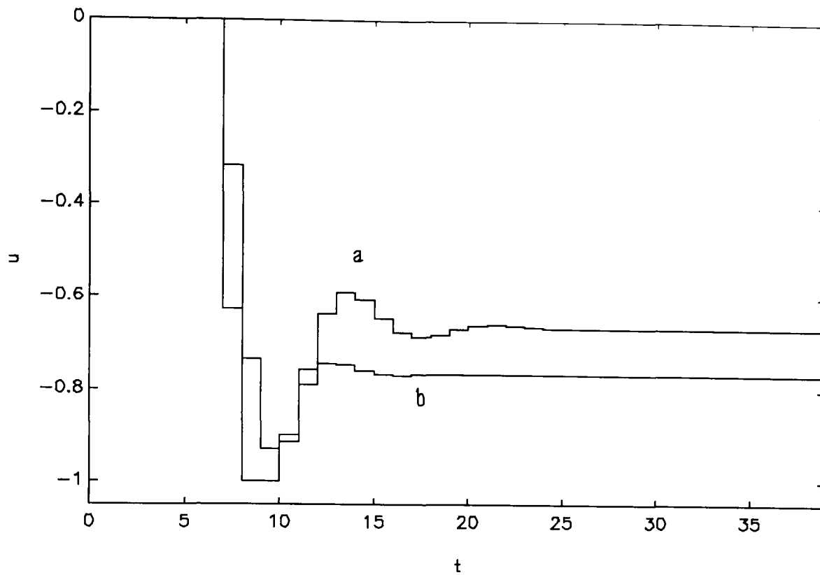
Figure 9.5.3.3: Example 9.5.3, control signal for cases (a) and (b)
