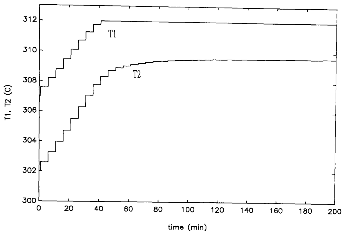
Figure 10.6.3.4: Example 10.6.3b, control signals, temperatures in reactors 1 and 2
