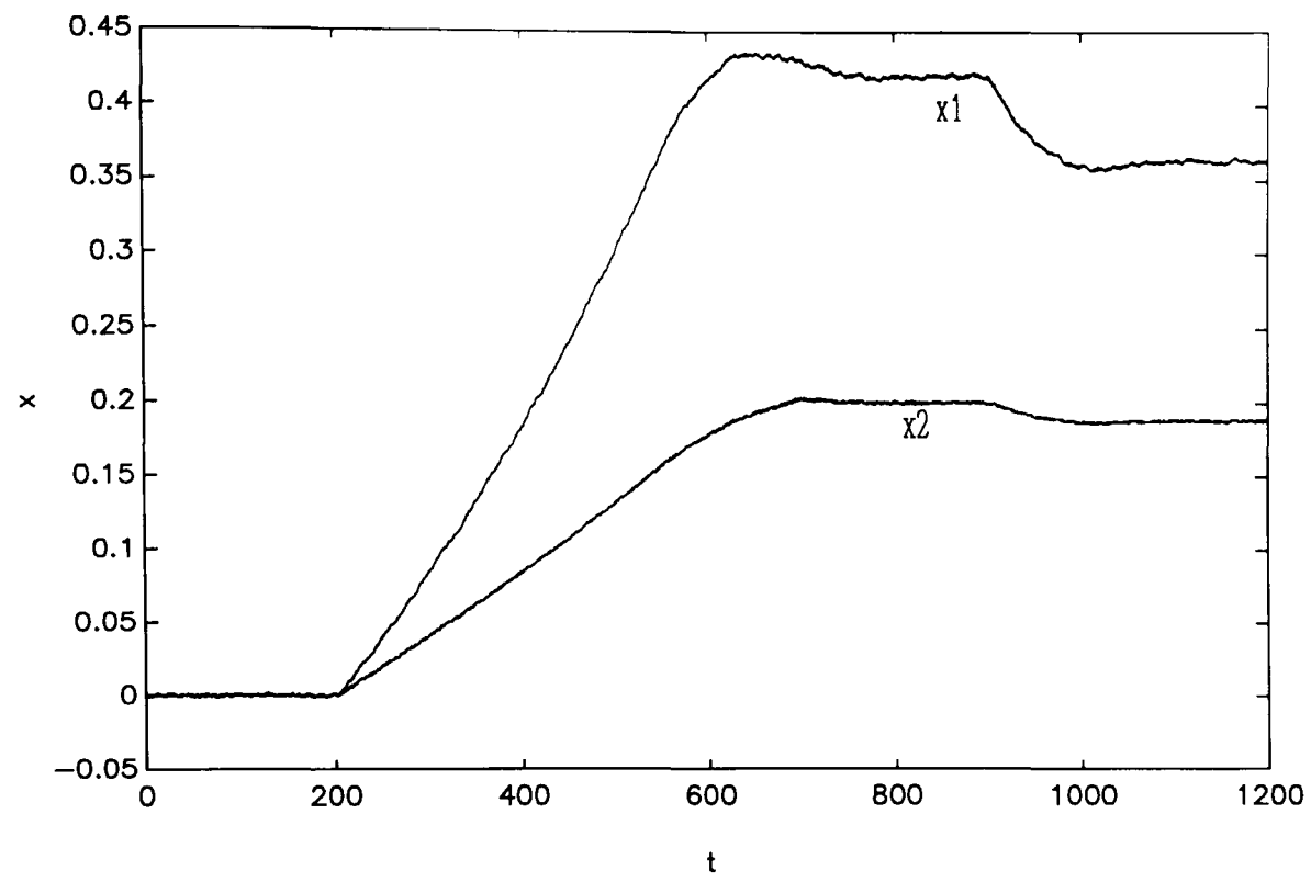
Figure 10.6.1.2: Example 10.6.1, state trajectory
