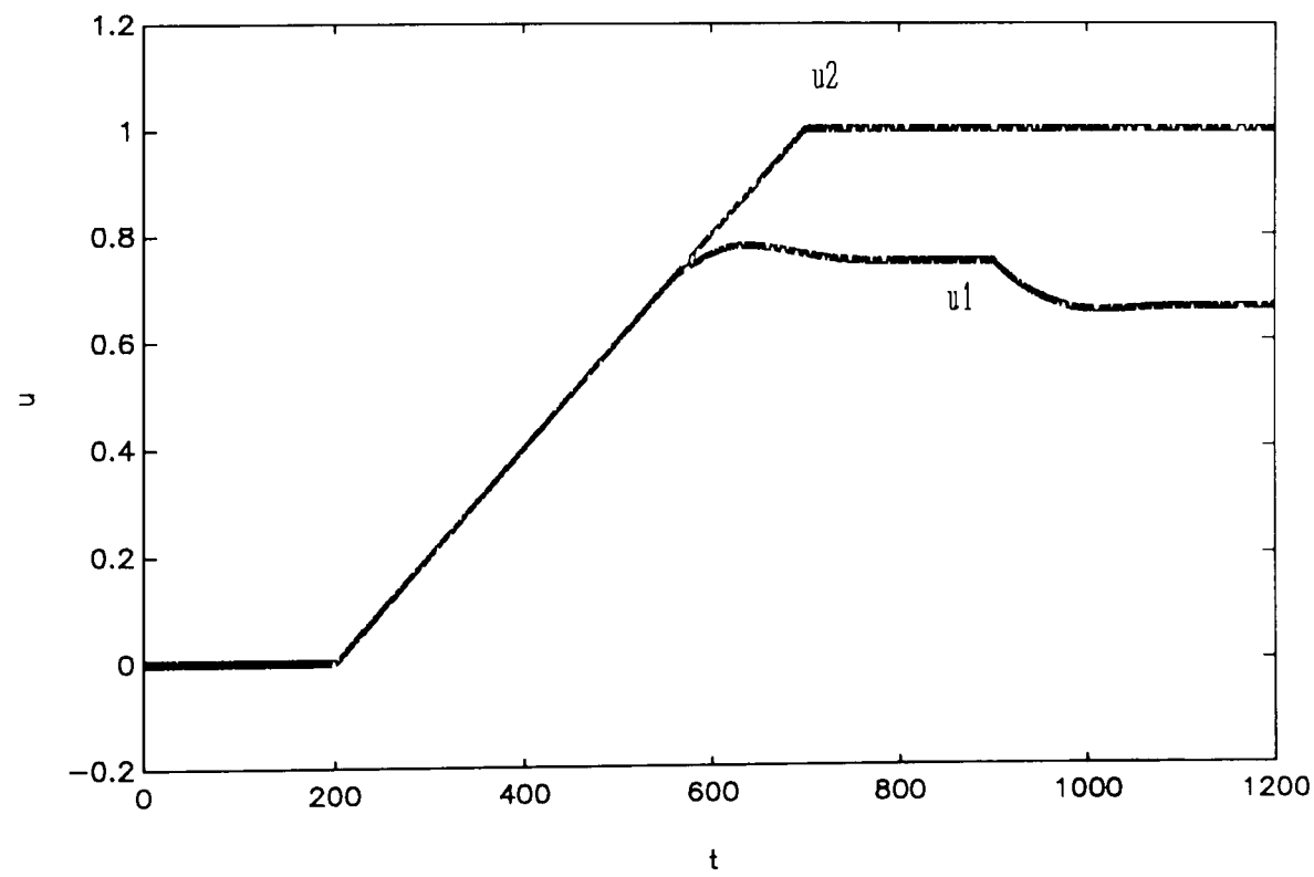
Figure 10.6.1.1: Example 10.6.1, control signals
