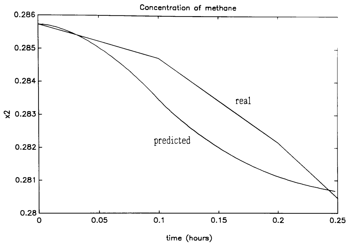
Figure 10.6.2.8: Example 10.6.2.a, concentration of methane predicted and actual trajectories
