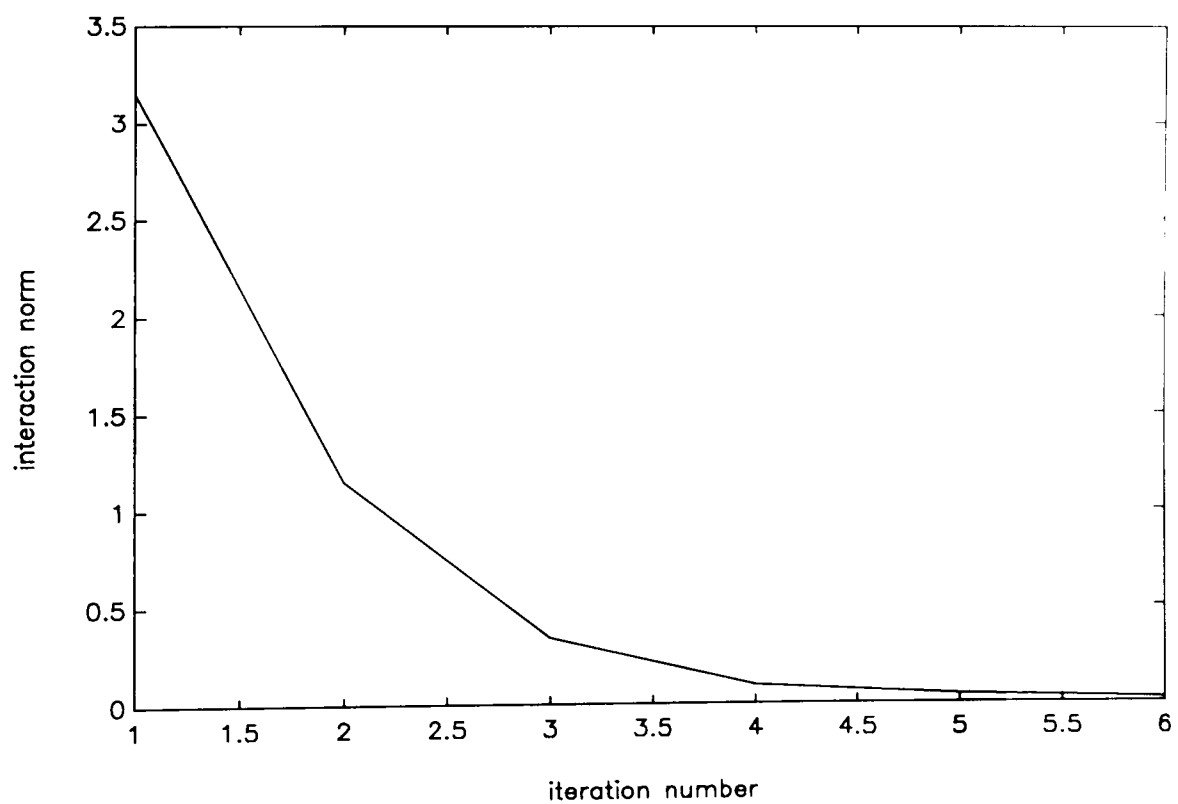
Figure 4.4.1.8: Example 4.4.1, interaction norm vs. iteration (hierarchical case)
