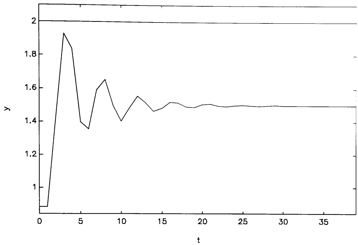
Figure 9.5.2.1: Example 9.5.2, dimensionless temperature and set-point, case (a).
