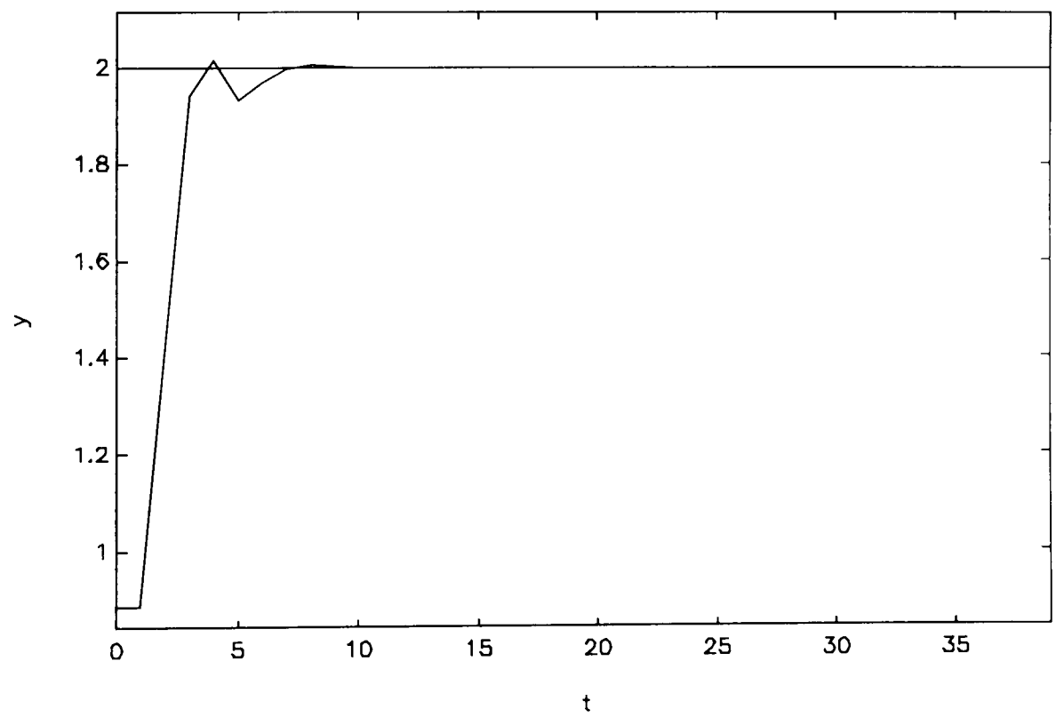
Figure 9.5.2.2: Example 9.5.2, dimensionless temperature and set-point, case (b).
