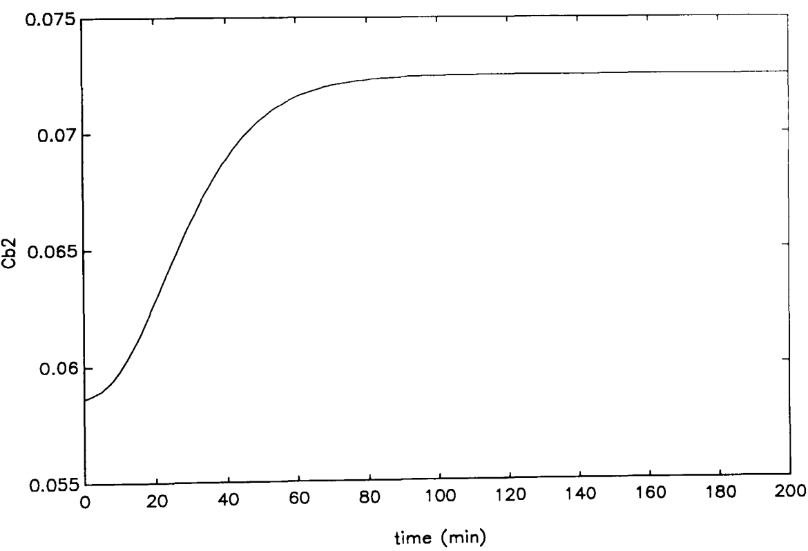
Figure 10.6.3.1: Example 10.6.3a, trajectory of concentration of B in the second reactor
