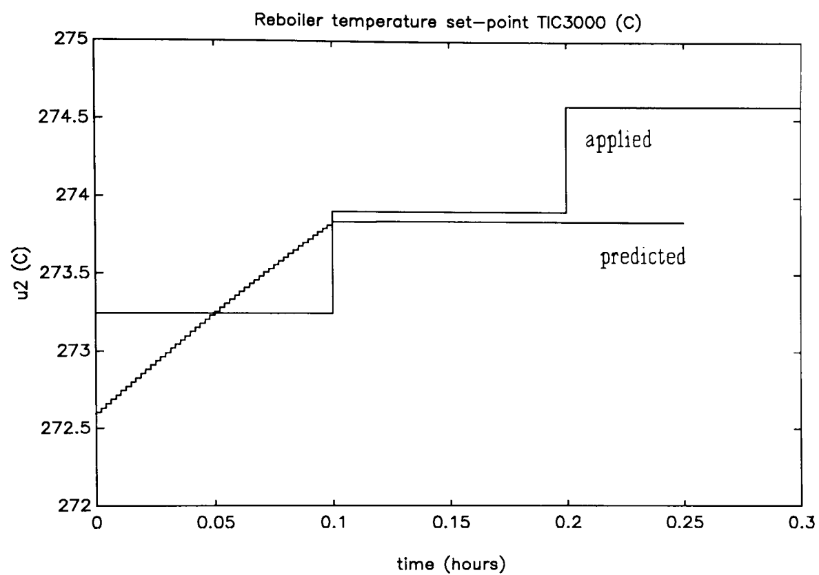
Figure 10.6.2.10: Example 10.6.2.a, predicted and applied reboiler temperature controller set-point
