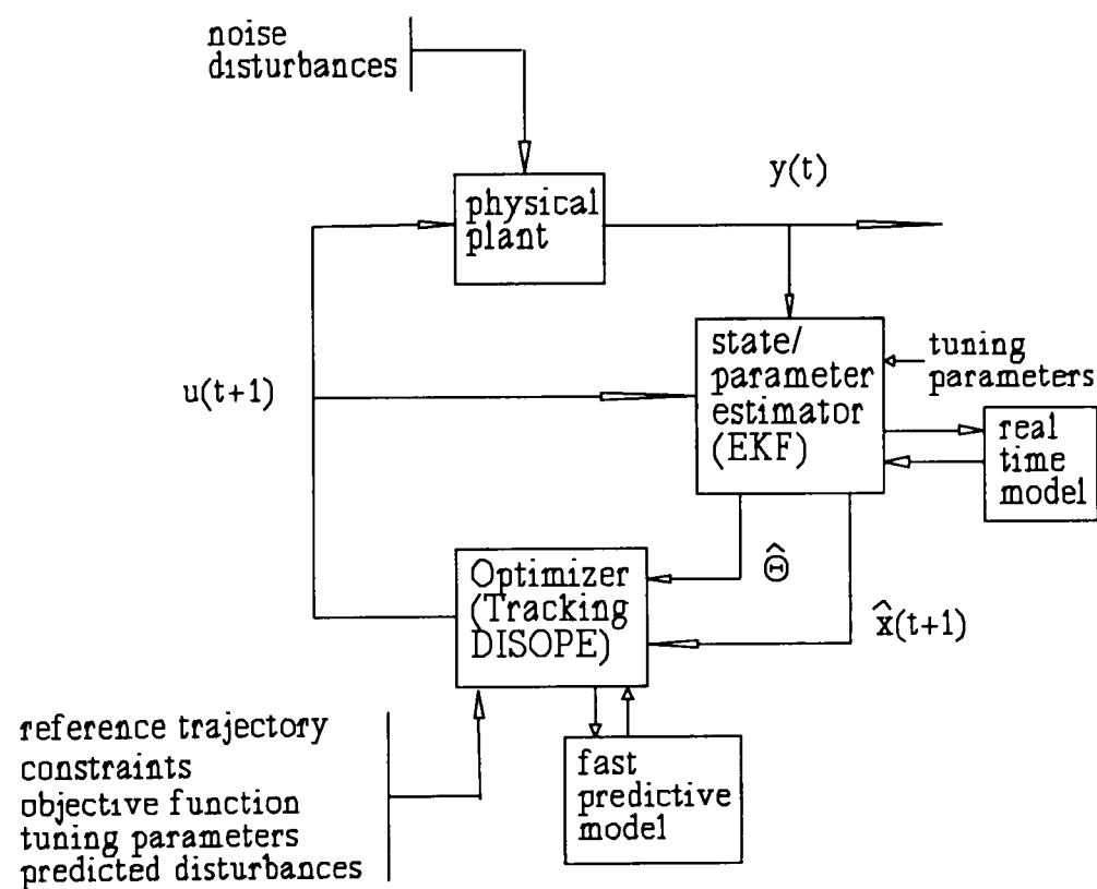
Figure 9.2.2: Schematic diagram of the controller
