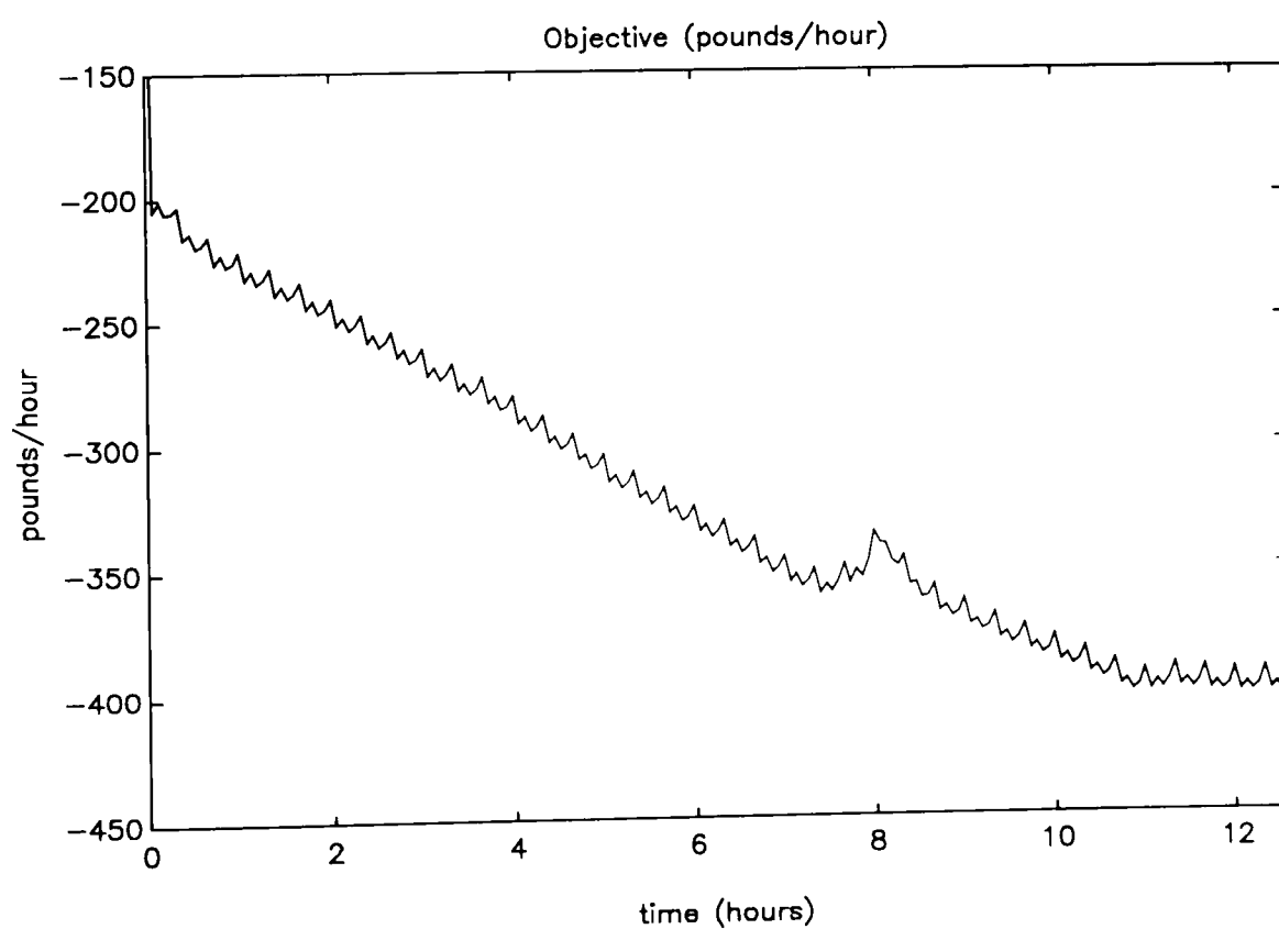
Figure 10.6.2.17: Example 10.6.2.b, evolution of the steady-state objective function
