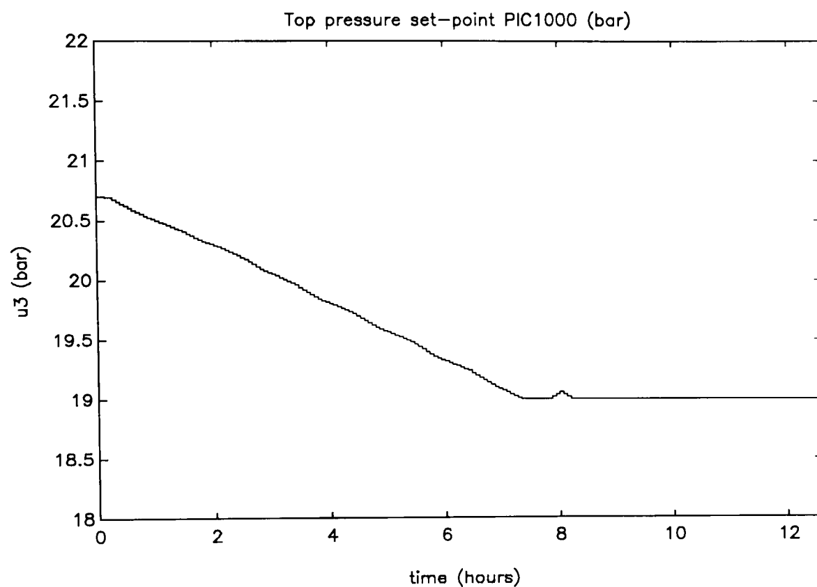
Figure 10.6.2.16: Example 10.6.2.b, top pressure controller set-point
