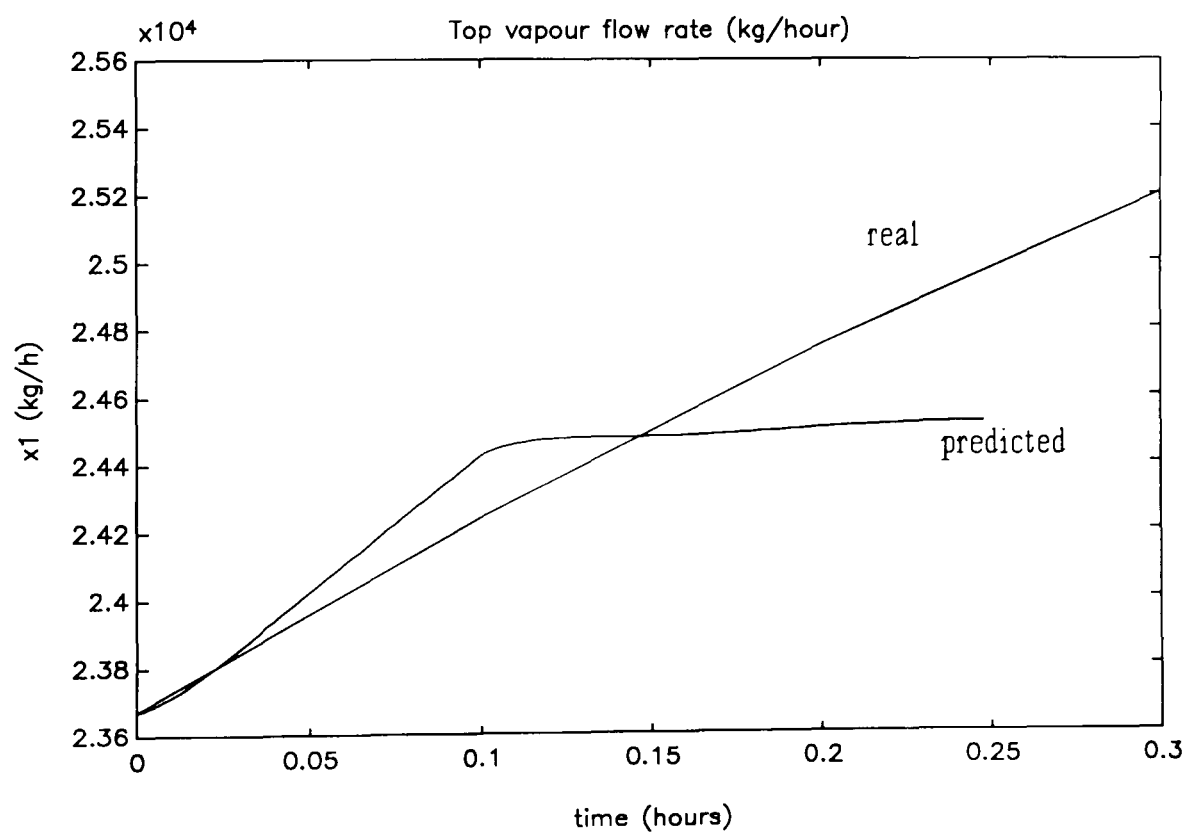
Figure 10.6.2.7: Example 10.6.2.a, Top vapour flow rate predicted and actual trajectories
