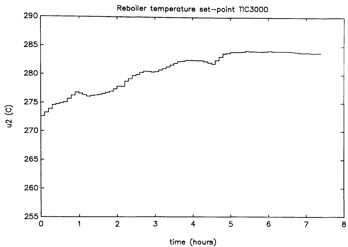
Figure 10.6.2.4: Example 10.6.2.a, reboiler temperature controller set-point
