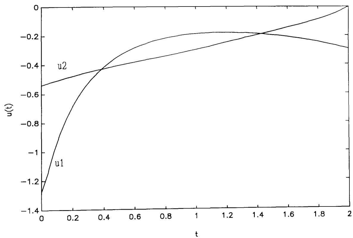
Figure 2.4.2.2: Example 2.4.2, final control signals
