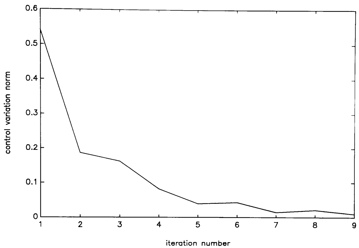
Figure 5.5.2.3: Example 5.5.2, control variation norm vs. iterations
