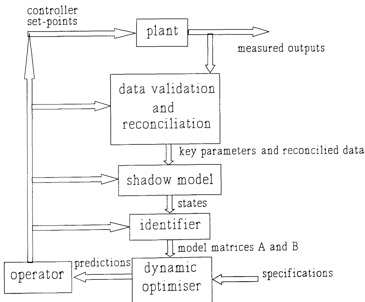
Figure 10.1: Simplified diagram of shadow model approach for plant dynamic optimisation
