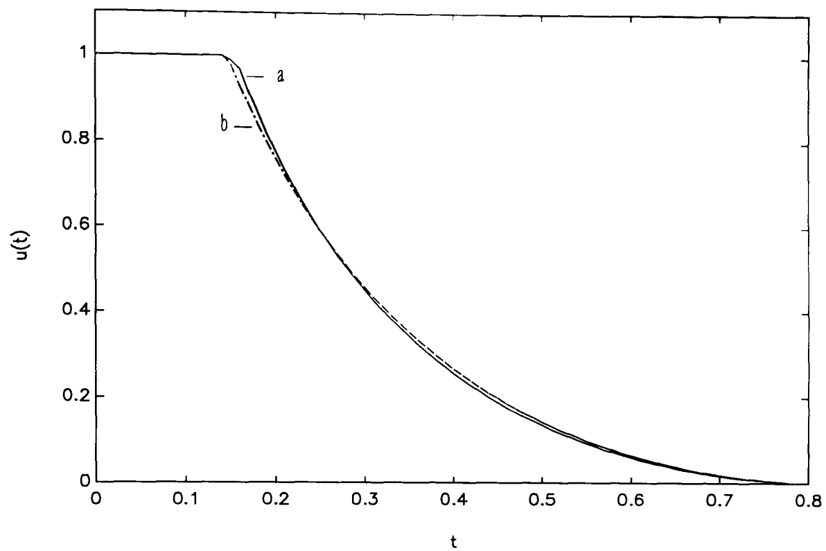
Figure 3.4.1.1: Example 3.4.1, final control signal
