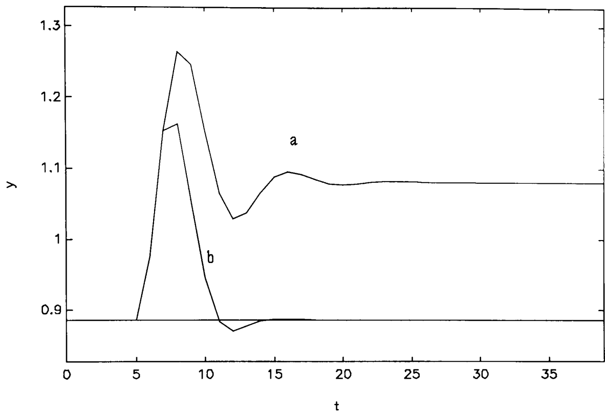
Figure 9.5.3.1: Example 9.5.3, dimensionless temperature and set-point, cases (a), (b).
