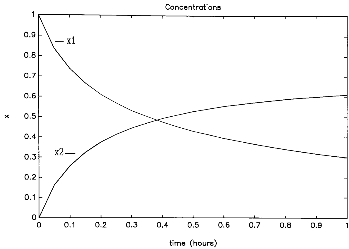
Figure 8.7.1.1: Example 8.7.1, final concentration responses
