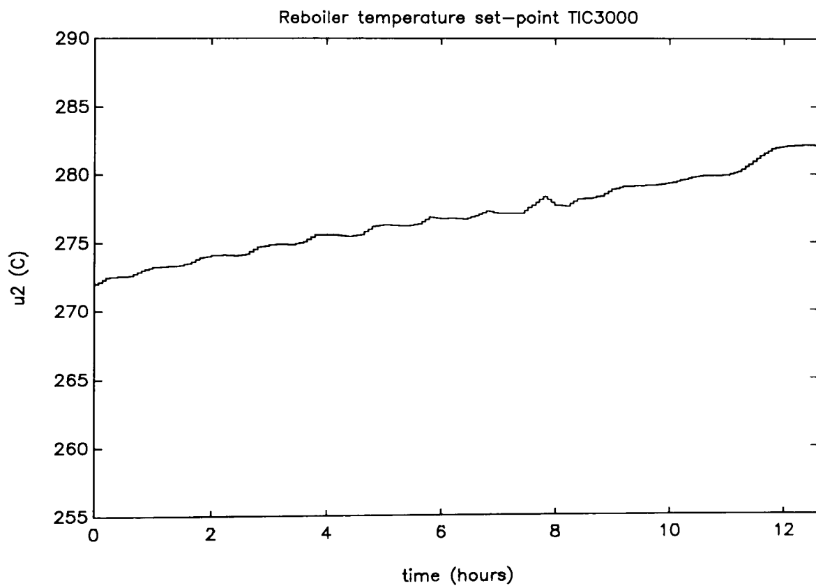
Figure 10.6.2.15: Example 10.6.2.b, reboiler temperature controller set-point
