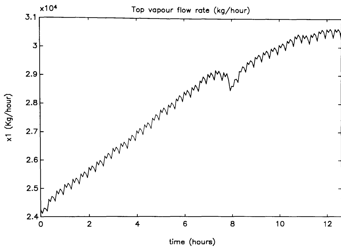
Figure 10.6.2.12: Example 10.6.2.b, top vapour flow rate trajectory
