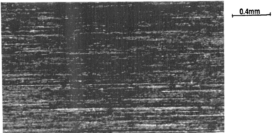
FIG.114a OPTICAL MICROGRAPH OF SURFACE PROIR TO TESTING ARMCO IRON
