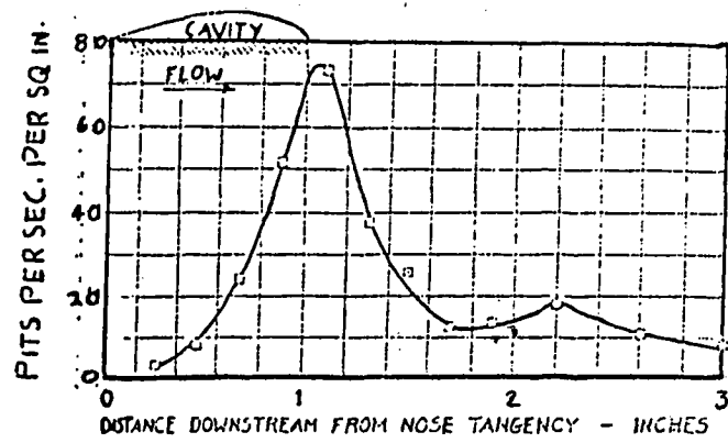
Fig.17 Distribution of Pitting for 1-in Cavity length
