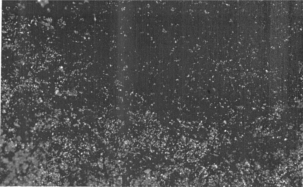
FIG.117d OPTICAL MICROGRAPH OF DEFORMED SURFACE OF TOOL STEEL (120 min)
