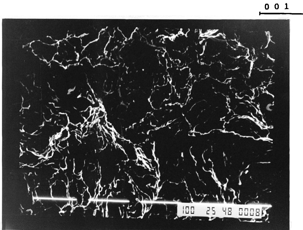
FIG.111c SCANNING ELECTRON MICROGRAPH OF DAMAGE IN CENTRAL ZONE AFTER TEST COMPLETION (160 min.)
