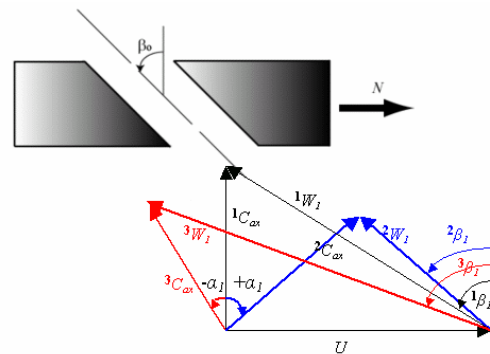
Figure 10: Velocity vectors at the inlet. ^1C_{ax} is inlet velocity with zero pre-swirl ( \alpha_1 = 0^\circ ), ^2C_{ax} is a +ve pre-swirl ( \alpha_1 > 0^\circ ), while ^3C_{ax} is a -ve pre-swirl ( \alpha_1 < 0^\circ ).
