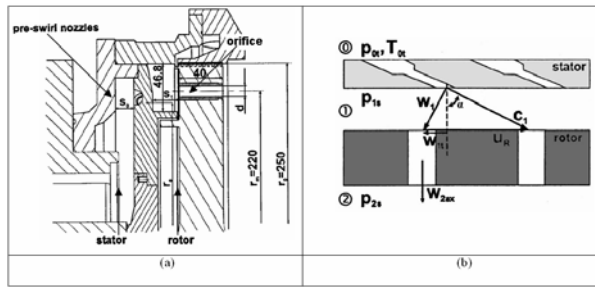
Figure 5: Dittmann et al. (2002) test rig (a) The position of the pre-swirl nozzles within the stator with a distance s_1 from the orifice. (b) The velocity vectors show the pre-swirl velocity ( C_1 ), the inlet relative velocity ( W_1 ), pre-swirl angle ( \alpha ), relative inlet tangential velocity ( W_{1t} = W_{10} ), and ideal velocity ( W_{2ax} = C_{1d,rel} ) [Note: the notations ( W_{1t} , W_{2ax} ) used in Dittmann et al. (2002) are slightly different from the present study.]
