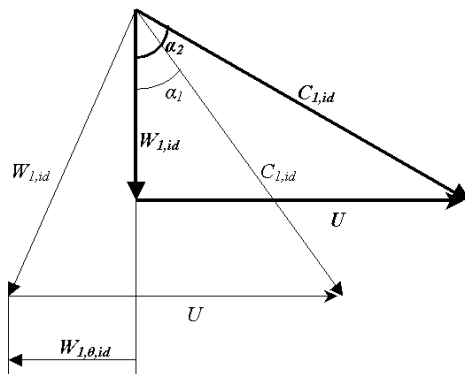
Figure 7: Velocity vectors describe how the tangential relative velocity ( W_{10} ) changes for different values of pre-swirl angle ( \alpha_1 to \alpha_2 ).
