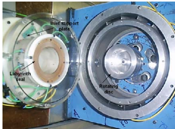
Figure 1: The assembly of the rotating orifices
