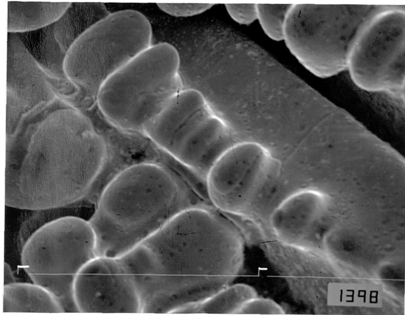
Fig. 8.11 Interdendritic type of fracture in the Nb containing steel in the "reheated as cast" condition tested at 900 °C, showing that most of the Mn(Fe)S inclusions have redissolved.
