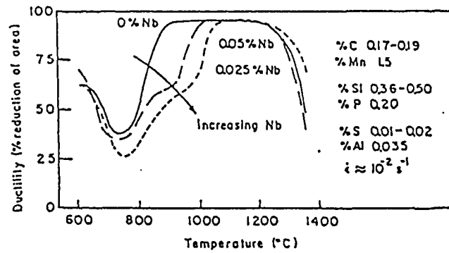
Fig. 3.11 Influence of Nb on hot ductility of C-Mn-Nb-Al steels. (After Bernard et al., 1978).
