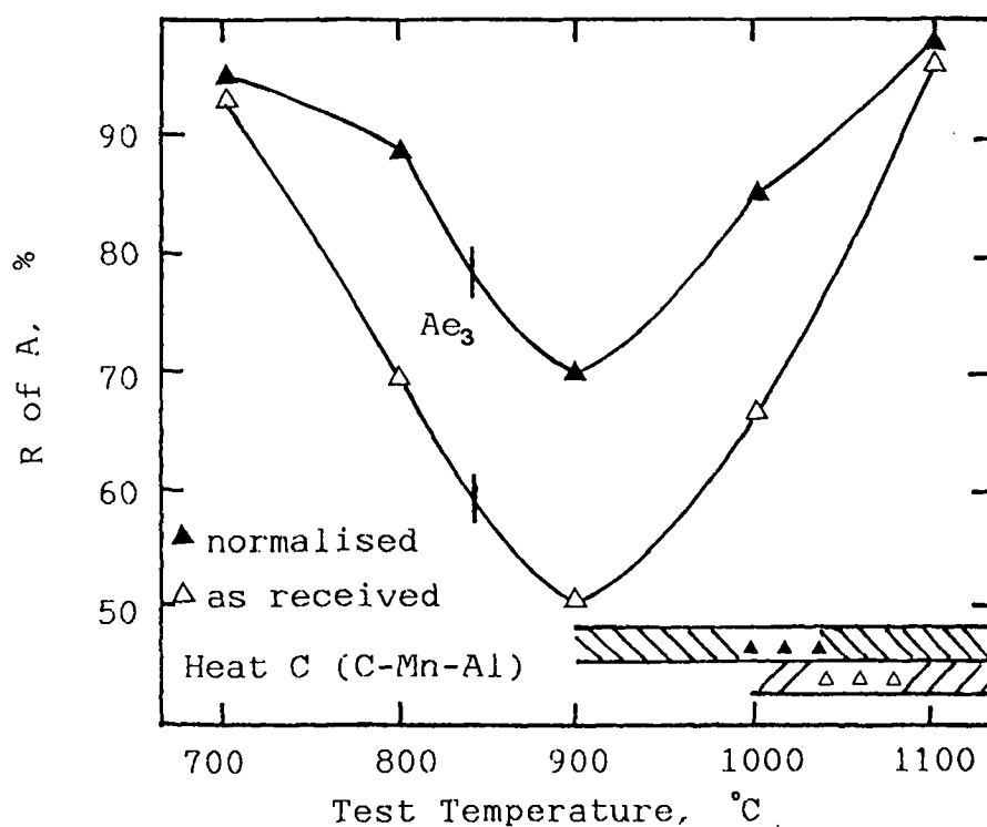
Fig. 9.6 Hot ductility curves for the Al containing steel with high S content in normalised and as received conditions.
