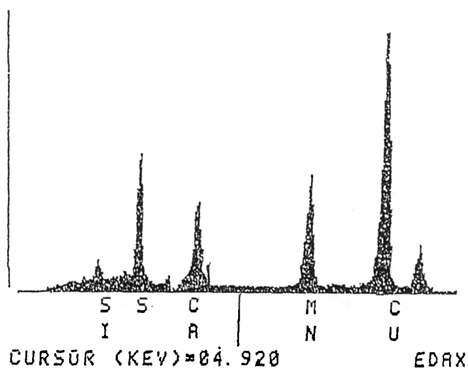
Fig. 6.14 (Mn,Ca)S inclusions observed in the Ca treated steels at 850 °C. with associated X-ray spectrum.
