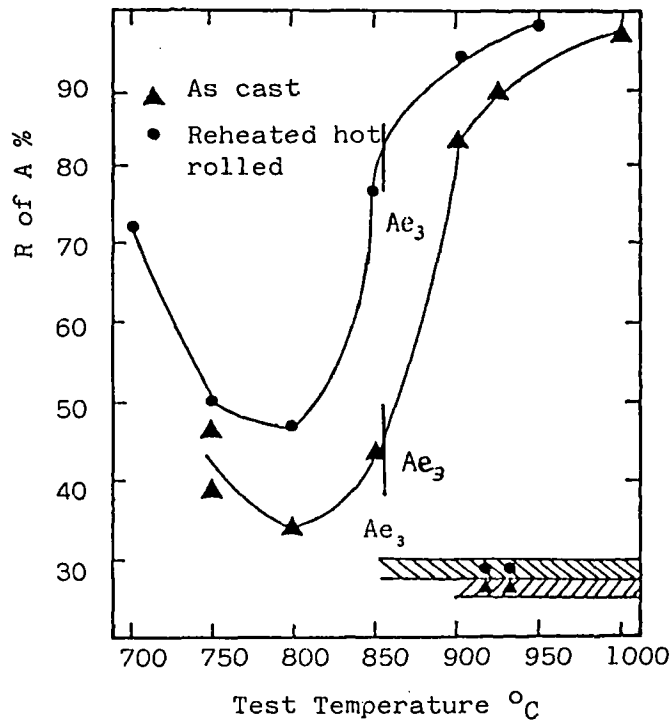
Fig. 8.4 Hot ductility curves for the Al steel, occurrence of dynamic recrystallisation indicated by shaded regions.
