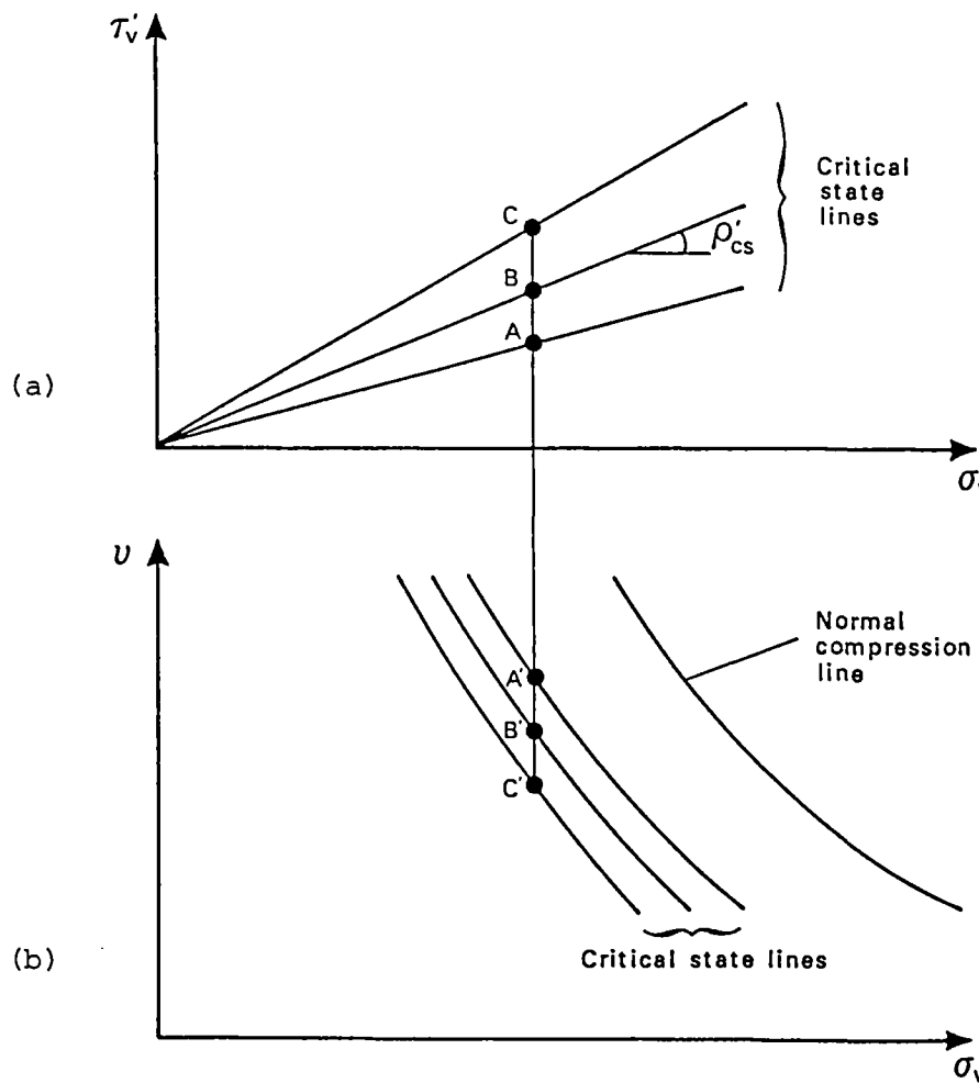
Figure 2.22 Critical state lines for simple shear tests
