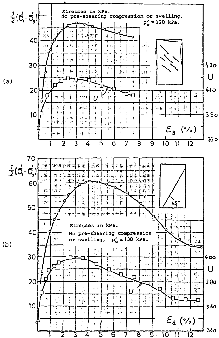
Figure 3.32 Stress-strain curves for undrained triaxial tests on undisturbed London clay (after Sandroni, 1977)
