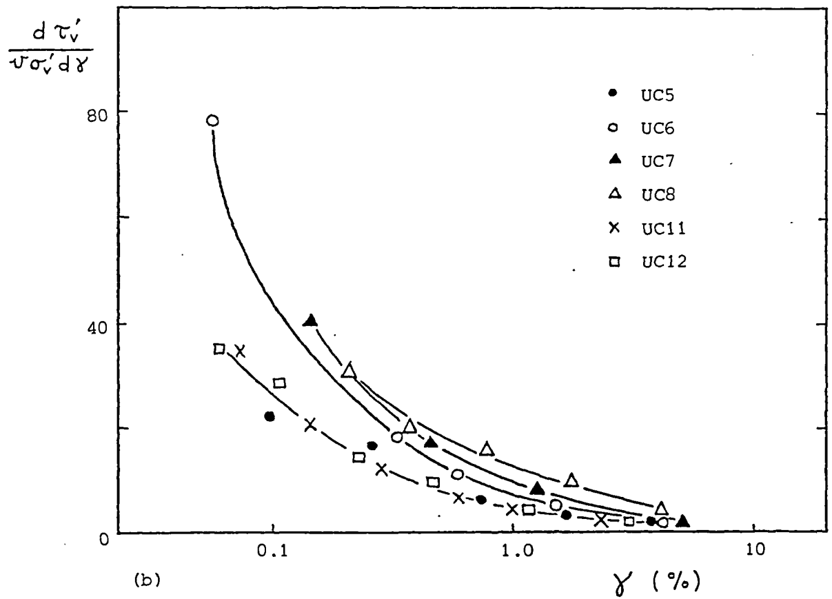
Figure 7.93 Variation of normalised tangent shear stiffness with logarithm of shear strain for undisturbed Cowden till simple shear samples
