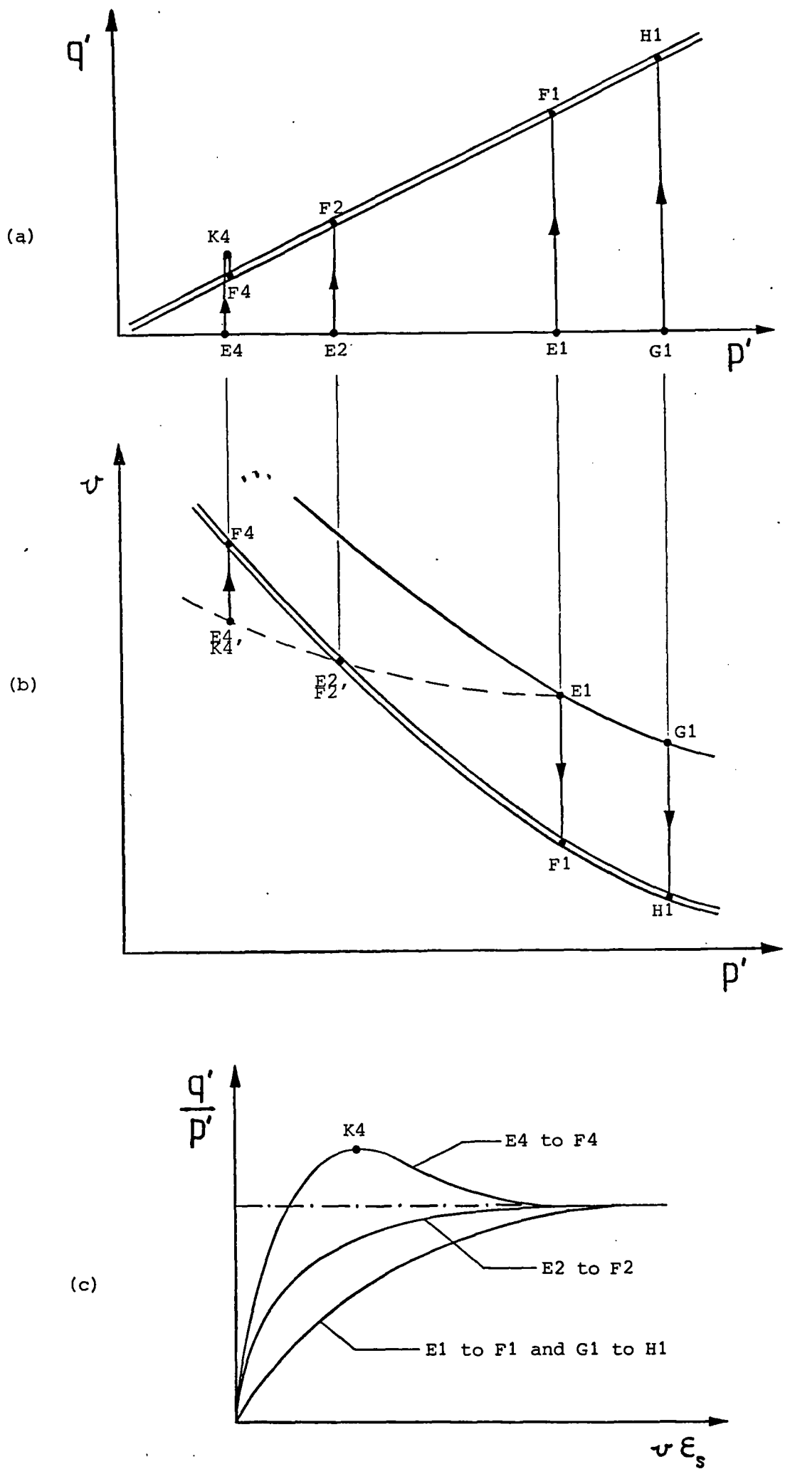
Figure 2.24 Idealised behaviour of soil in constant p' triaxial compression tests
