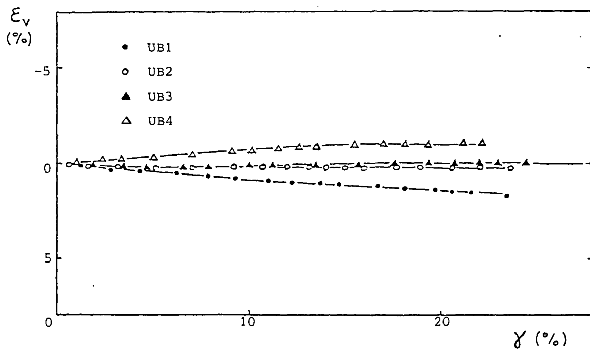
Figure 6.13 Results of shearing from undisturbed London clay (brown) simple shear samples
