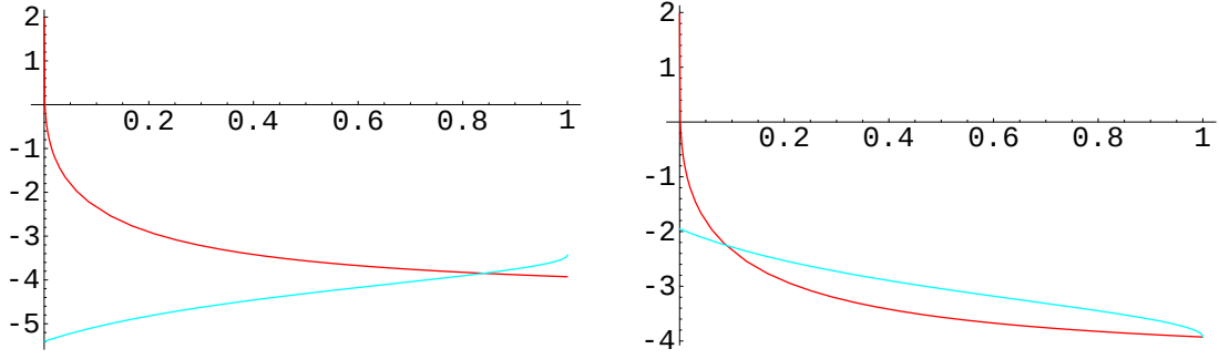
Figure 2: The intersection showing the roots of Det inside the region x \in (0, 1] . The (red) convex descending curve in both cases is that of 2h(x) . In the graph to the left, we have chosen b = 1, B = 0.1 and have shown a typical intersection of 2f(x) with the (blue) b - \frac{4B\pi^2\sqrt{1-x}}{\sqrt{1+3x}} - 4(\gamma + \log(4)) . There is always 1 point of intersection. On the graph to the right, we have chosen the limiting case b = 0, B = 0.1 and the (red) curve is now b + \frac{4B\pi^2\sqrt{1-x}}{\sqrt{1+3x}} - 4(\gamma + \log(4)) . There is always 1 point of intersection in between and here there is another at the endpoint x = 1 . For any other value of b , x = 1 would no longer be an intersection point.
