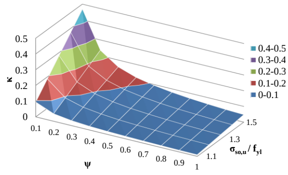
Fig. 7: Range of values of \kappa for typical values of \psi and \sigma_{so,u}/f_{yI}
