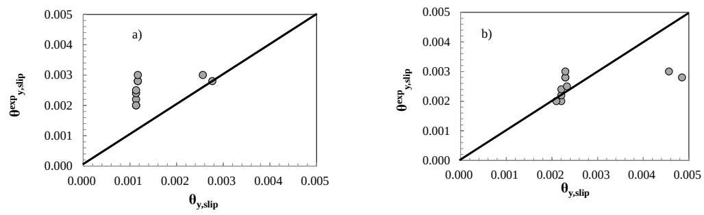
Fig. 8: Comparison of \theta_{y,slip} experimental data with analytical predictions by a) EC8-Part 3 [15]; b) proposed methodology
