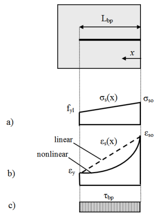
Fig. 5. Proposed solution methodology for inelastic fixed-end rotations: a) steel stress distribution; b) steel strain distribution and c) bond distribution along L_{bp}
