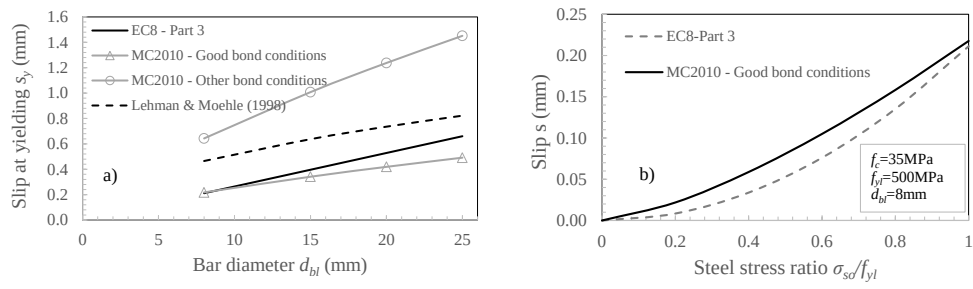
Fig. 4. Comparison of proposed model (with \tau - s from MC2010) and relationships from the literature: (a) s_y vs. d_{bl} ; (b) s vs. \sigma_{sd}/f_{yl}
