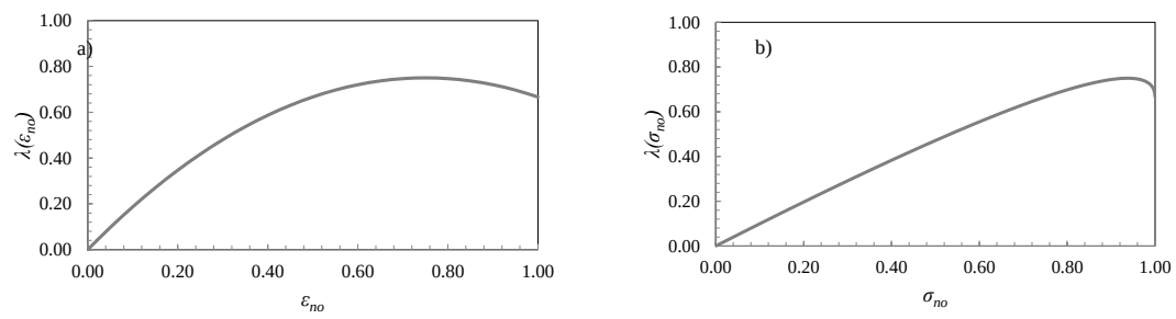
Fig. 6: Variation of \lambda with a) \epsilon_{no} ; b) \sigma_{no}
