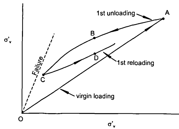
Figure 2.4 Influence of stress history on K_0 (Mayne and Kulhawy, 1982).
