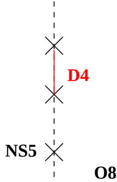
Figure 5: The D4 brane probe in type I'.
