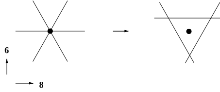
Figure 3: The 8d modulus for k = 3 .
