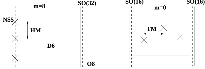
Figure 1: Examples of the two different phases in the type I' setup. Tensor multiplets correspond to motion on the compact 6 interval, hyper-multiplets to motion in the transverse 789 space. The m referred to the cosmological constant set up in the bulk.
