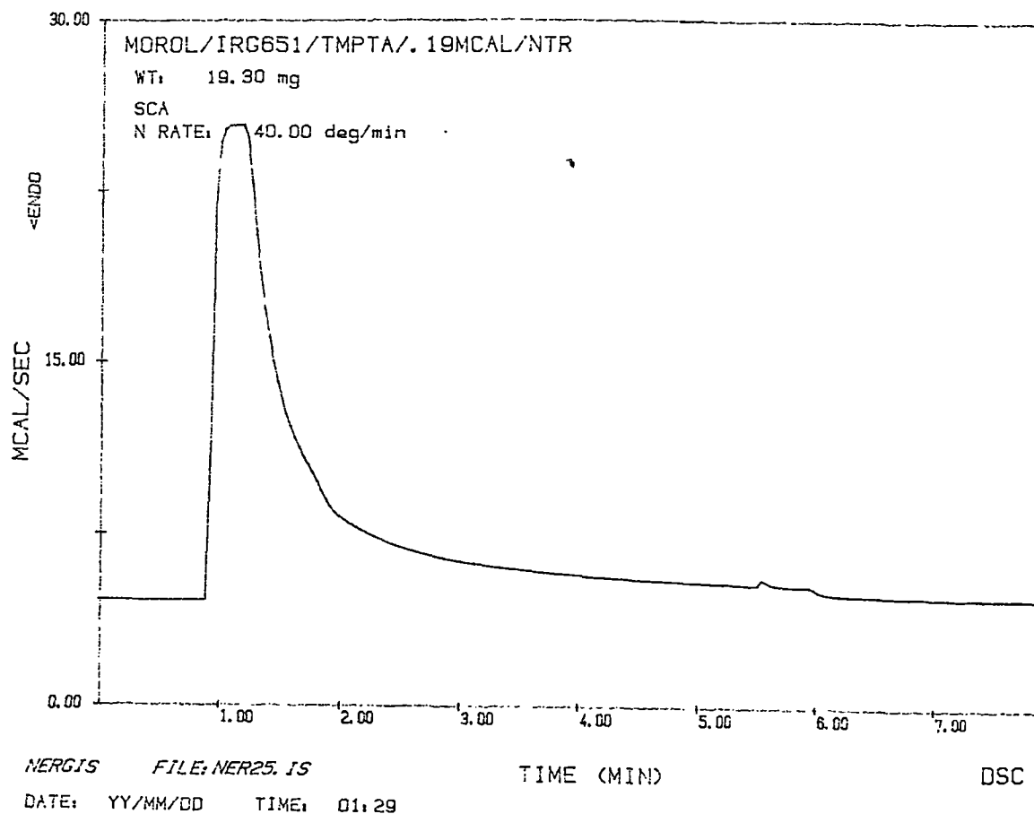
Fig 8.25. DSC trace for photopolymerisation of 2% IRG-651/1% 2-Benzyl-2-dimethylamino-1-(4-morpholinophenyl)-butan-1-ol (MOROL) in nitrogen.
