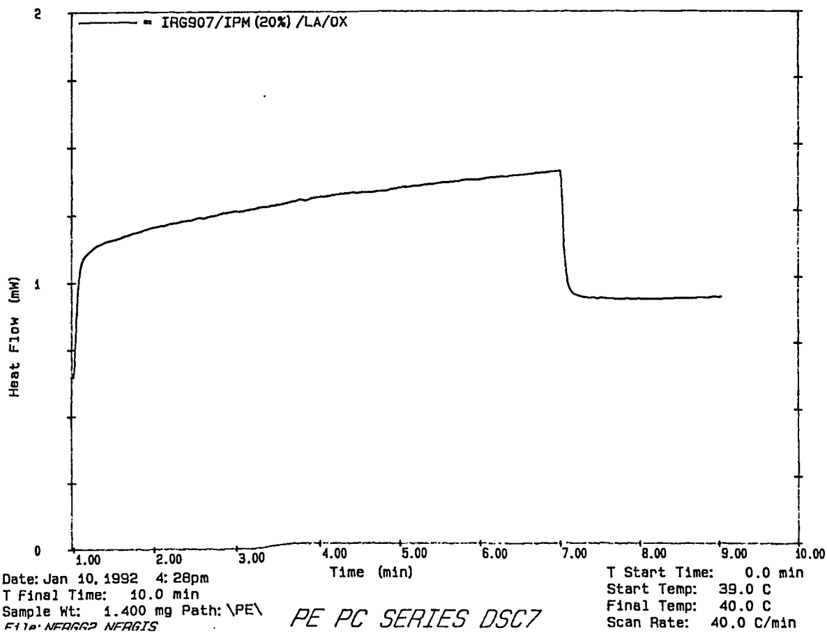
Fig 6.11. DSC trace of photopolymerisation of 2%IRG-907/20% IPM/LA.
