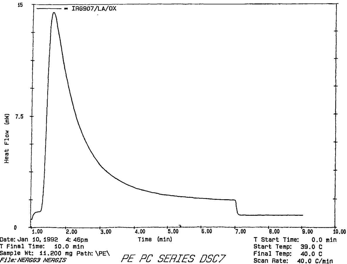
Fig 6.8. DSC trace for photopolymerisation of 2% IRG-907/LA.
