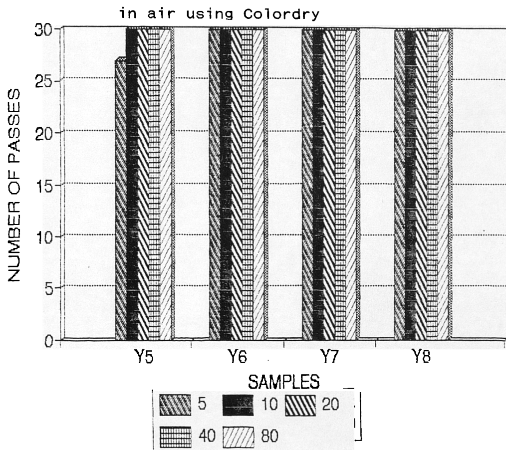
Fig 8.6 The curing results of samples (Y5-Y8)
