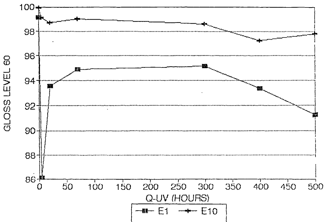
Fig 9.24 Gloss levels (60°) of UV-cured samples
