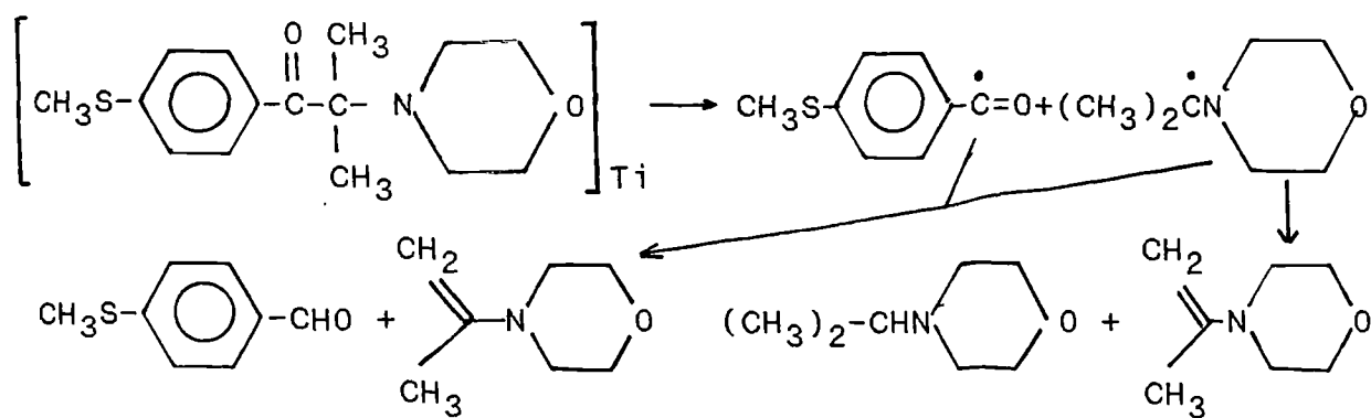
Scheme III
