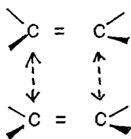
Fig. 1.6 [2_s + 2_s] cyclo-addition
