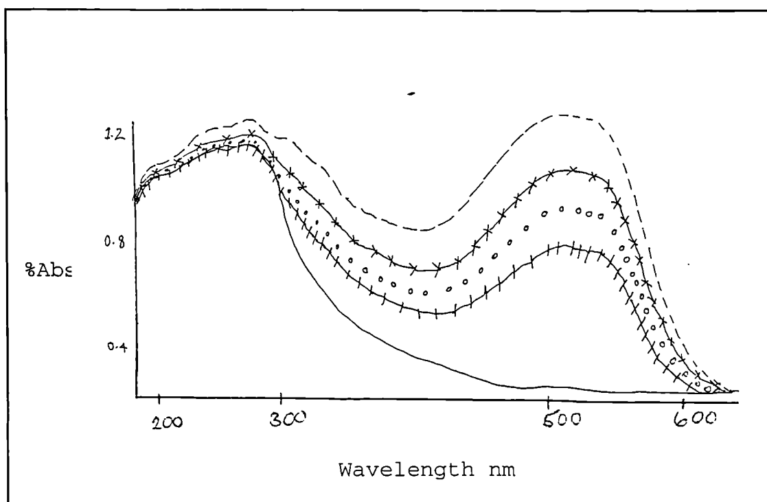
Figure 4:6 Diffuse reflectance spectra of blank wool, competitively dyed with \text{H}_3\text{PO}_2/\text{CH}_2\text{O} pretreated wool using Acid Red 37. — = blank wool alone, - - = 100% \text{H}_3\text{PO}_2 / 100% \text{CH}_2\text{O} , -*- = 50% \text{H}_3\text{PO}_2 / 100% \text{CH}_2\text{O} , ..... = 20% \text{H}_3\text{PO}_2 / 100% \text{CH}_2\text{O} and +++ = 10% \text{H}_3\text{PO}_2 / 100% \text{CH}_2\text{O} .
