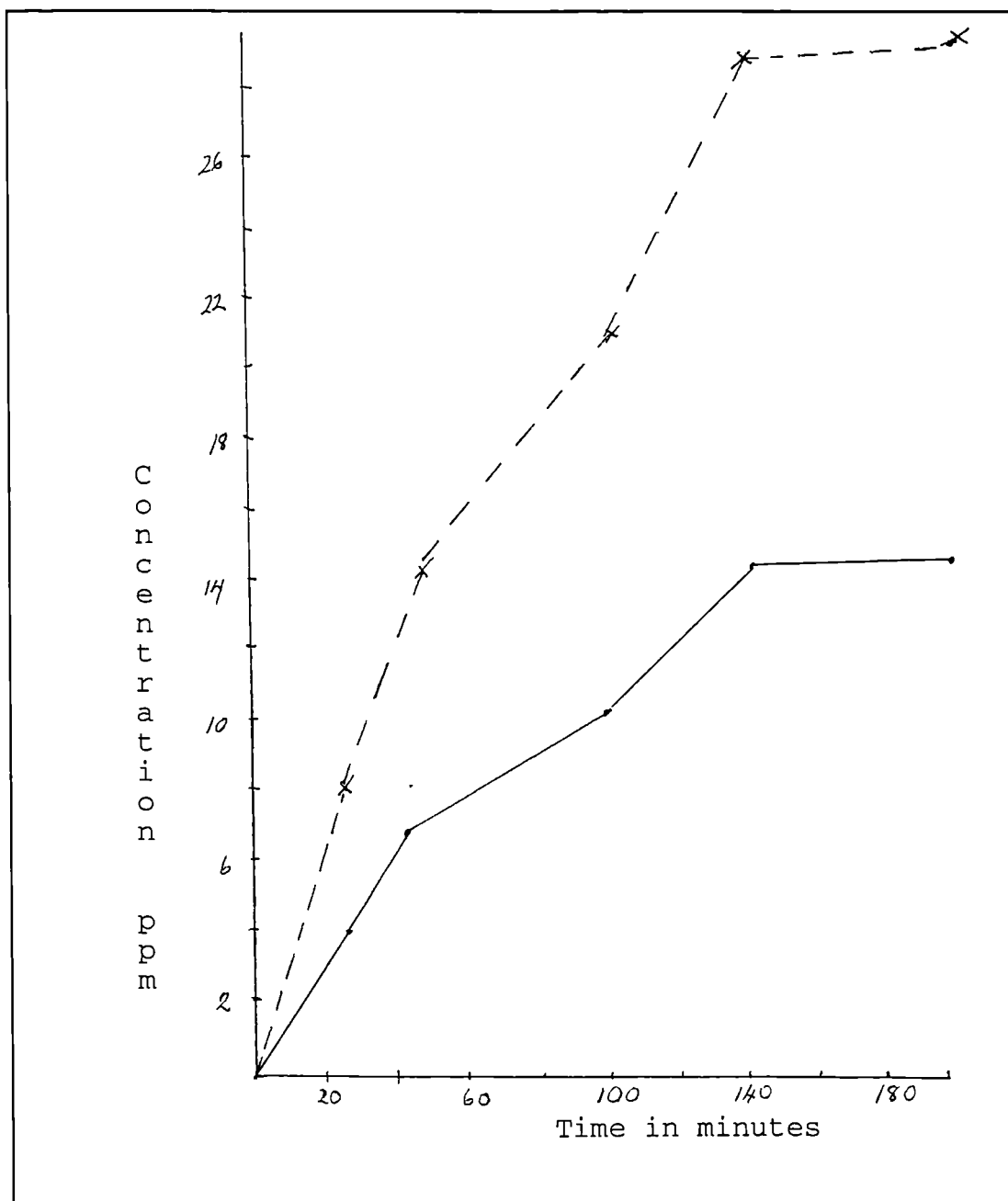
Figure 3:9 Graph of \text{H}_2\text{S} and \text{SO}_2 concentration against time. For the reaction of wool with 2.5 M \text{H}_3\text{PO}_2 under air in the presence of 0.5 g of hydroquinone. ( pH 1 and temperature 80^\circ\text{C} ). - - = \text{SO}_2 and — = \text{H}_2\text{S} .
