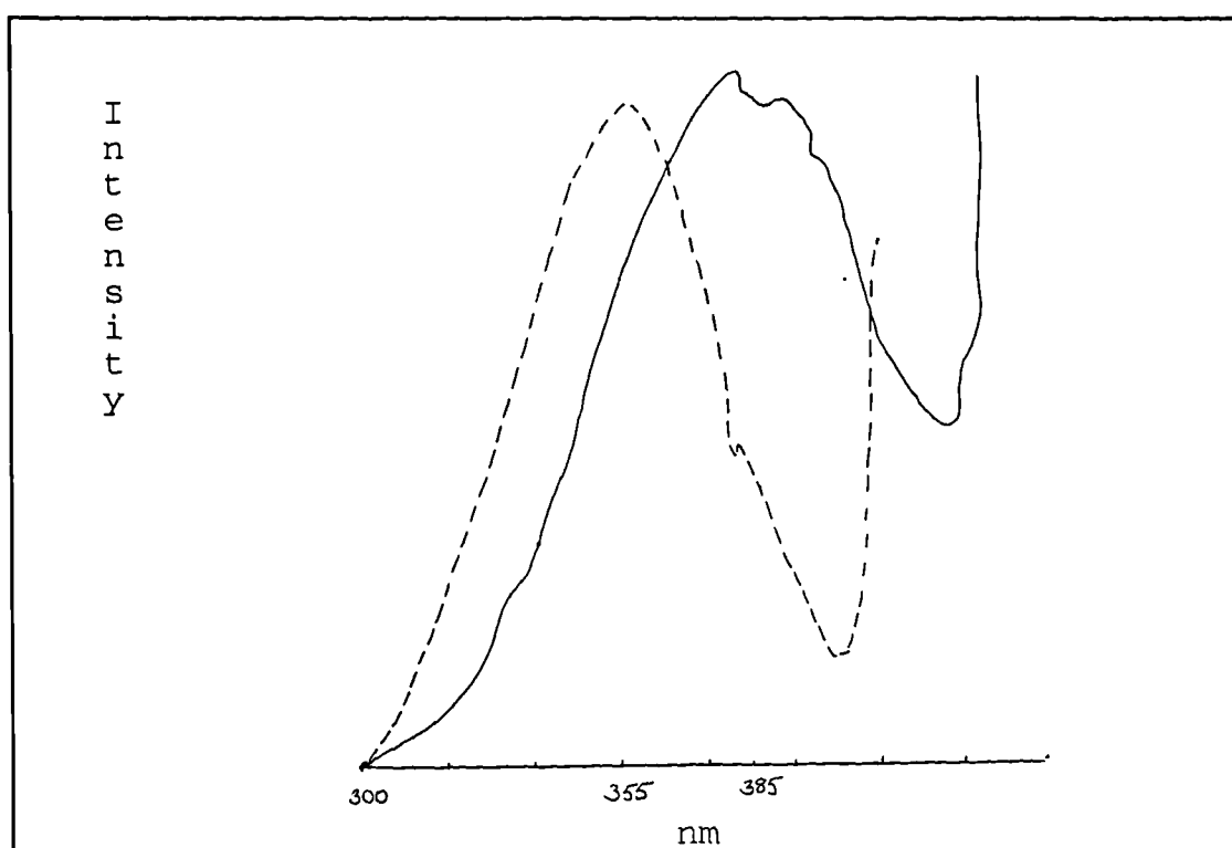
Figure 6:8 Fluorescence excitation spectrum of (a) - - acetic anhydride pretreated wool and (b) — untreated blank, excited at 450 nm.
