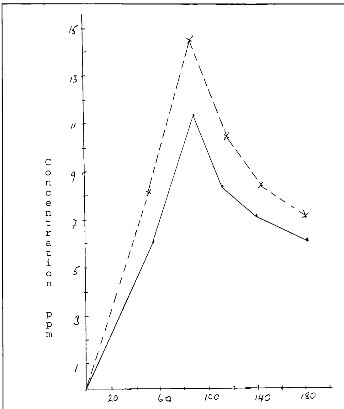
Figure 3:12 Graph of H 2 S and SO 2 concentration against time. For the reaction of cystine and 2.5 M H 3 PO 2 under N 2 . ( pH 1 and temperature 80°C ). - - = SO 2 and — = H 2 S.
