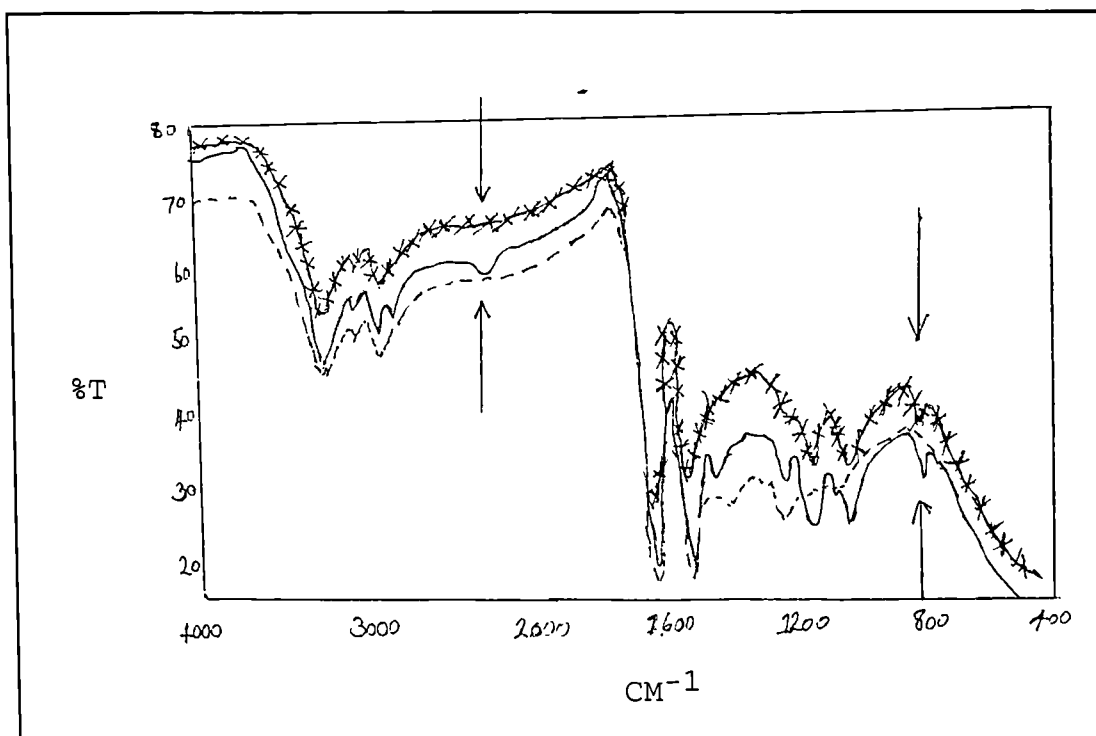
Figure 4:2 Surface I.R. spectra of wool, \text{H}_3\text{PO}_2 pretreated wool and \text{H}_3\text{PO}_2/\text{CH}_2\text{O} pretreated wool. - - = wool, — = \text{H}_3\text{PO}_2 wool and -*- = \text{H}_3\text{PO}_2/\text{CH}_2\text{O} wool
