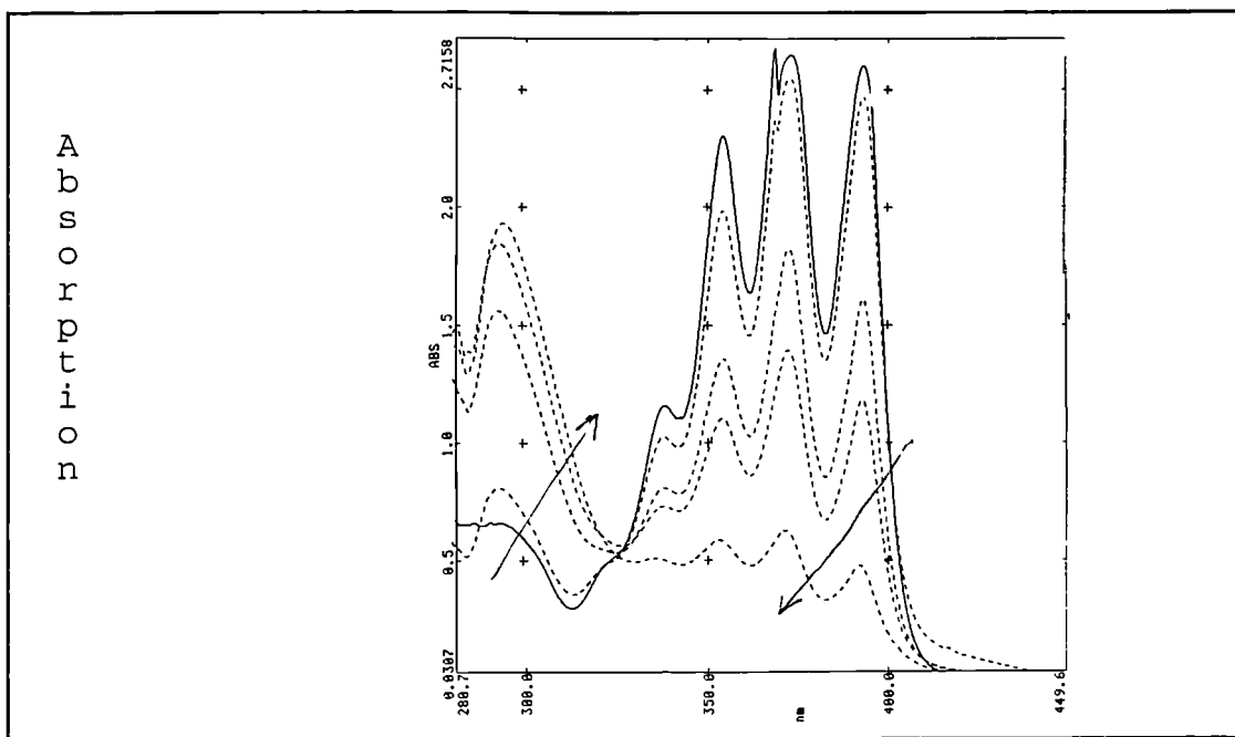
Figure 5:13 The UV spectrum of a 1 \times 10^{-3} M solution of product 1 ( benzylamino anthryl phosphonous acid ) in THF. On irradiation with black light at time intervals ( mins ) = 0, 25, 105, 135, 160.
