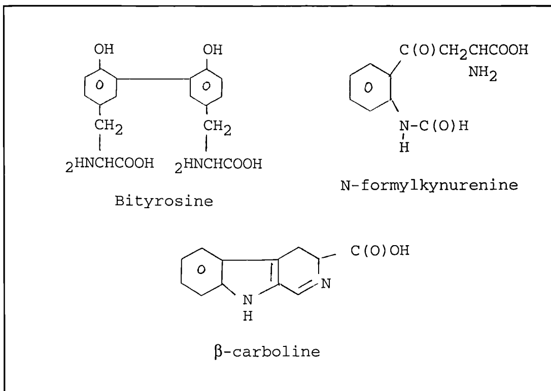
Figure 2:4 Species which have been suggested as responsible for the long wavelength fluorescence of wool.
