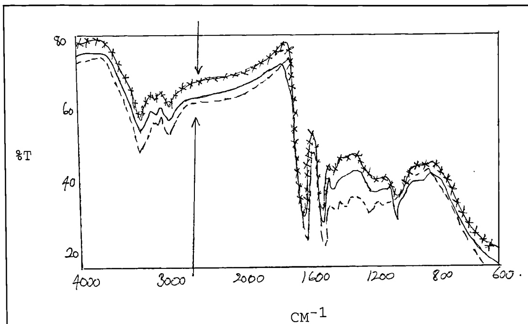
Figure 4:4 The surface I.R. spectra of wool, \text{H}_2\text{SO}_4 pretreated wool and \text{H}_2\text{SO}_4/\text{CH}_2\text{O} pretreated wool. - - = wool, — = \text{H}_2\text{SO}_4 wool and -*- = \text{H}_2\text{SO}_4/\text{CH}_2\text{O} wool.
