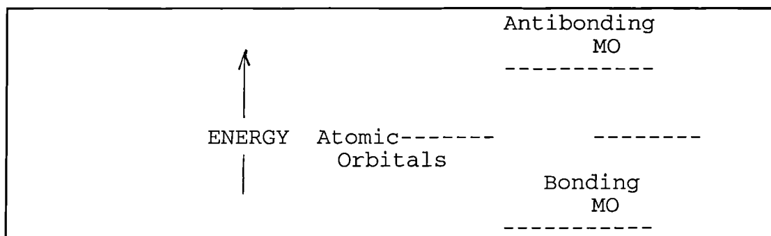
Figure 1:2 Effect on Orbital Energy of a Linear Combination of Atomic Orbitals
