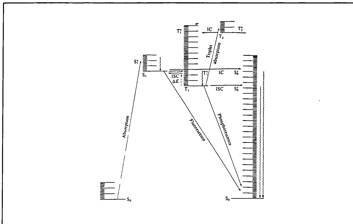
Figure 1:4 A Jablonski Diagram
