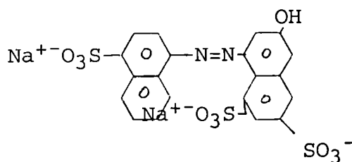
C.I. Acid Red 18
