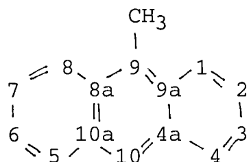
9-Methylanthracene
