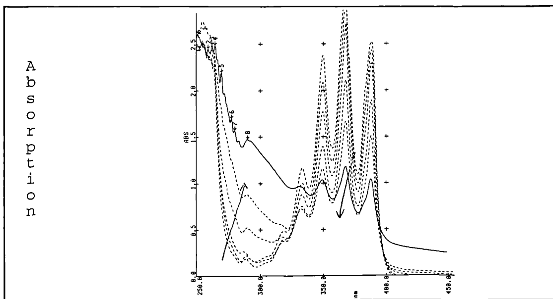
Figure 5:12 The UV spectrum of a 1 \times 10^{-3} M solution of 9-methylanthracene in THF. On irradiation with black light at time intervals ( mins ) = 0, 5, 15, 30, 45, 75.
