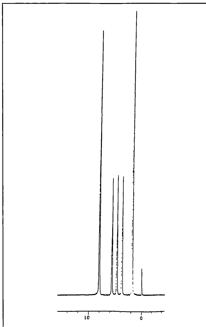
Figure 3:2 ^{31}\text{P} N.M.R. spectrum of \text{H}_3\text{PO}_3 in \text{D}_2\text{O} after 24 hours. Reference 85% \text{H}_3\text{PO}_4 .
