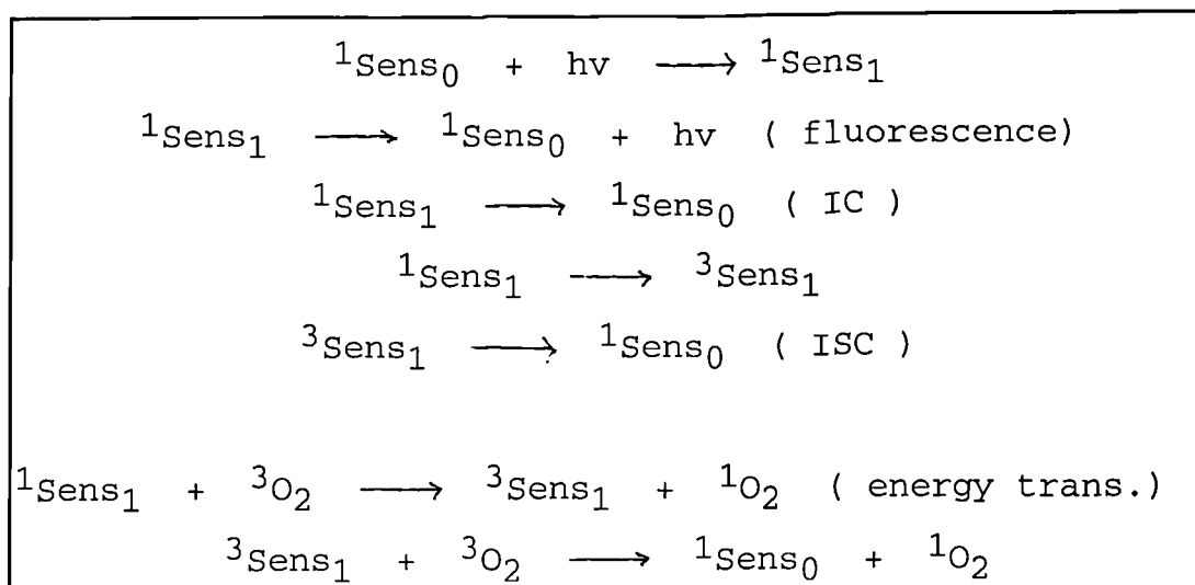
Figure 1:6 Possible transitions involved in the photosensitised production of singlet excited oxygen.
