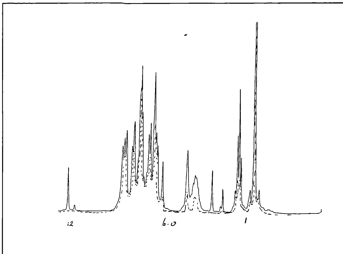
Figure 5:14 Proton N.M.R. spectra of (a) — product 1 and (b) - - - product 1 with D 2 O after 24 hrs. Solvent CDCl 3 , reference T.M.S.
