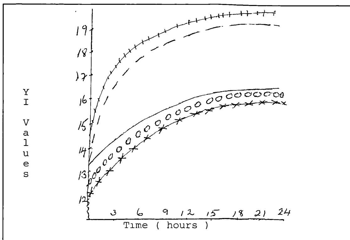
Figure 6:12 Graph of YI (E3I3) values against time ( hours ) of irradiation. For (a) — wool, (b) ++++ Phenyl isocyanate pretreated wool, (c) - - - Ethyl isocyanate pretreated wool, (d) o o o Phenyl isocyanate bisulphite pretreated wool, (e) * * Ethyl isocyanate pretreated wool.
