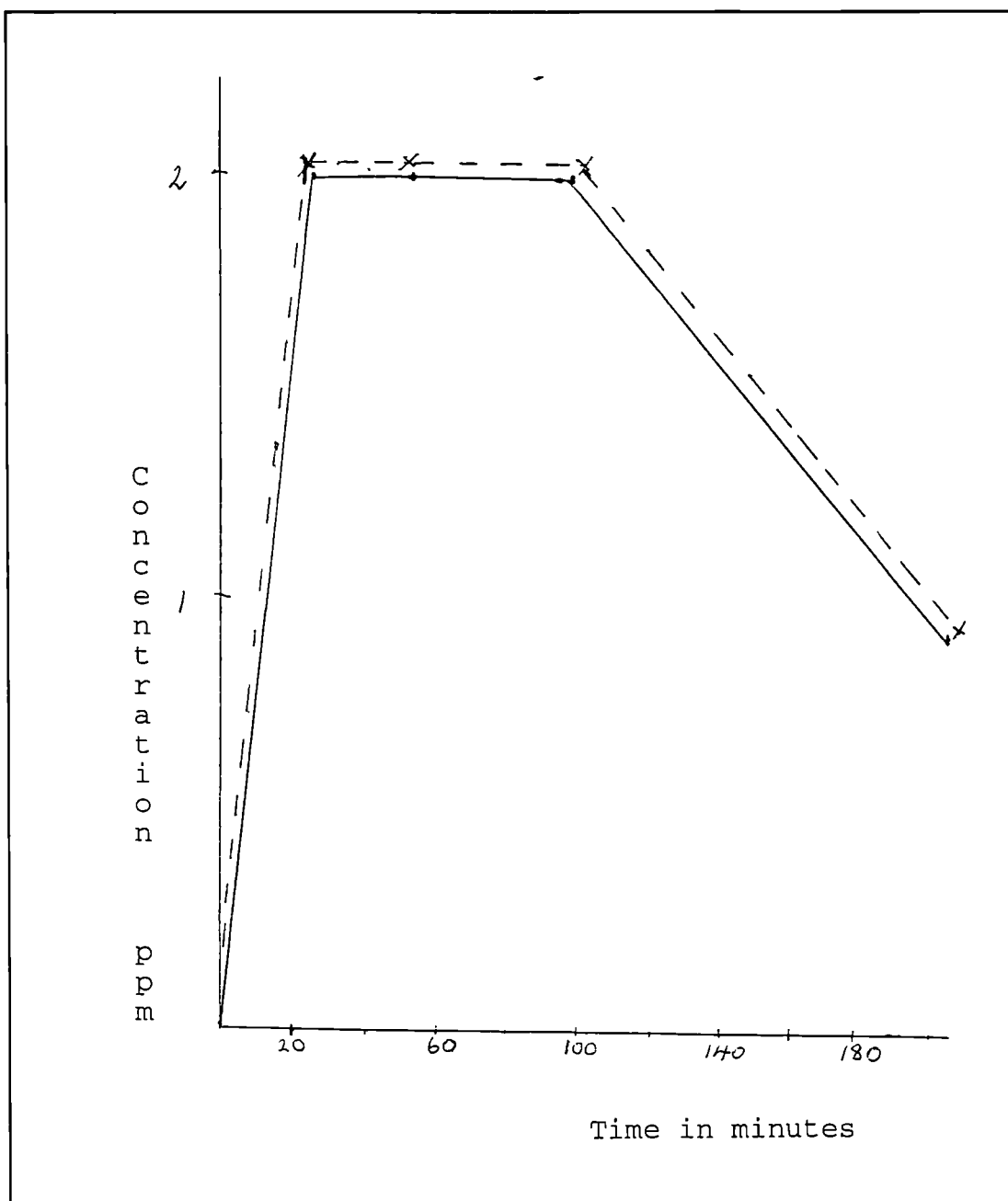
Figure 3:8 Graph of H 2 S and SO 2 concentration against time. For the reaction of cystine with 2.5 M H 3 PO 3 under air. ( pH 1 and temperature 80°C ). - - = SO 2 and — = H 2 S.
