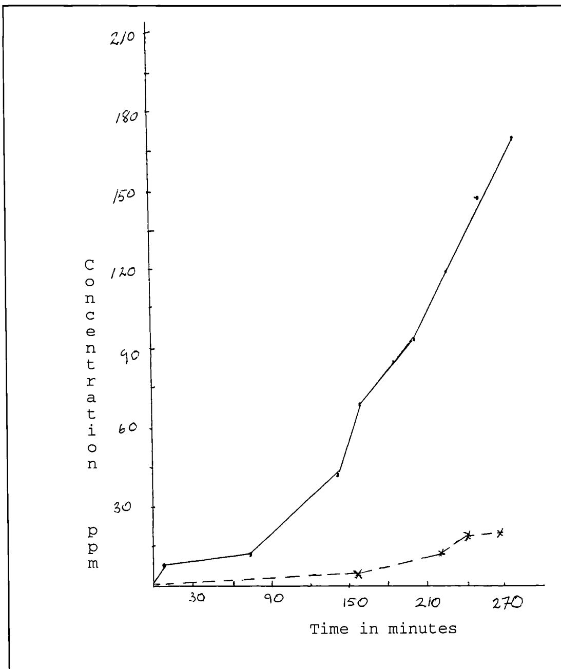
Figure 3:7 Graph of H 2 S and SO 2 concentration against time. For the reaction of cystine with 2.5 M H 3 PO 2 under air. ( pH1 and temperature 80°C ). - - = SO 2 and — = H 2 S.
