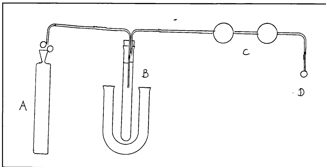
Figure 3:3 A schematic representation of the experimental system used for \text{H}_2\text{S} and \text{SO}_2 determination.
