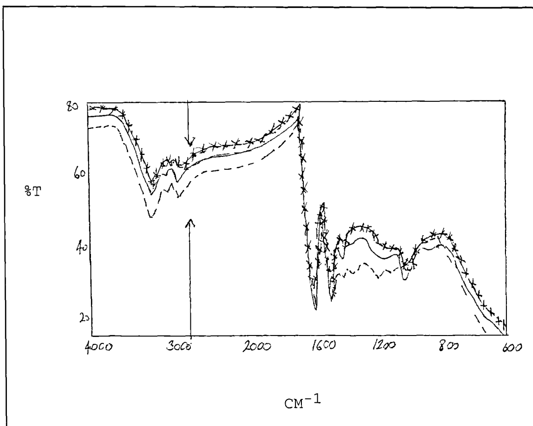
Figure 4:3 Surface I.R. spectra of wool, \text{H}_3\text{PO}_3 pretreated wool and \text{H}_3\text{PO}_3/\text{CH}_2\text{O} pretreated wool. - - = wool, — = \text{H}_3\text{PO}_3 wool and -*- = \text{H}_3\text{PO}_3/\text{CH}_2\text{O} wool.
