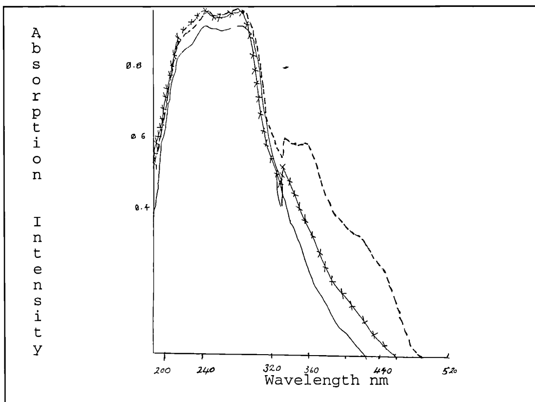
Figure 3:15 Diffuse reflectance spectra of wool, wool + 9-BMA and \text{H}_3\text{PO}_2 pretreated wool + 9-BMA.
