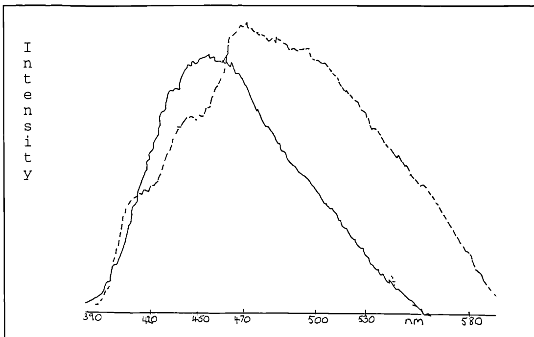
Figure 3:14 Fluorescence emission spectra of \text{H}_3\text{PO}_2 treated wool and blank alkali wool, both treated with 9-bromomethylacridine. Excitation wavelength at 380 nm and sensitivity of 100/0. — = Wool + BMA, - - - = \text{H}_3\text{PO}_2 wool + BMA.
