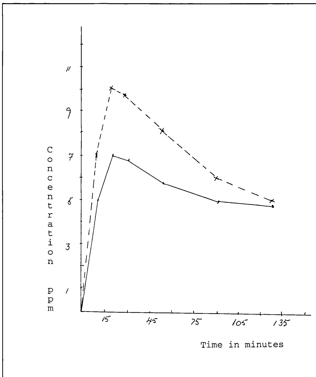
Figure 3:10 Graph of H 2 S and SO 2 concentration against time. For the reaction of 2-hydroxyethyl disulphide and 2.5 M H 3 PO 2 under air. ( pH 1 and temperature 80°C ). - - = SO 2 and — = H 2 S.
