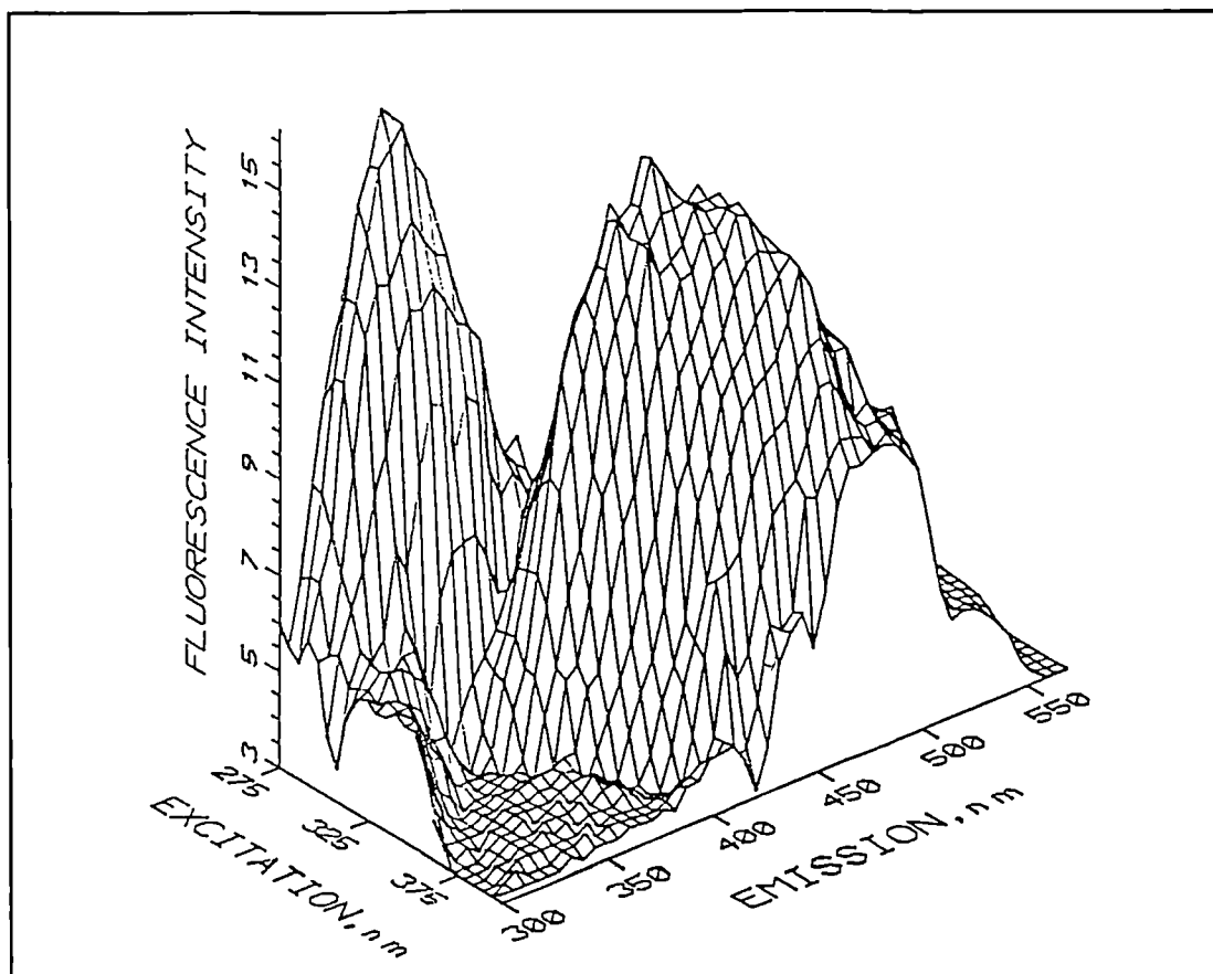
Figure 2:3 3D Plot of Fluorescence Intensity from Wool in Excitation-Emission Space.
