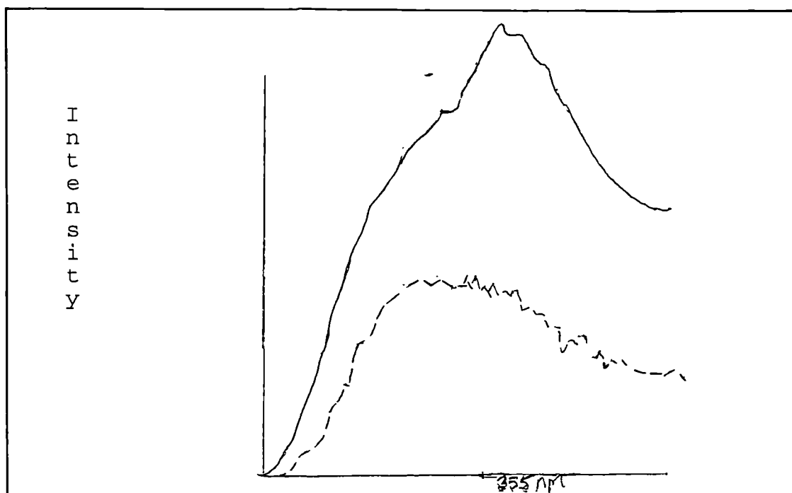
Figure 6:11 Fluorescence emission intensity of (a) --- untreated wool and (b) — phenyl isocyanate pretreated wool, excited at 280 nm. Sensitivity of (a) 100, of (b) 30.2. Slit width 4.
