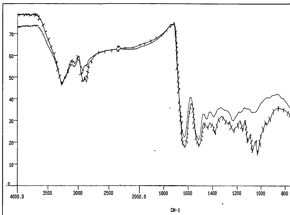
Figure 6:1 Surface I.R. spectrum of (a) \longrightarrow blank wool and (b) ++++ LP3 pretreated wool.
