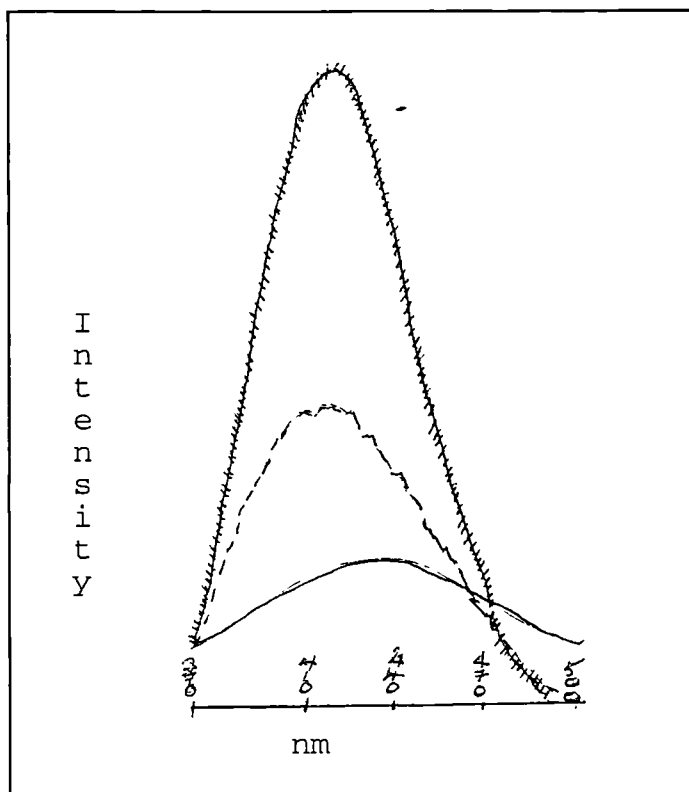
Figure 8:5 The fluorescence emission spectrum of a) — blank wool treated with OPA and EA, b) - - - H 3 PO 2 reduced wool treated with OPA and EA, and c) ++++ tributylphosphine reduced wool treated with OPA and EA. Excited at 350 nm, slit width 4, sensitivity 30/0.
