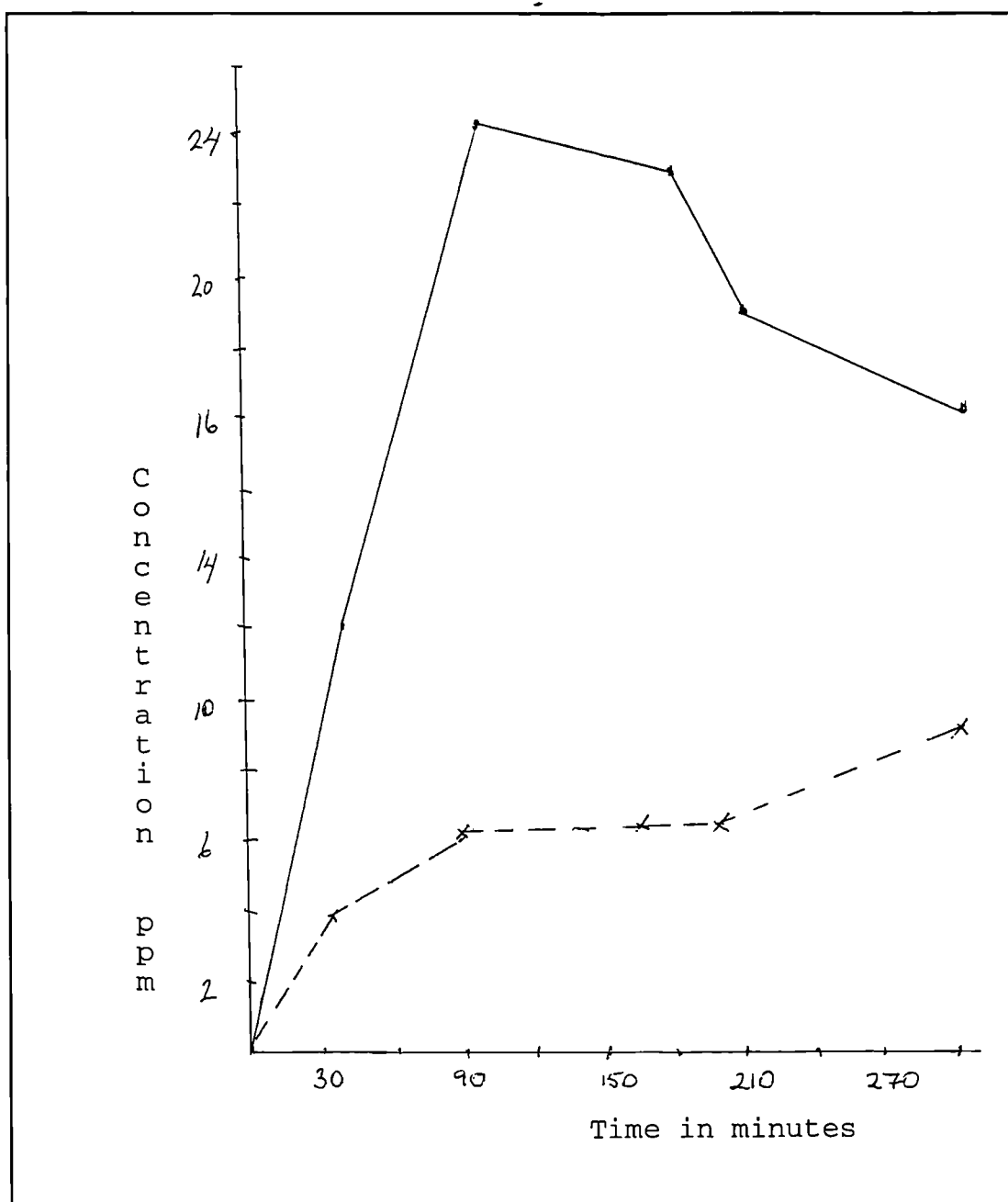
Figure 3:13 Graph of H 2 S and SO 2 concentration against time. For reaction of H 2 O 2 bleached wool with 2.5 M H 3 PO 2 under air. ( pH 1 and temperature 80°C ). - - = SO 2 and — = H 2 S.
