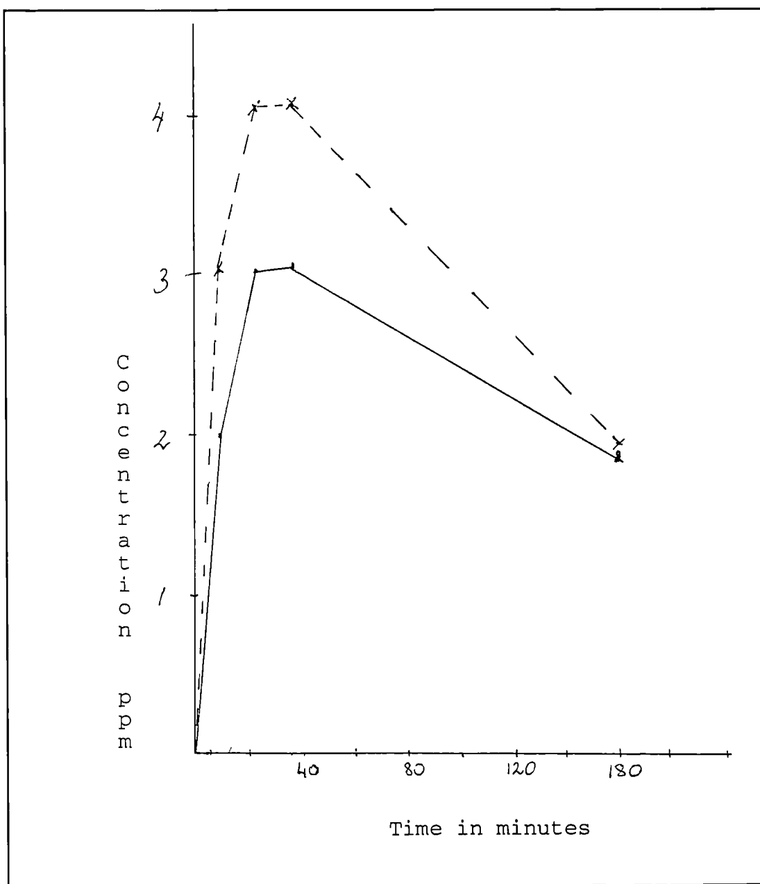
Figure 3:6 Graph of H 2 S and SO 2 concentration against time. For the reaction of 2.5 M H 3 PO 3 and wool under air. ( pH1 and at 80°C ). - - = SO 2 and — = H 2 S.
