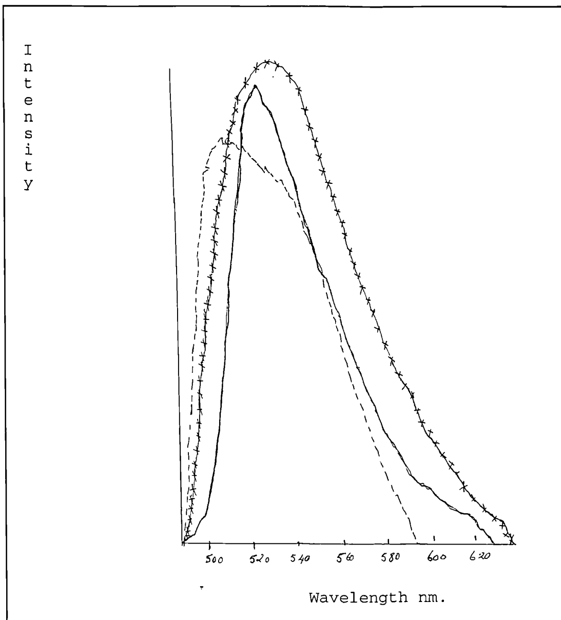
Figure 3:16 Fluorescence emission spectra of alkali treated wool ( blank ), \text{H}_3\text{PO}_2 and \text{H}_3\text{PO}_3 pretreated samples on reaction with 5-IAF. At excitation wavelength 480 nm and sensitivity 3/5. — = alkali treated wool, -*- = \text{H}_3\text{PO}_3 pretreated wool and - - - = \text{H}_3\text{PO}_2 pretreated wool.
