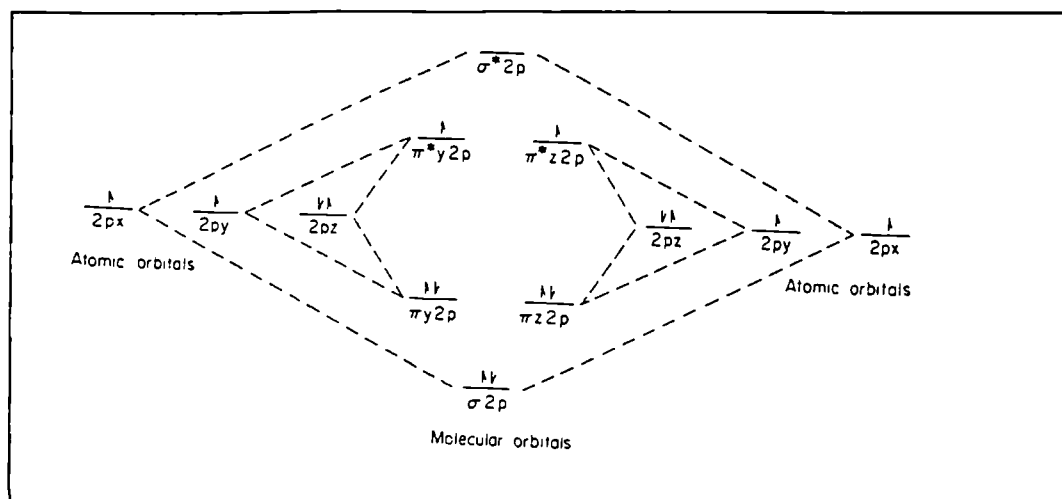
Figure 1:5 Orbital representation of molecular oxygen triplet.
