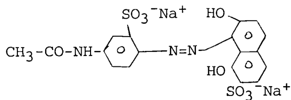
C.I. Acid Red 37
