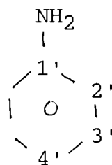
Aniline
