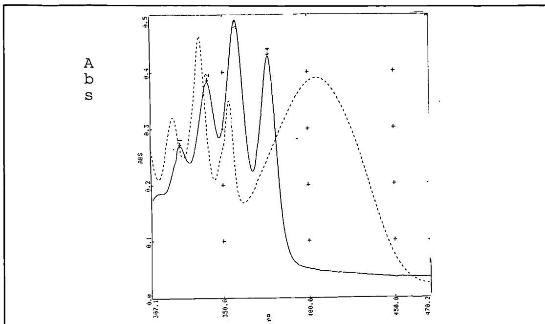
Figure 5:6 The U.V. spectra of 2-aminoanthracene (a) - - - in alkali ( NaOH ) and (b) ——— in acid ( trifluoroacetic acid ) solvent methanol.
