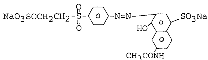
C.I. Reactive Orange 16
