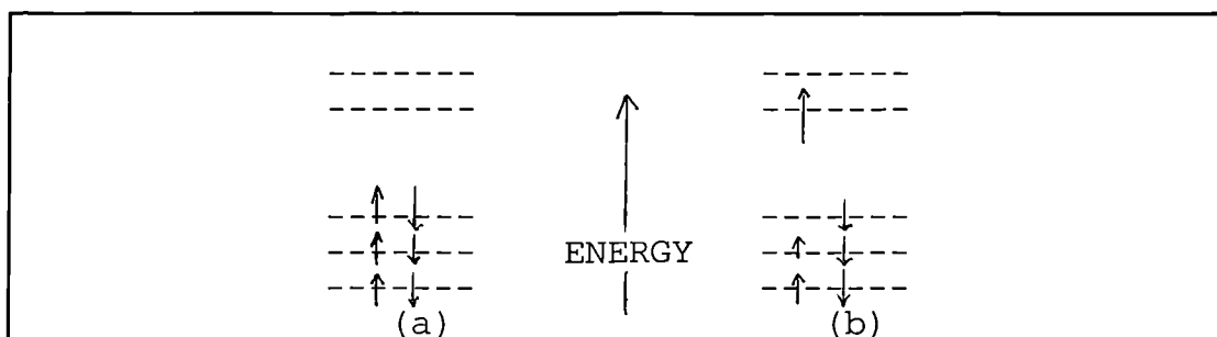
Figure 1:1 Molecular orbital diagram for an organic molecule, showing some of the orbitals and their occupancy in (a) the ground state and in (b) an electronically excited state.
