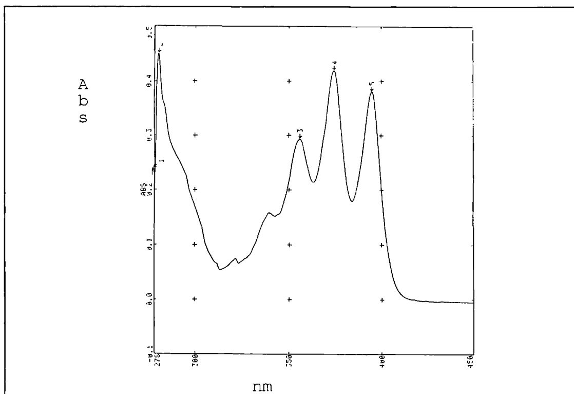
Figure 5:4 U.V. spectrum of product ( \alpha -phenylamino anthryl phosphonous acid ), solvent toluene.
