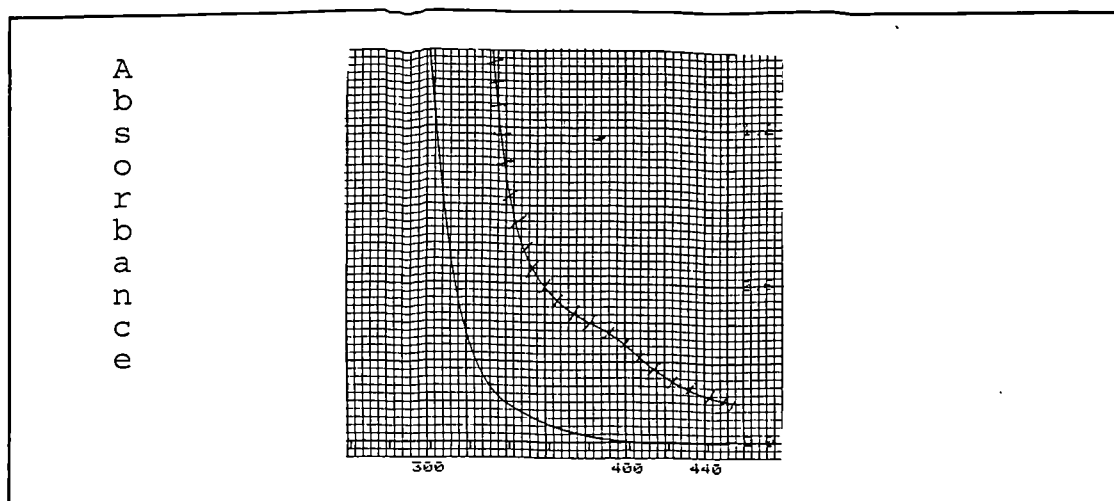
Figure 6:4 UV spectrum of (a) — solution of Z-LP3 in DMF, and (b) ++++ solution of Z-LP3 in DMF, irradiated for 24 hours.
