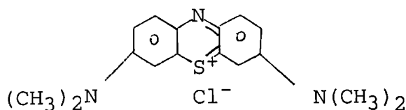
C.I. Methylene Blue
