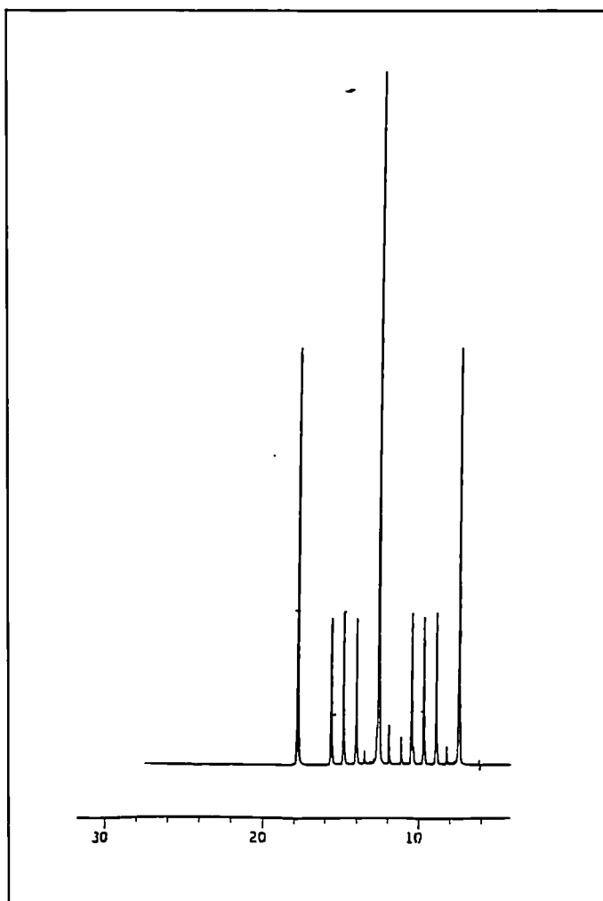
Figure 3:1 ^{31}\text{P} N.M.R. spectrum of \text{H}_3\text{PO}_2 in 50% \text{D}_2\text{O} after 24 hours. Reference 85% \text{H}_3\text{PO}_4 .
