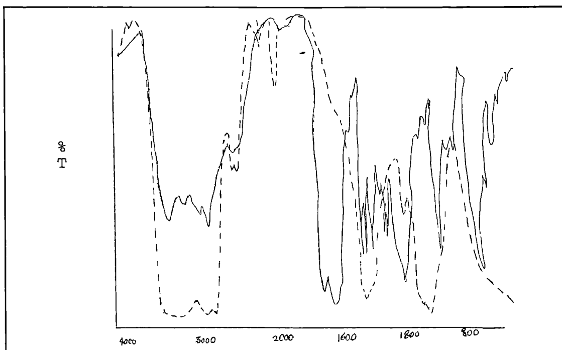
Figure 8:4 IR spectrum ( liquid in \text{H}_2\text{O} ) of a) — OPA and cysteine red solution and b) - - - same solution reacted with \text{NaBH}_4 .
