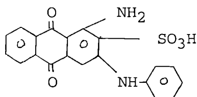
C.I. Acid Blue 62
