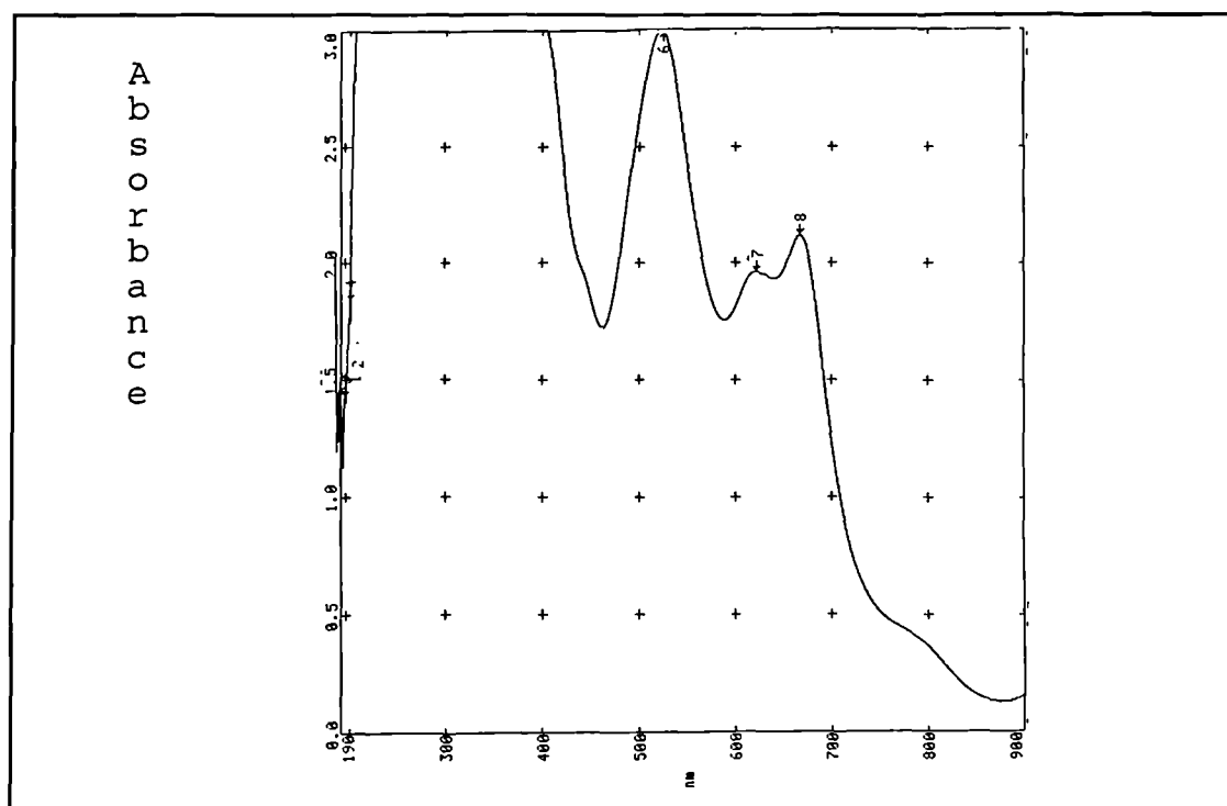
Figure 8:2 UV spectrum of compound formed after addition of a molar excess of dodecylamine to an equimolar solution of OPA and cysteine.
