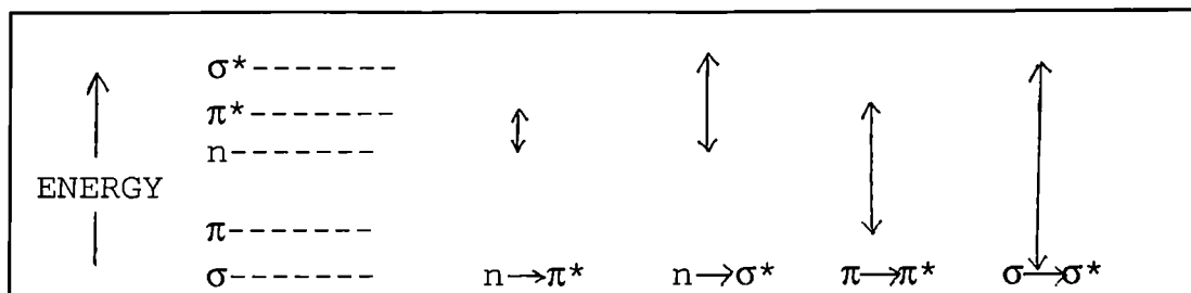
Figure 1:3 Some possible transition types of organic molecules.
