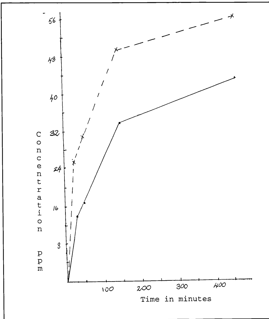
Figure 3:5 Graph of H 2 S and SO 2 concentration against time. For the reaction of wool with 2.5 M solution of H 3 PO 2 , ( pH 1 and at 80°C ), under air. - - = SO 2 and — = H 2 S.
