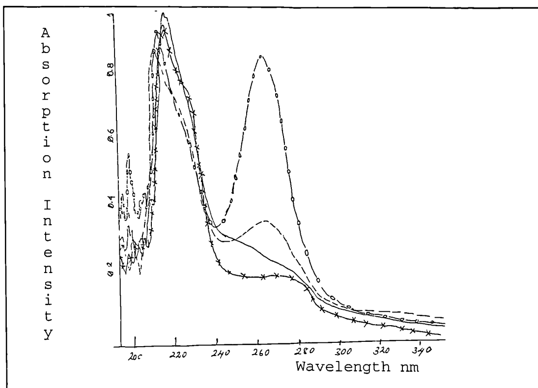
Figure 3:18 Absorption Spectra of 2-PEC. For blank hydrolysed wool, \text{H}_3\text{PO}_3 treated wool, \text{H}_3\text{PO}_2 treated wool and tributylphosphine treated wool. Solvent 6 N HCl. — = blank, -*-* = \text{H}_3\text{PO}_3 wool, - - = \text{H}_3\text{PO}_2 wool and -o-o- = tributylphosphine wool.
