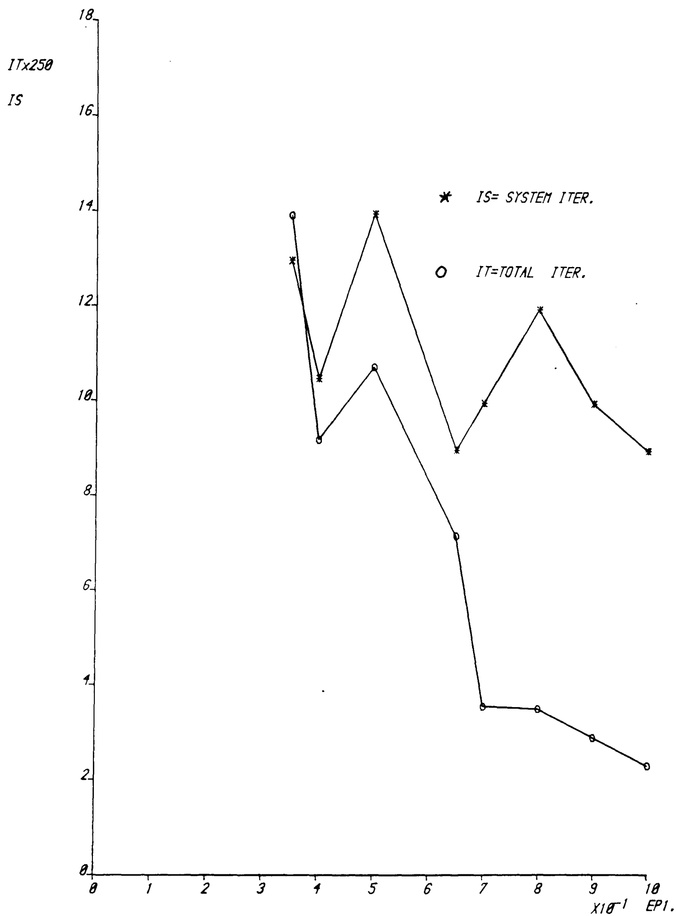
FIGURE(4.10) SENSITIVITY OF DIPCM(V.2),EX. 1
