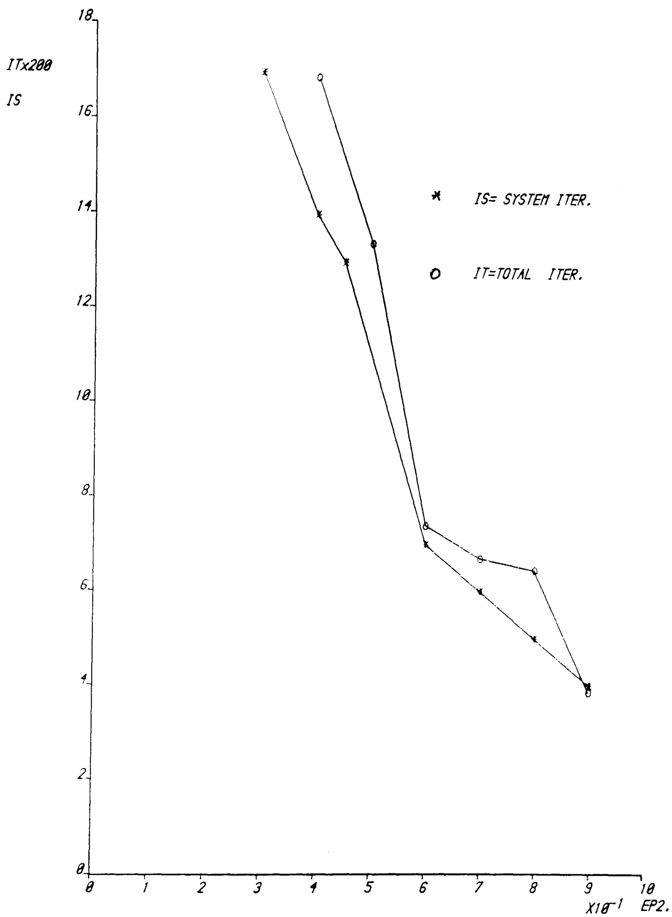
FIGURE(4.11) SENSITIVITY OF DIPC(V.2), EX. 1
