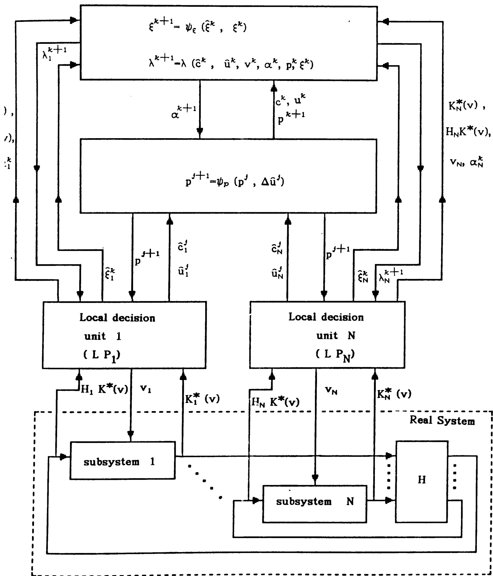
Figure ( 6. 5) Information Structure of the DIA (ISOPE).
