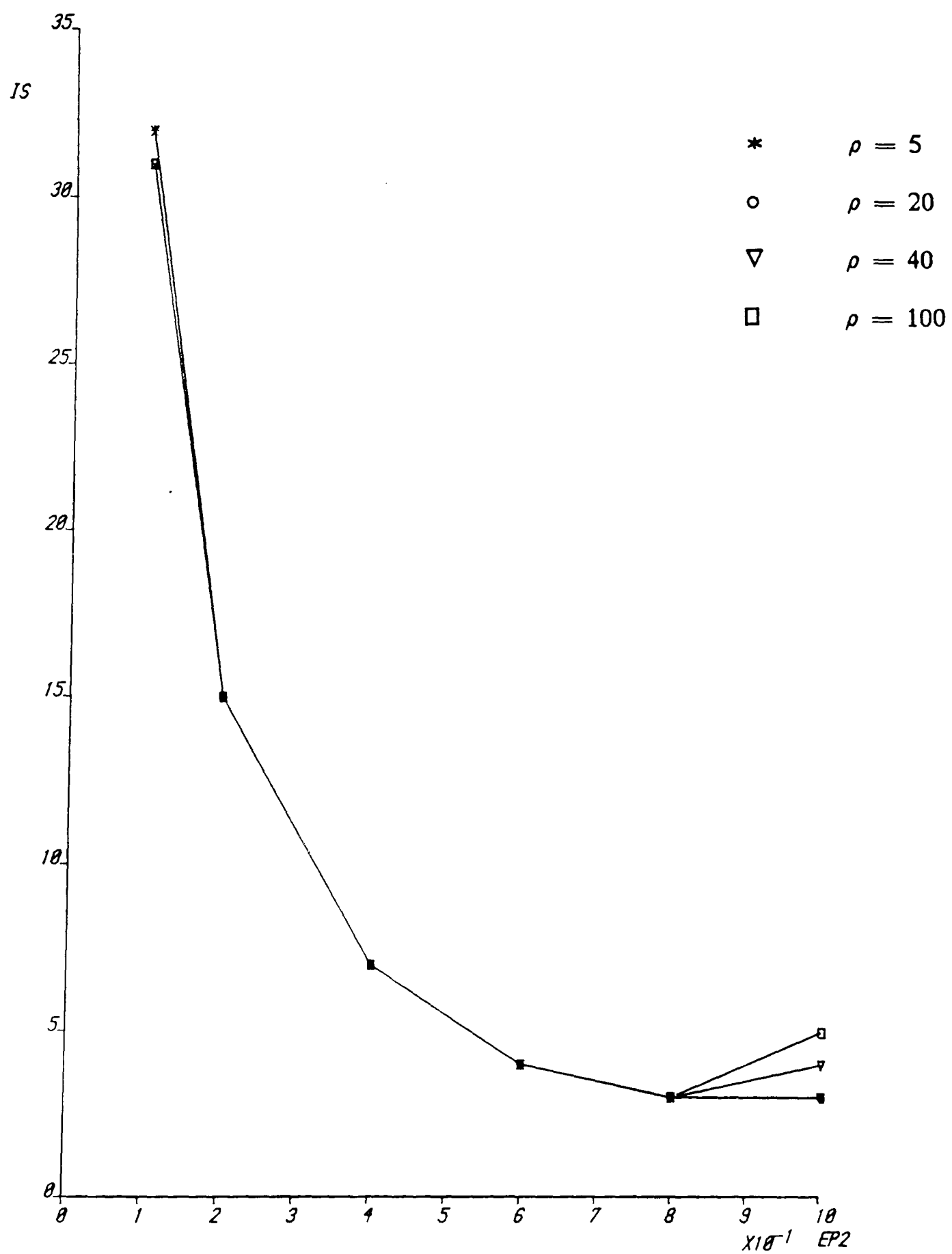
FIGURE(5.3) SENSITIVITY OF ALGORITHM TO EP2 ( \epsilon_2 ), EX. 2
