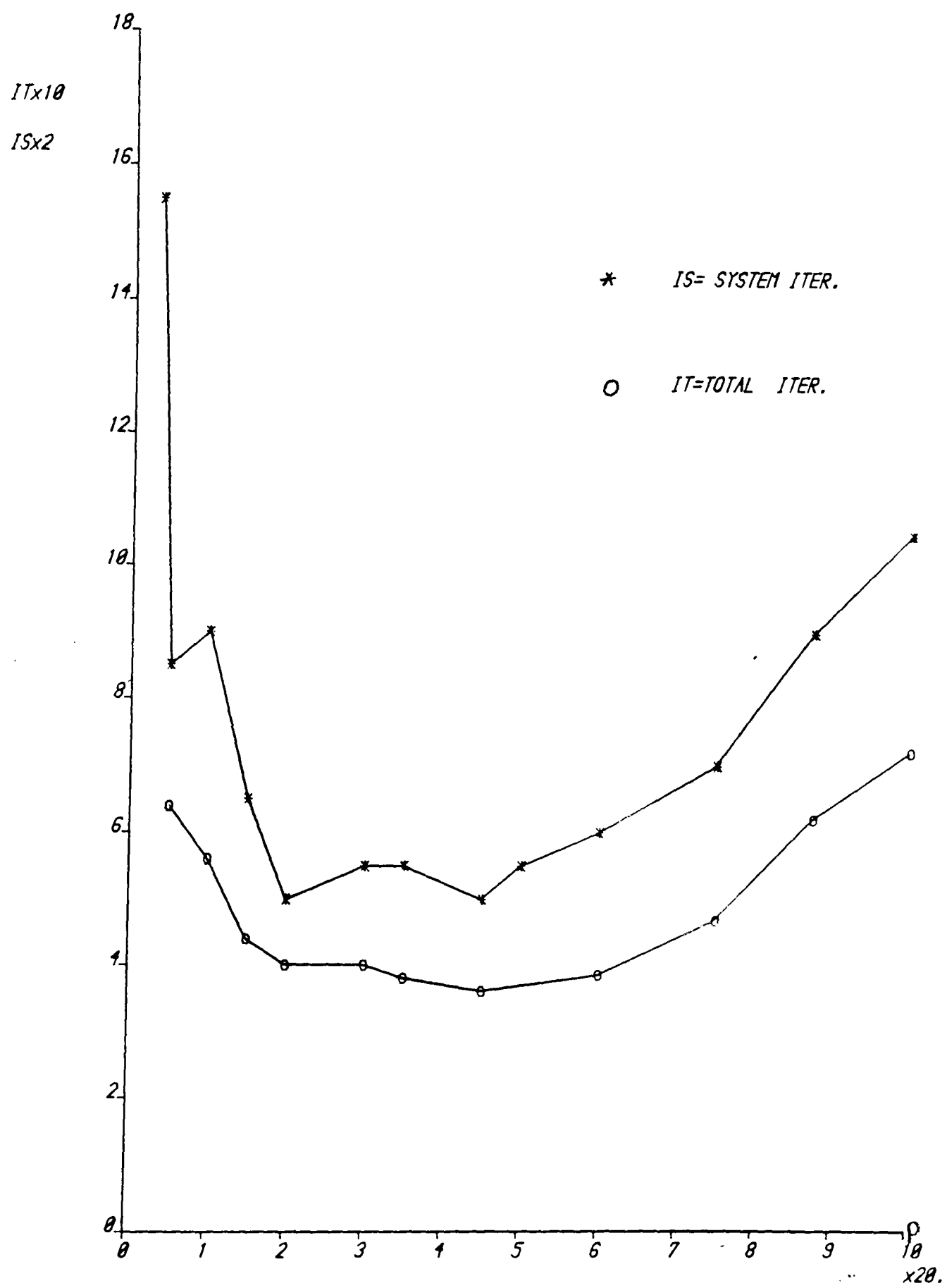
FIGURE(4.14) SENSITIVITY OF THE AIMF, EX. 1
