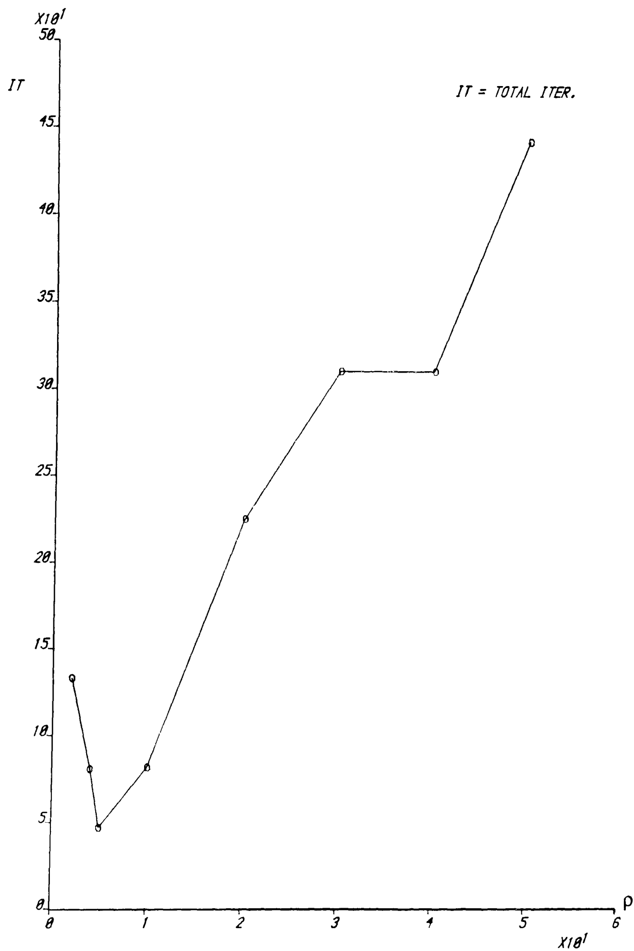
FIGURE(5.6) EFFECT OF PENALTY COEFFICIENT ON CONVERGENCE OF IT, EX. 1
