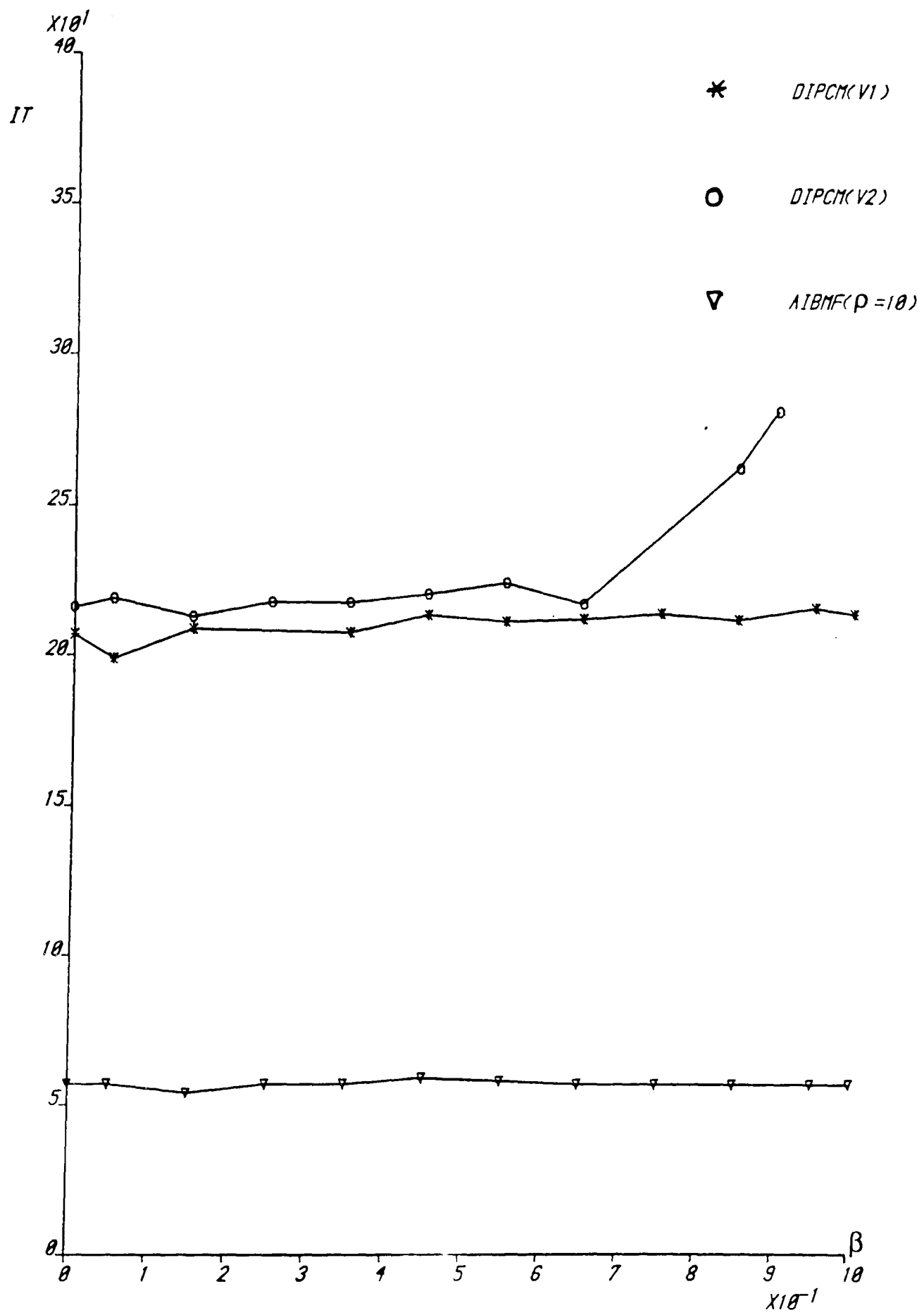
FIGURE(4.16) EFFECT OF NONLINEARITY ON TOTAL ITER. FOR DIPCM(V1,V2) AND THE AIBMF(EX.3)
