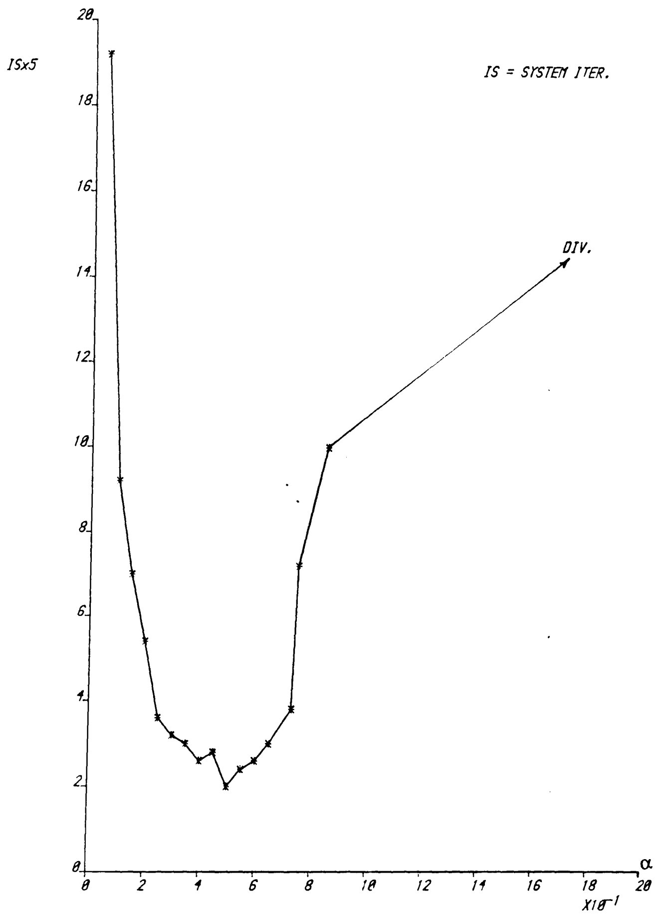
FIGURE(4.12) EFFECT OF \alpha ON IS FOR p=10 , EX. 1
