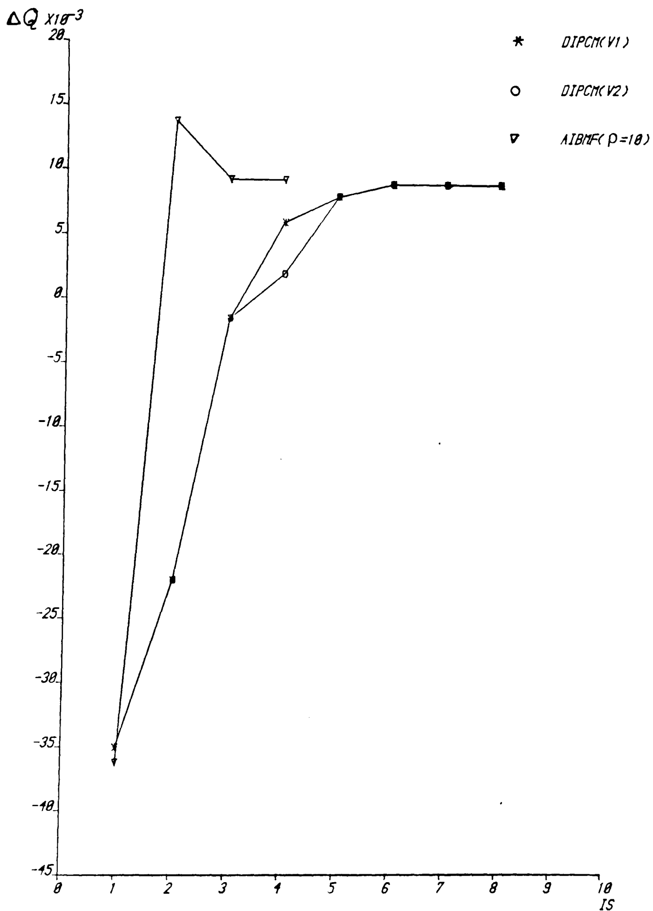
FIGURE(4.17) CONVERGENCE OF ALGORITHMS FOR EXAMPLE 3.
