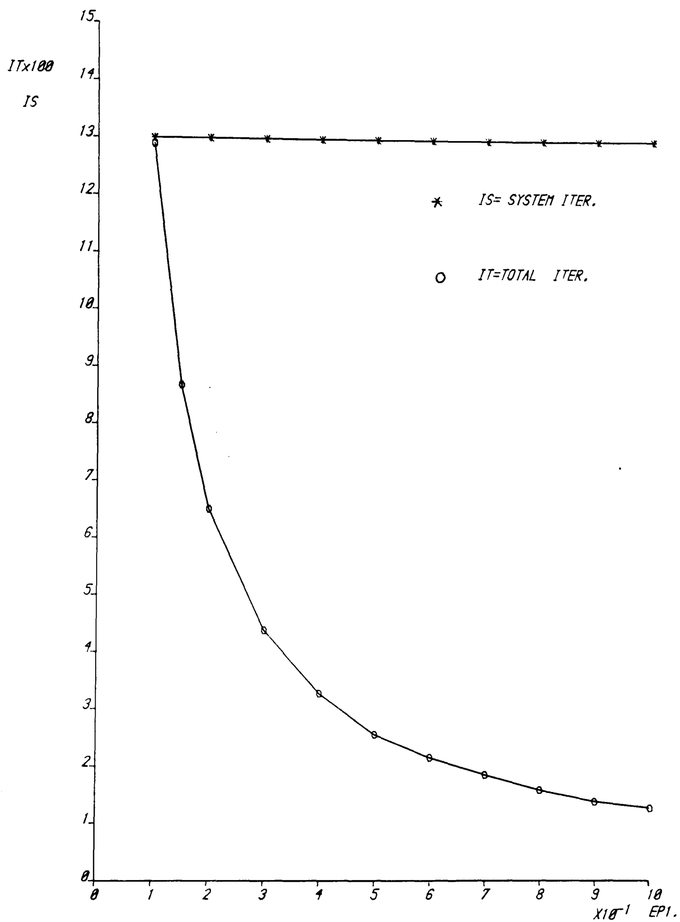
FIGURE(4.8) SENSITIVITY OF DIPCM(V.1),EXAMPLE 1
