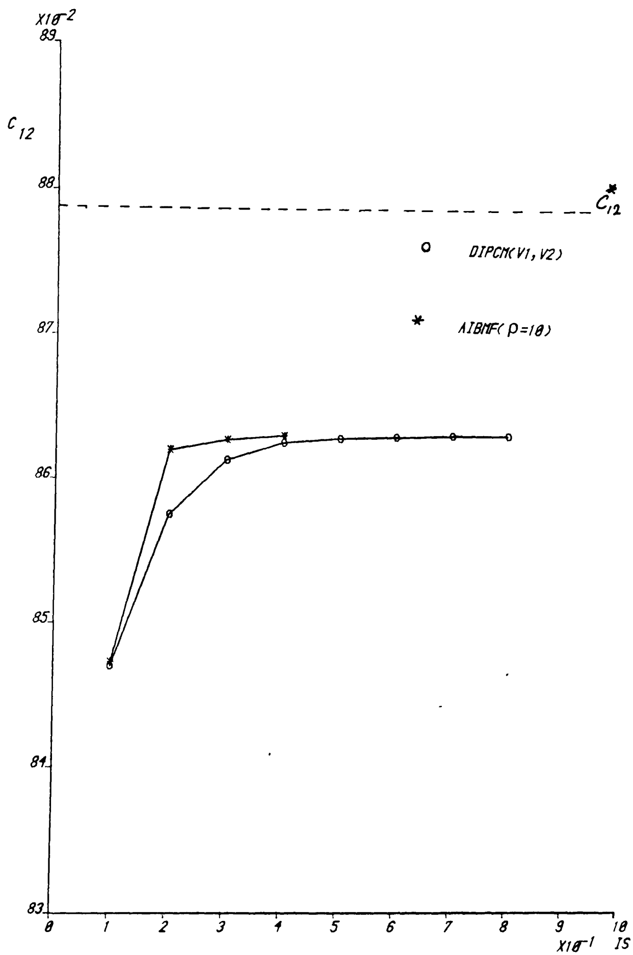
FIGURE(4.19) CONVERGENCE OF SET POINT C_{12} , EX. 3
