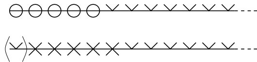
FIGURE 3. The weight diagram x_\emptyset for \delta = 2m or 2m + 1 with m = 5 or m = -5
