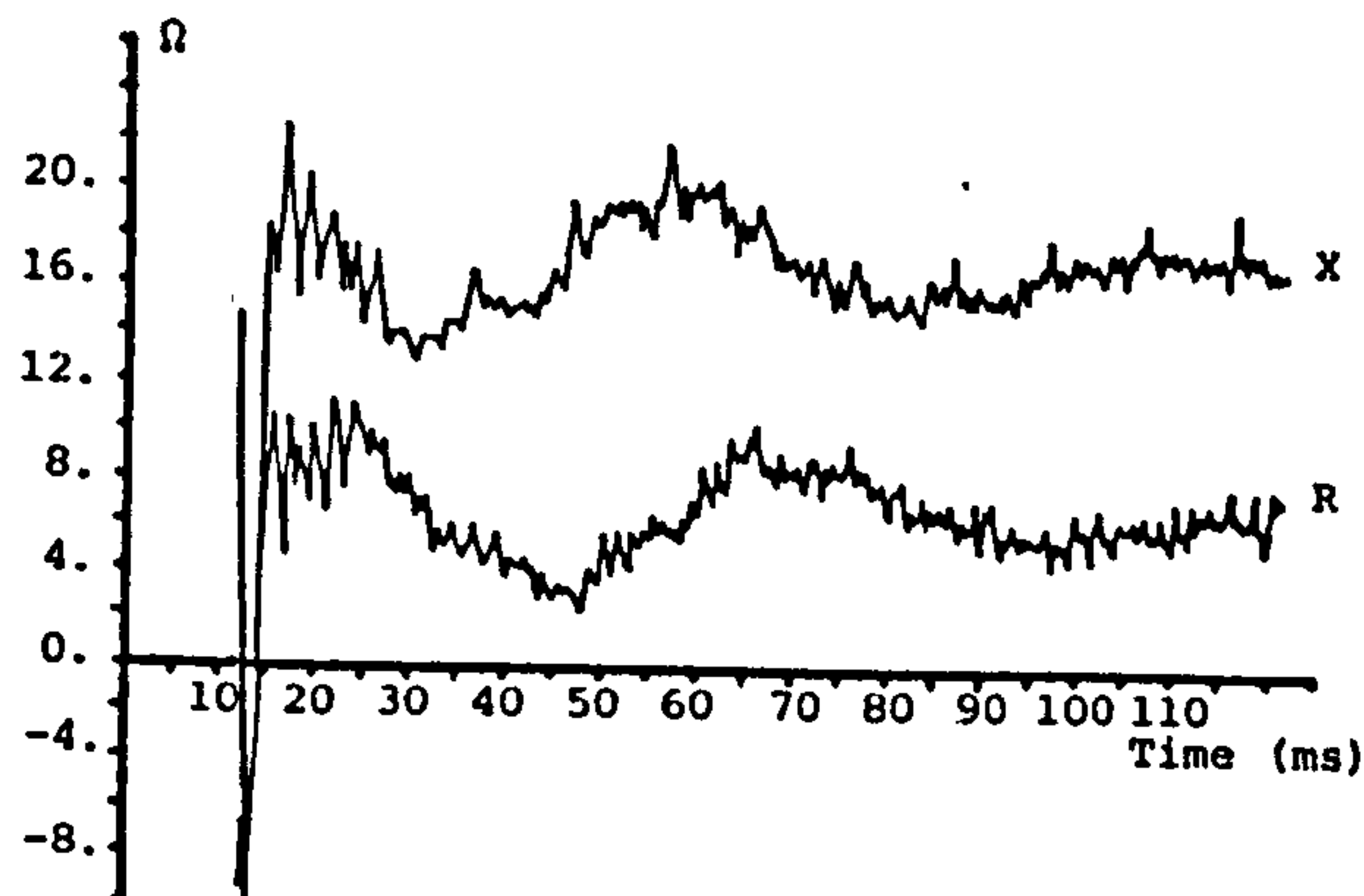
Fig 6 Effect of Subsynchronous Resonance.
