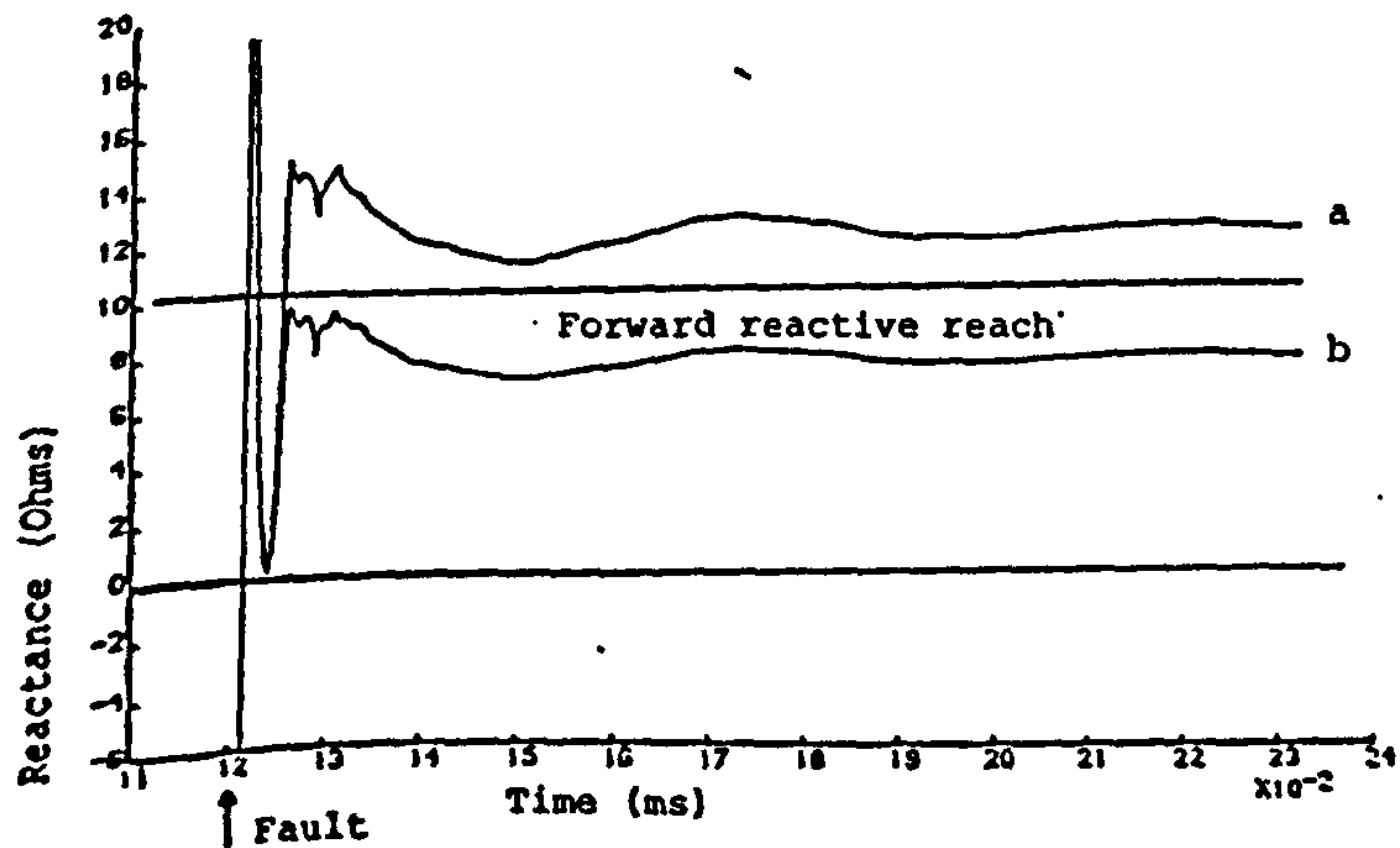
Fig 4. Measured reactance vs time
