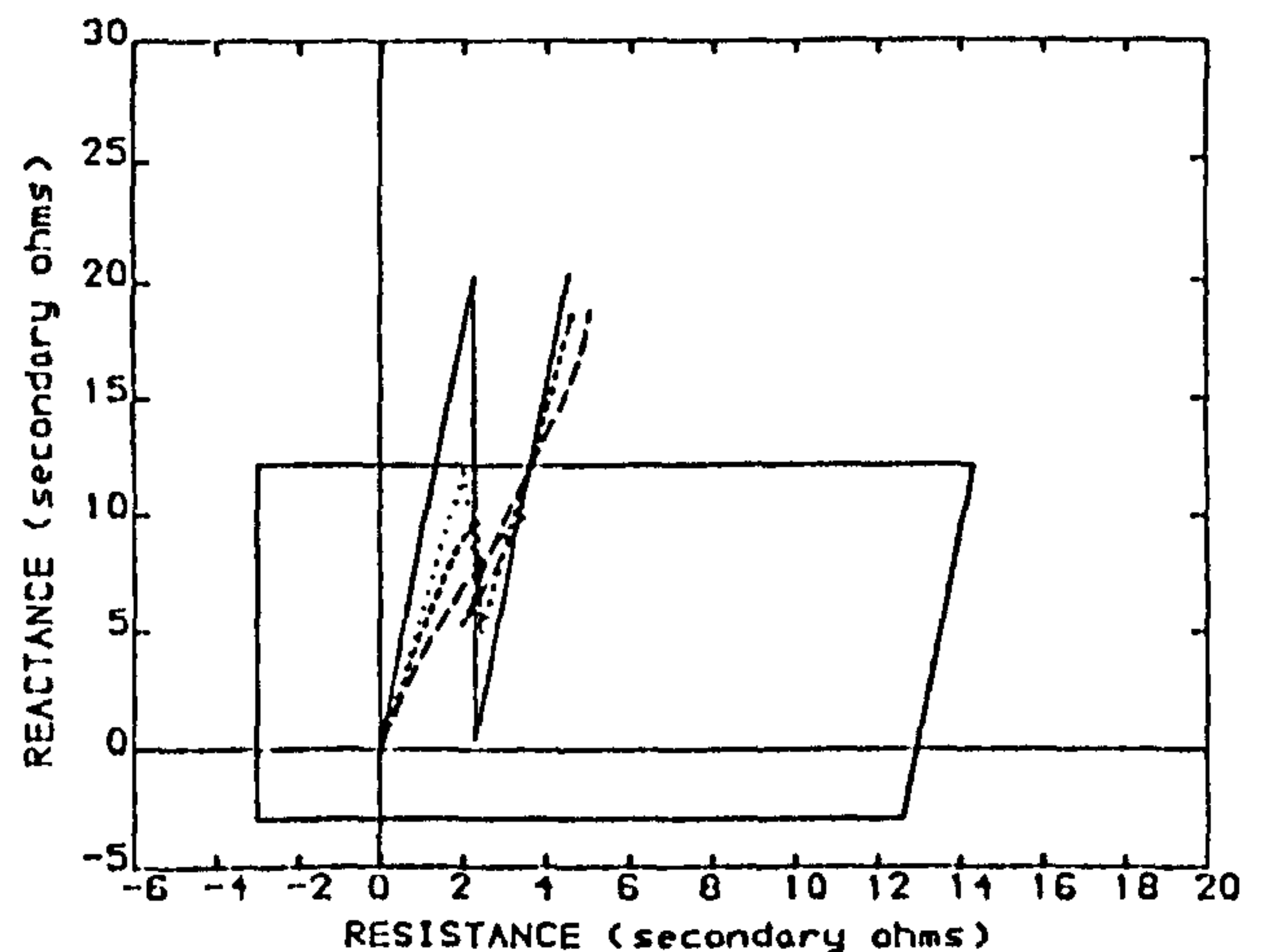
Fig 8: Quadrilateral Trip Characteristic And Measured Impedances With NRCF ( K(\alpha)=2.015 \angle 4.5^\circ )
