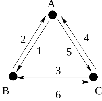
Theory (a)
