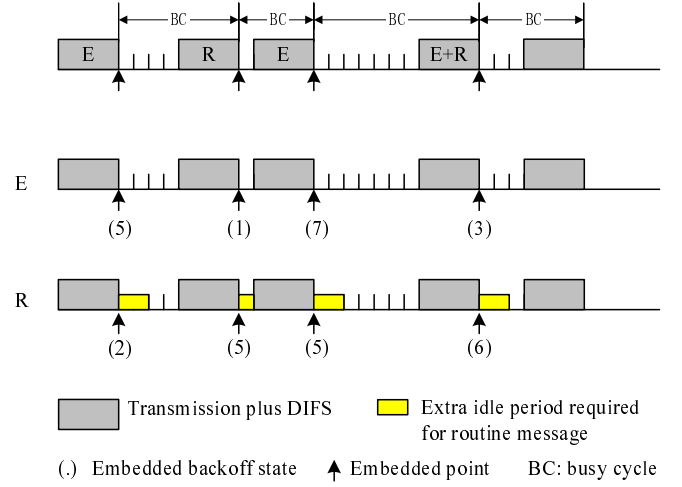
Fig. 4. A simple illustration of embedded state.
