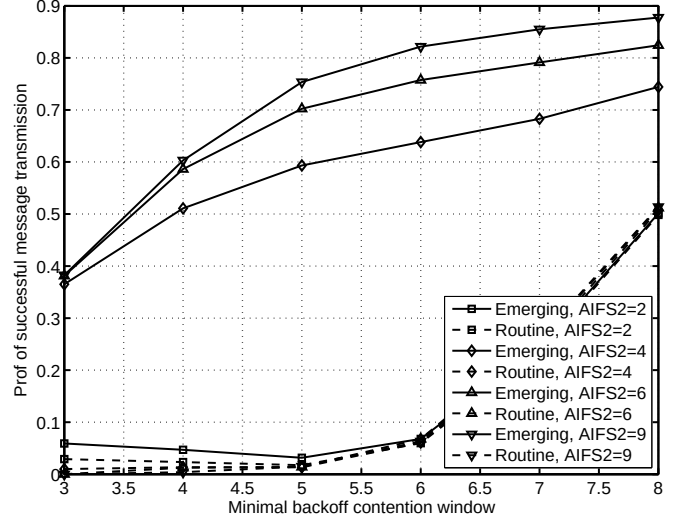
Fig. 12. Successful message delivery rate of emerging and routine applications versus \log_2(W_e) for emerging applications. N_e = 5 , L_d = 100 bytes, R_t = 1 Mbps, V_d=0.1 , R_t = 110 m.
