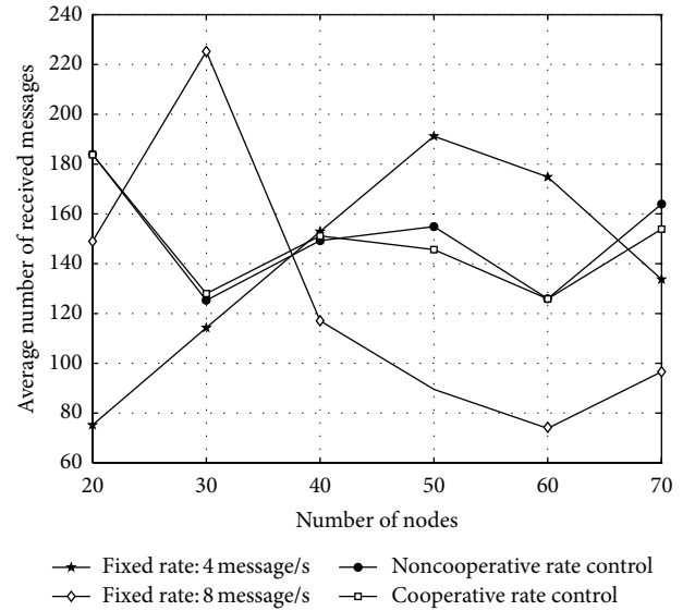
FIGURE 6: Average number of successfully received messages per second.
