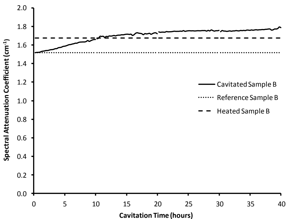
Figure 14: Graph of the Spectral Extinction Coefficient ( \text{cm}^{-1} ) of: (a) Cavitated Sample B, (b) Reference Sample B, and (c) Heated Sample B, as a Function of Cavitation Time (hours).
