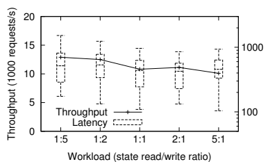
Figure 5: Throughput and latency with different read/write ratios (online collaborative filtering)
