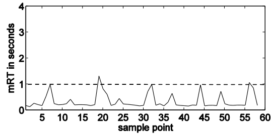
Figure 16. MIMO-UB requests mRT.
