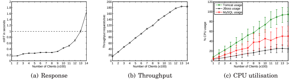
Fig. 3. System identification results. Error bars in Figure 3(a) correspond to a 95% confidence interval (CI) around the mean and in Figure 3(c) they show \pm one standard deviation ( \sigma ) around the mean.
