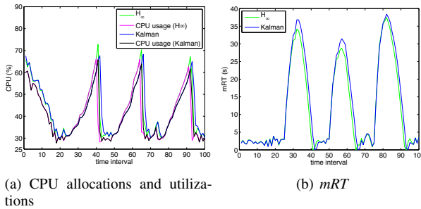
Fig. 6. Saw-Tooth Workload Changes: \mathcal{H}_\infty controller performance when the process ( w_k ) and the measurement ( v_k ) noise are normally distributed.
