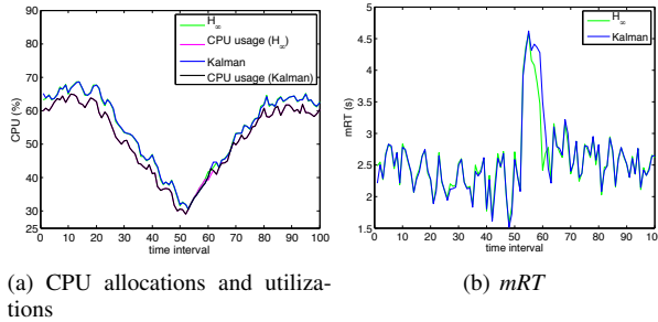
Fig. 5. Gradual Workload Changes: \mathcal{H}_\infty controller performance when the process ( w_k ) and the measurement ( v_k ) noise are uniformly distributed.
