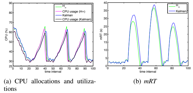
Fig. 7. Saw-Tooth Workload Changes: \mathcal{H}_\infty controller performance when the process ( w_k ) and the measurement ( v_k ) noise are uniformly distributed.
