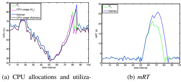
Fig. 4. Gradual Workload Changes: \mathcal{H}_\infty controller performance when the process ( w_k ) and the measurement ( v_k ) noise are normally distributed.
