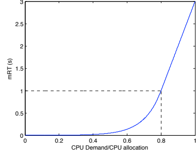
Fig. 3. mRT model with respect to CPU usage, where \gamma = 10 and \phi = 0.8 .
