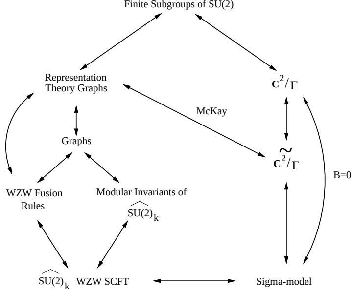
Figure 3: Web of Correspondences: Each finite group \Gamma \subset SU(2) gives rise to an isolated Gorenstein singularity as well as to its representation ring \mathcal{R} . The cohomology ring of the resolved manifold is isomorphic to \mathcal{R} . The \widehat{SU(2)}_k WZW theory at level k = \# \text{ Conjugacy classes of } \Gamma - 2 has a graphical representation of its modular invariants and its fusion ring. The resulting graph is precisely the non-affine version of McKay's graph for \Gamma . The WZW model arises as a subsector of the conformal field theory description of the quotient singularity when the B -field has been set to zero. We further note that the three rings in the picture are equivalent.
