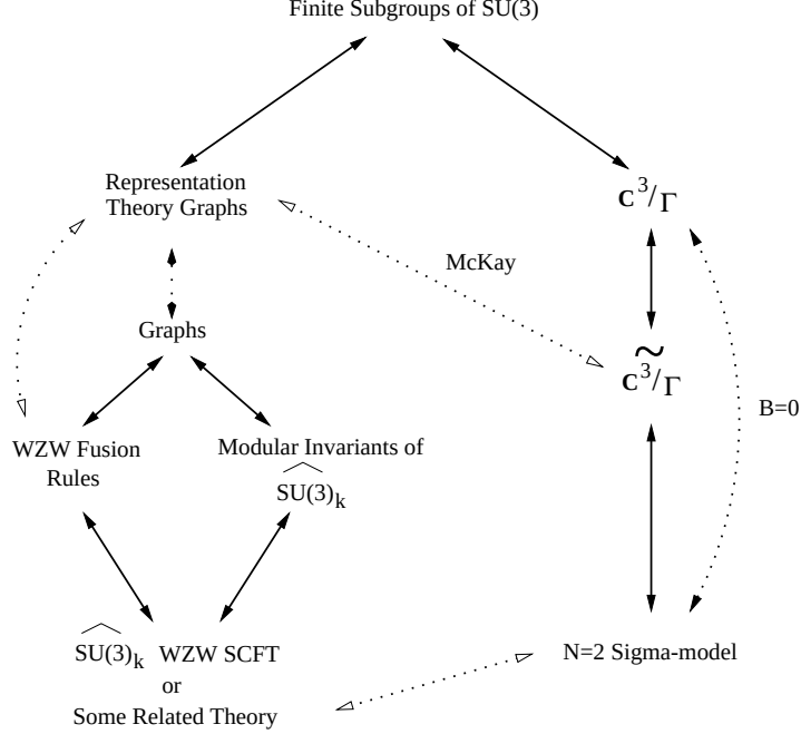
Figure 4: Web of Conjectures: Recently, the graphs from the representation theory side were constructed and were noted to resemble those on \widehat{SU(3)}_k side [1]. The solid lines have been sufficiently well-established while the dotted lines are either conjectural or ill-defined.
