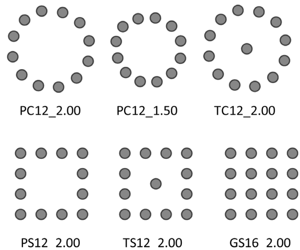
Fig. 11. Examples of pile group arrangements
