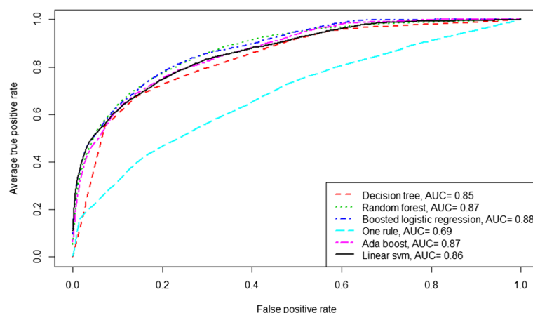
Figure 1 Receiver operating characteristic curves plotting performance of different statistical learning methods, averaging results from 50 bootstrap tests (out-of-bag predictions, dataset imputing mean/mode for missing values).
