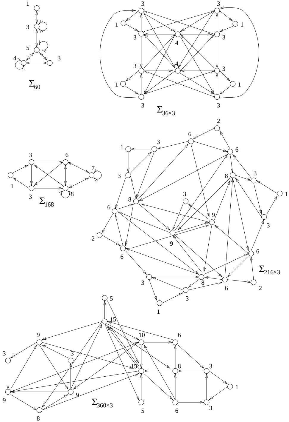
Figure 5: \Sigma \subset \text{full } SU(3) . Only \Sigma_{36 \times 3}, \Sigma_{216 \times 3}, \Sigma_{360 \times 3} belong only to the full SU(3) , for these we have the one loop \beta -function vanishing condition manifesting as the label of each node equaling to \frac{1}{3} of that of the incoming and outgoing neighbours respectively. The matrix representation for these graphs are given in Appendix IV.
