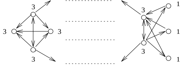
Figure 3: \Delta_{3n^2} \subset SU(3) for n \not\equiv 0 \pmod{3} . These belong to both the full and center-removed SU(3) .
