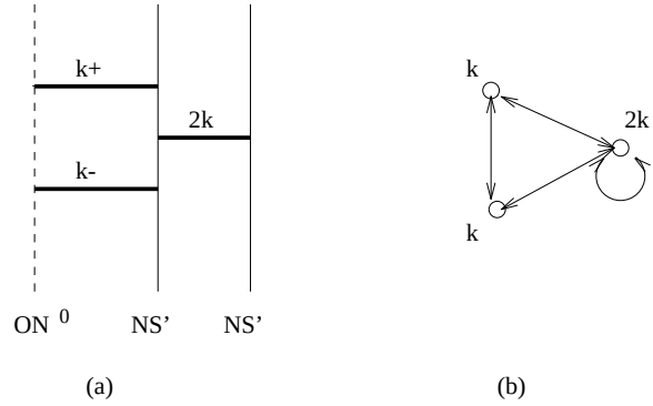
Figure 7: (a). The brane configuration of projection using NS5'-branes. (b). The quiver diagram for the brane configuration in (a).
