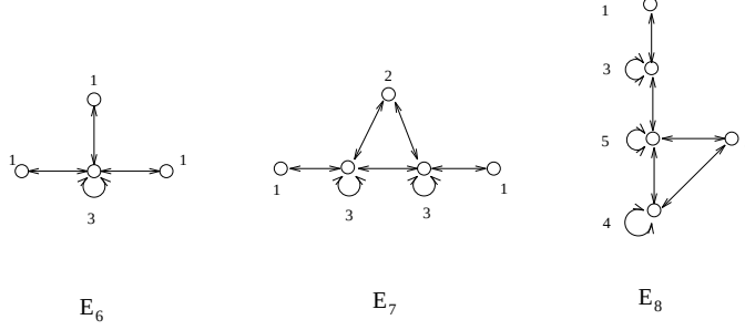
Figure 4: The quiver diagrams for E_6 = A_4 = \Delta(3 \times 2^2) , E_7 = S_4 = \Delta(6 \times 2^2) and E_8 = A_5 = \Sigma_{60} . The theories are finite and non-chiral.
