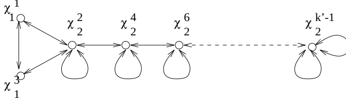
Figure 3: The quiver diagram for d_{k=\text{odd}} . Here again we use the notation of the irreps of D_k to index the nodes. Notice that the theory is again finite and non-chiral.
