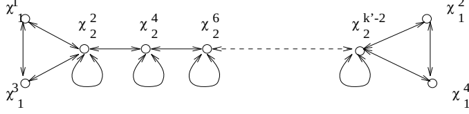
Figure 2: The quiver diagram for d_{k=\text{even}} . Here the notation of the irreps placed on the nodes is borrowed from D_k in §2.1. Notice that it gives a finite theory with non-chiral matter content.
