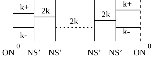
Figure 5: The brane configuration which gives the same matter content as the d_{k=\text{even}} quiver.
