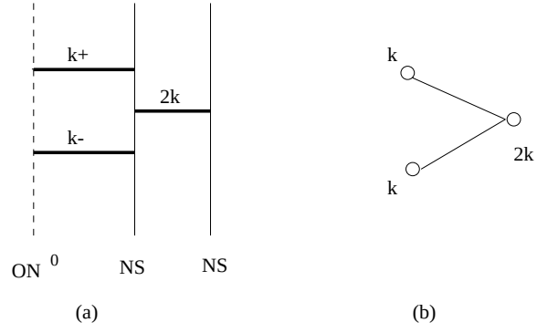
Figure 6: (a). The brane configuration of the projection using NS5-branes. (b). The quiver diagram for the brane configuration in (a).
