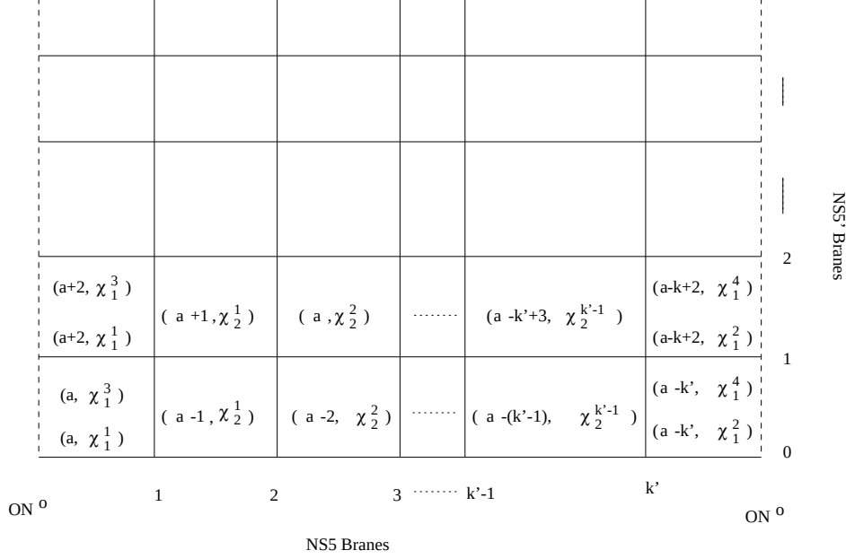
Figure 1: The Brane Box Model for Z_k \times D_{k'} . Notice that for every step along the vertical direction from the bottom to top, the first index has increment 2, while along the horizontal direction from left to right, the first index has decrement 1 and the second index, increment 1. The vertical direction is also periodically identified so that k(\text{ or } \frac{k}{2}) \equiv 0 .
