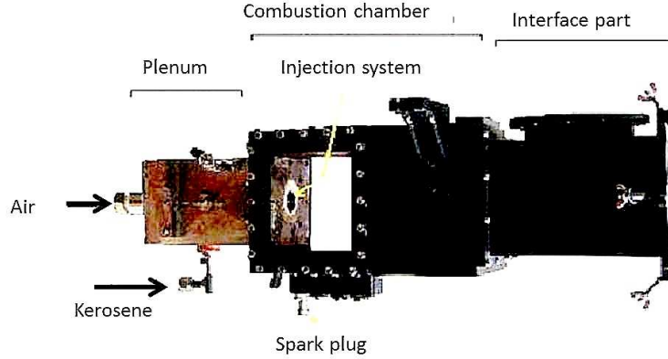
Figure 1: Experimental geometry of the DLR generic combustor [10, 11].
