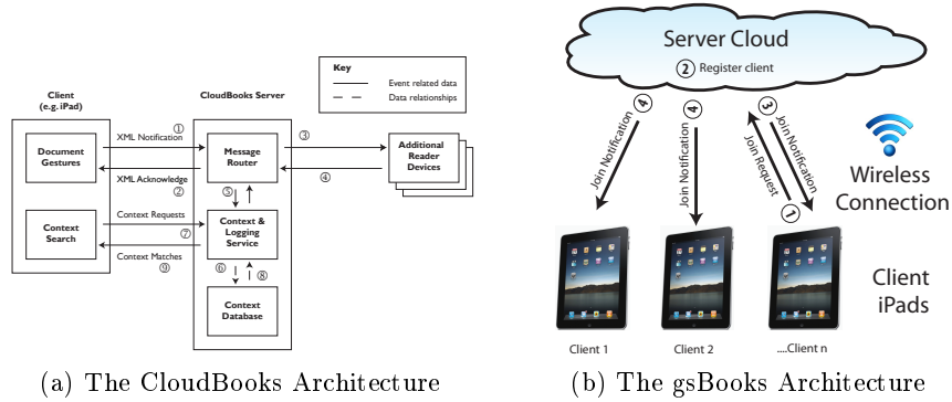
Figure 1: CloudBooks and gsBooks Architectures
