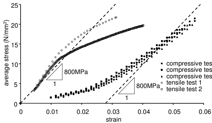
Figure 8 Comparison of tensile and compressive tests on piles made from Sika Biresin G27 mixed 50:50 w/w with aluminium trihydrate (ON) filler.
