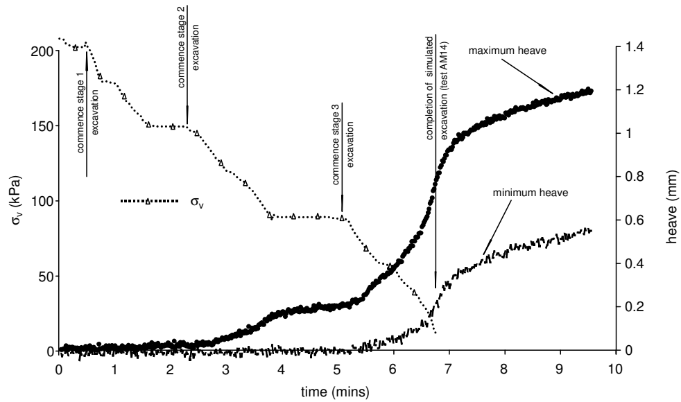
Figure 11 Deformation of excavation formation during the simulated excavation stage of a typical test.
